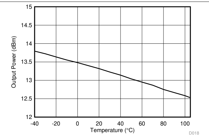
Figure 5-28. TX Maximum Output Power vs Temperature, 915 MHz
