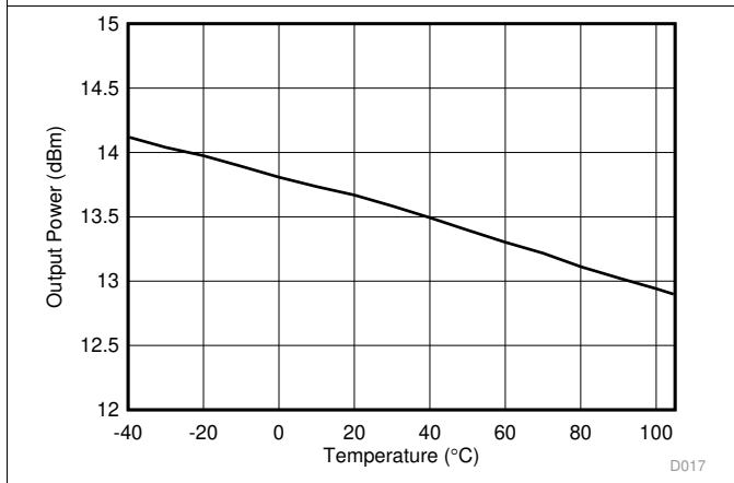
Figure 5-27. TX Maximum Output Power vs Temperature, 868 MHz
