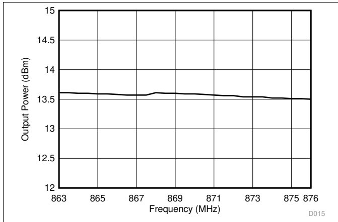
Figure 5-25. TX Maximum Output Power, 863 MHz to 876 MHz
