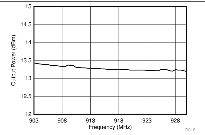
Figure 5-26. TX Maximum Output Power, 902 MHz to 928 MHz
