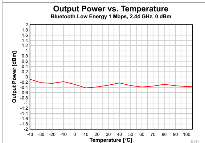
7-37. Output Power vs. Temperature (Bluetooth Low Energy 1 Mbps, 2.44 GHz)
