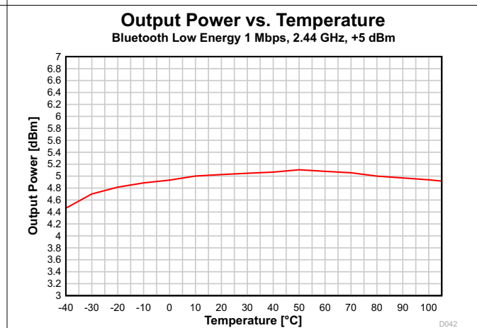
7-38. Output Power vs. Temperature (Bluetooth Low Energy 1 Mbps, 2.44 GHz, +5 dBm)
