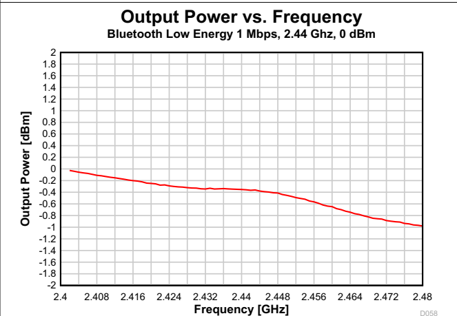
7-50. Output Power vs. Frequency (Bluetooth Low Energy 1 Mbps, 2.44 GHz)
