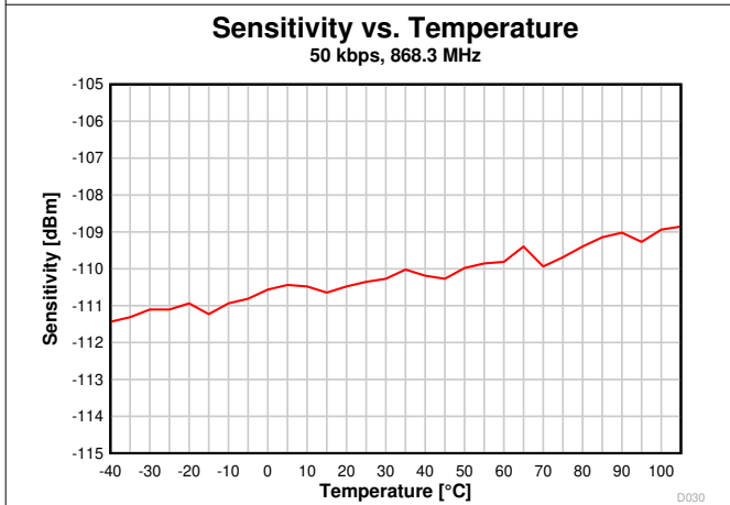
7-24. Sensitivity vs. Temperature (50 kbps, 868.3 MHz)
