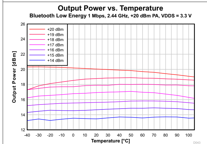
7-39. Output Power vs. Temperature (Bluetooth Low Energy 1 Mbps, 2.44 GHz, +20 dBm PA)
