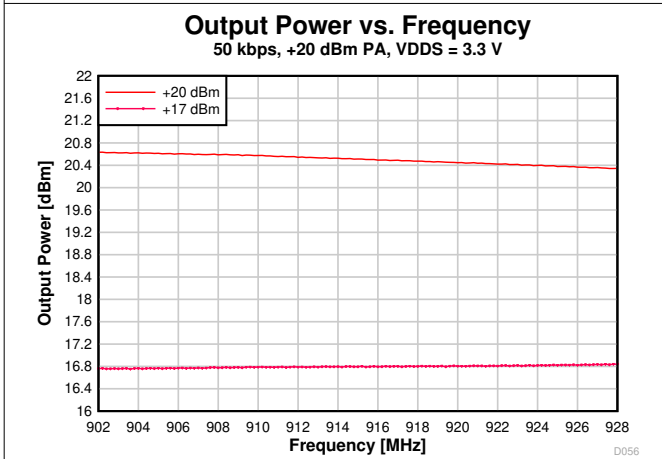
7-49. Output Power vs. Frequency (50 kbps, 915 MHz, VDD3 = 3.3 V)
