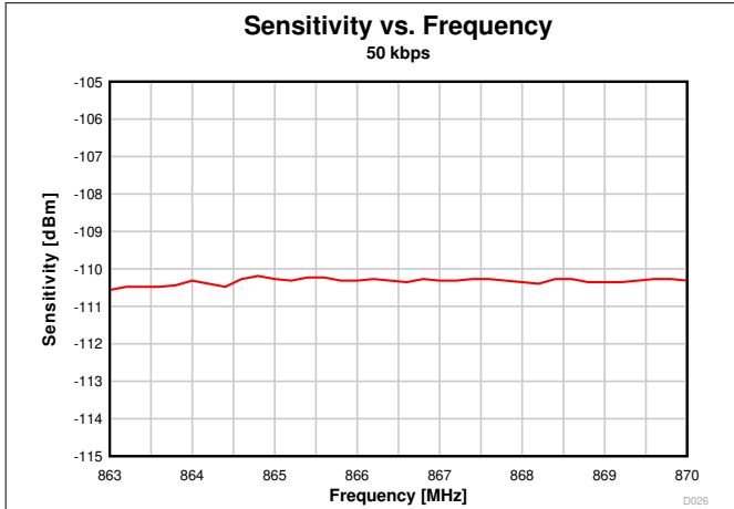
7-20. Sensitivity vs. Frequency (50 kbps, 868 MHz)
