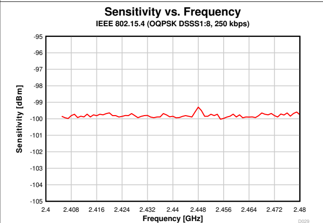
7-23. Sensitivity vs. Frequency (250 kbps, 2.44 GHz)
