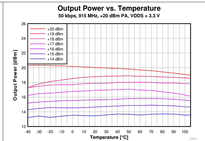
7-36. Output Power vs. Temperature (50 kbps, 915 MHz)
