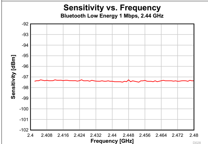
7-22. Sensitivity vs. Frequency (Bluetooth Low Energy 1 Mbps, 2.44 GHz)
