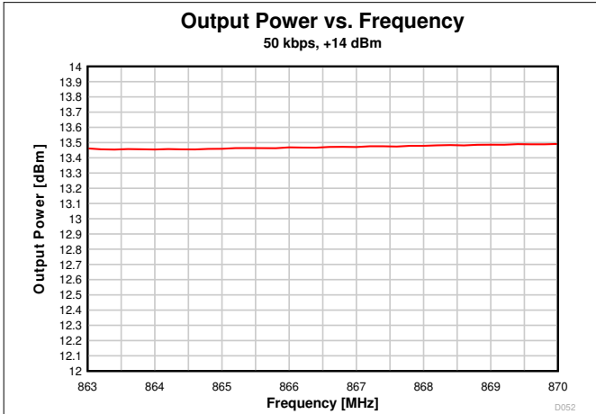
7-47. Output Power vs. Frequency (50 kbps, 868 MHz)
