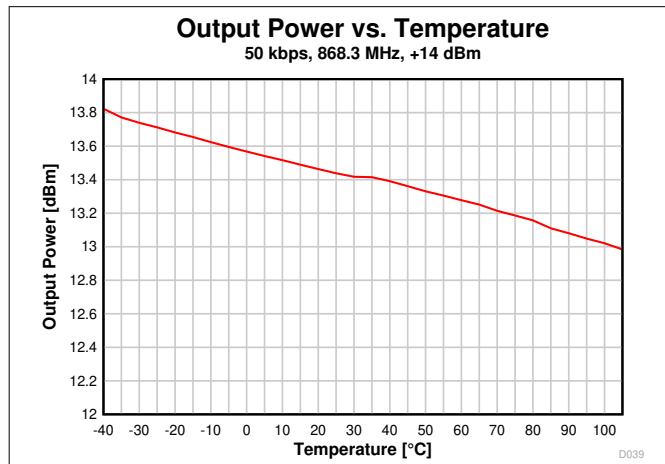
7-35. Output Power vs. Temperature (50 kbps, 868.3 MHz)
