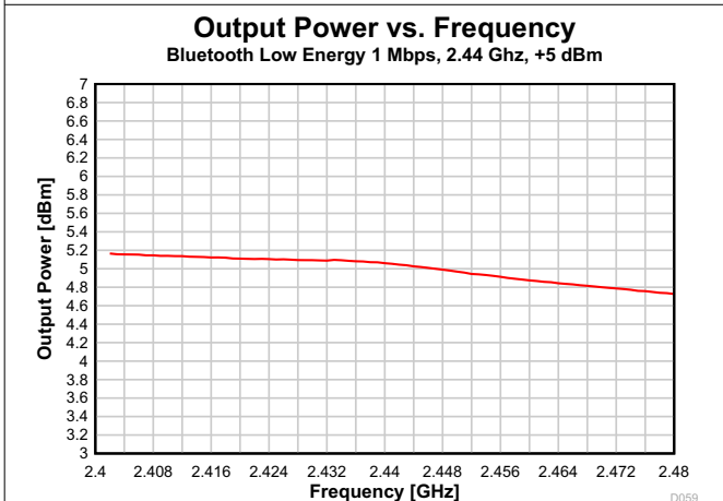
7-51. Output Power vs. Frequency (Bluetooth Low Energy 1 Mbps, 2.44 GHz, +5 dBm)
