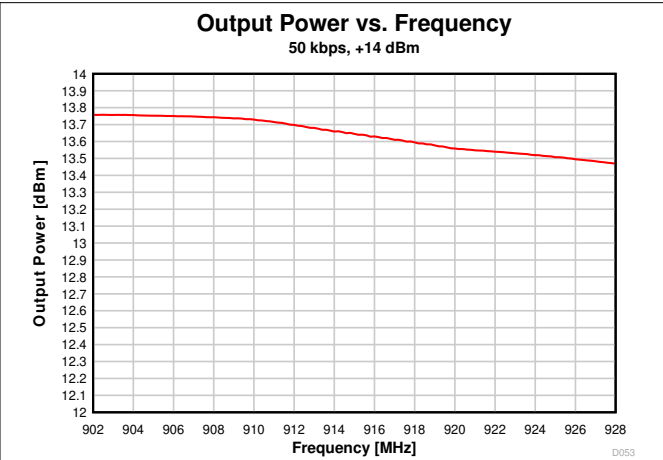
7-48. Output Power vs. Frequency (50 kbps, 915 MHz)
