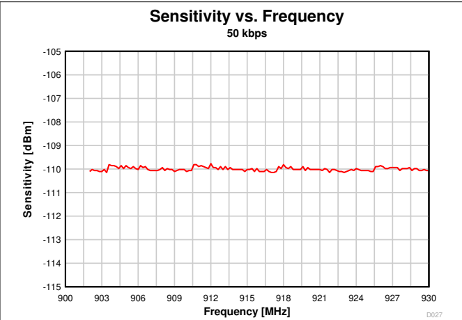
7-21. Sensitivity vs. Frequency (50 kbps, 915 MHz)
