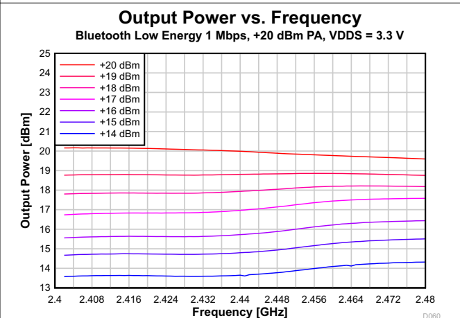
7-52. Output Power vs. Frequency (Bluetooth Low Energy 1 Mbps, 2.44 GHz, +20 dBm PA)
