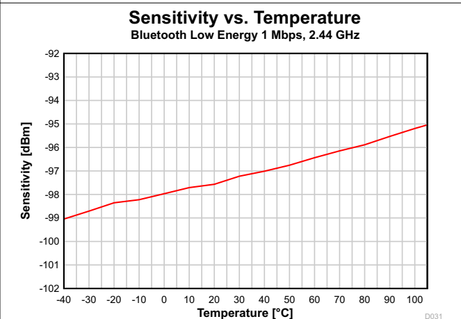
7-25. Sensitivity vs. Temperature (Bluetooth Low Energy 1 Mbps, 2.44 GHz)
