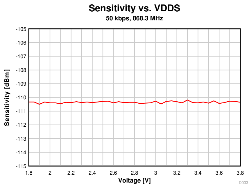
8-24. Sensitivity vs. Supply Voltage (VDDDS) (50 kbps, 868.3 MHz)
