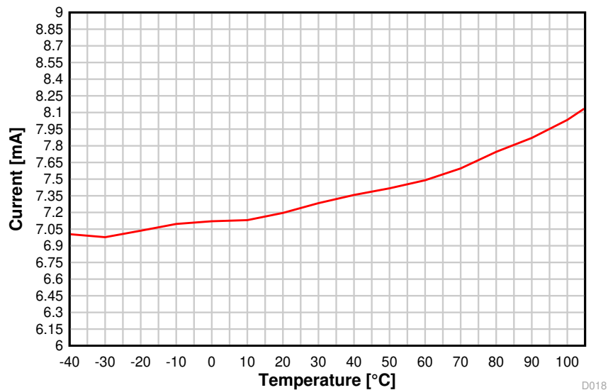
8-14. TX Current vs. Temperature (BLE 1 Mbps, 2.44 GHz)
