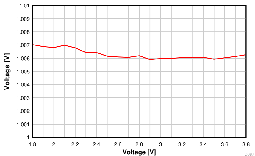
8-48. ADC Accuracy vs. Supply Voltage (VDDS)
