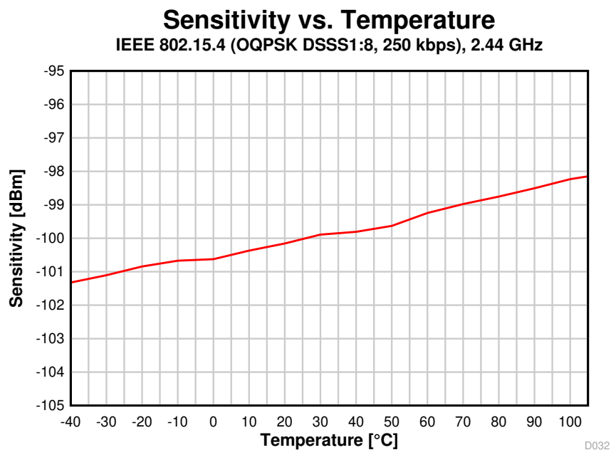
8-23. Sensitivity vs. Temperature (250 kbps, 2.44 GHz)
