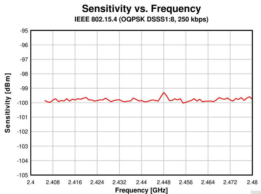
8-20. Sensitivity vs. Frequency (250 kbps, 2.44 GHz)
