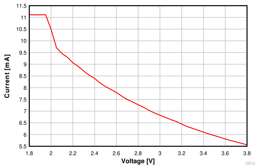
8-10. RX Current vs. Supply Voltage (VDD5) (50 kbps, 868.3 MHz)
