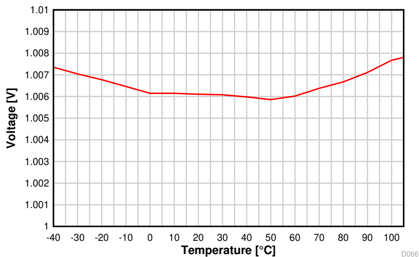
8-47. ADC Accuracy vs. Temperature
