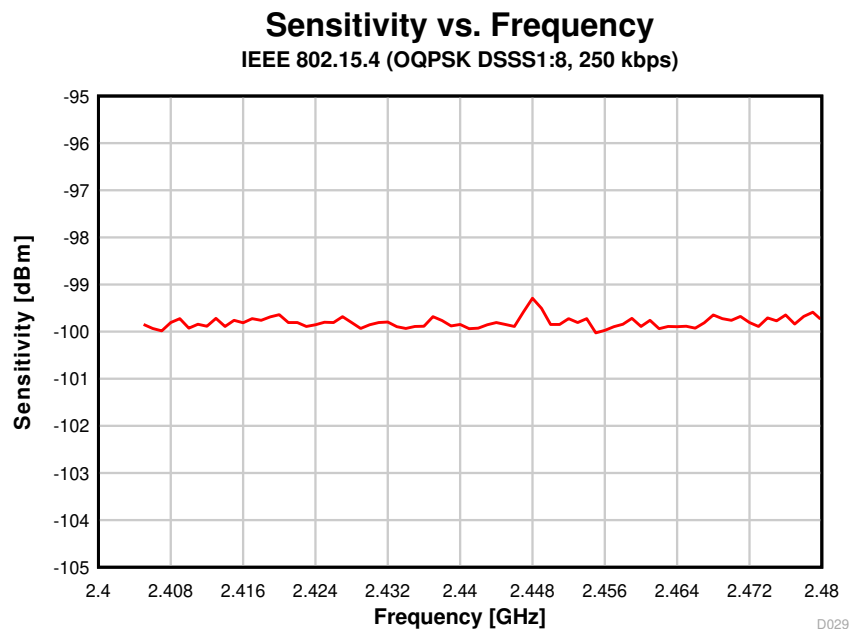
8-20. Sensitivity vs. Frequency (250 kbps, 2.44 GHz)
