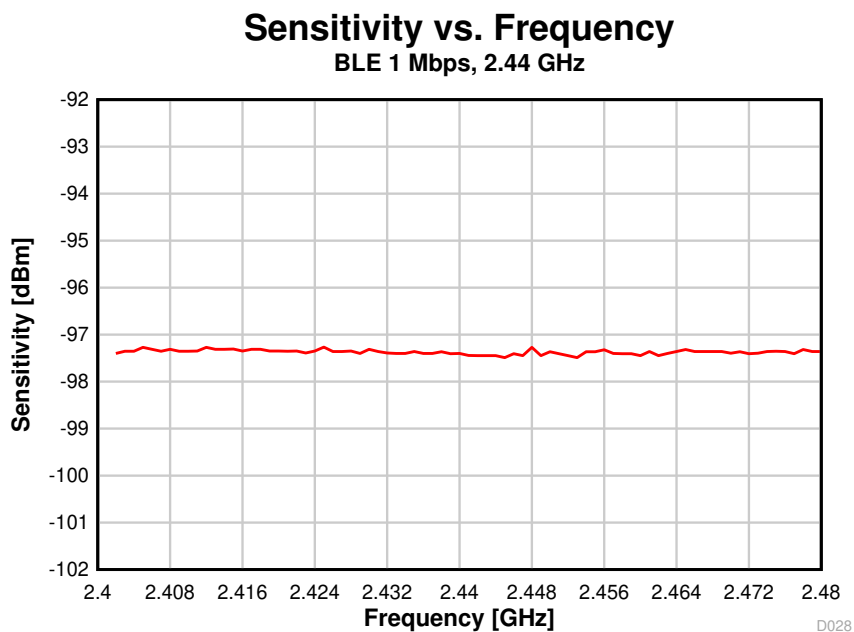
8-19. Sensitivity vs. Frequency (BLE 1 Mbps, 2.44 GHz)
