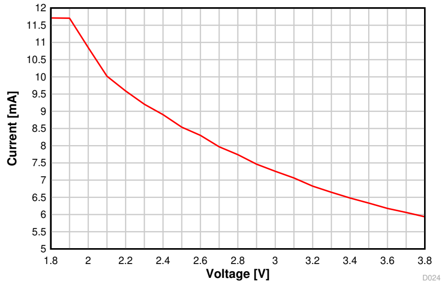
8-16. TX Current vs. Supply Voltage (VDD5) (BLE 1 Mbps, 2.44 GHz)
