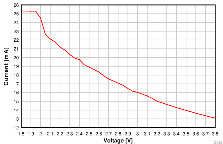
8-15. TX Current vs. Supply Voltage (VDDS) (50 kbps, 868.3 MHz)
