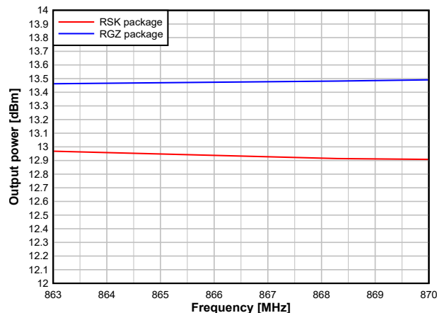
図 7-31. Output Power vs. Frequency (50kbps, 868MHz, +14dBm)
