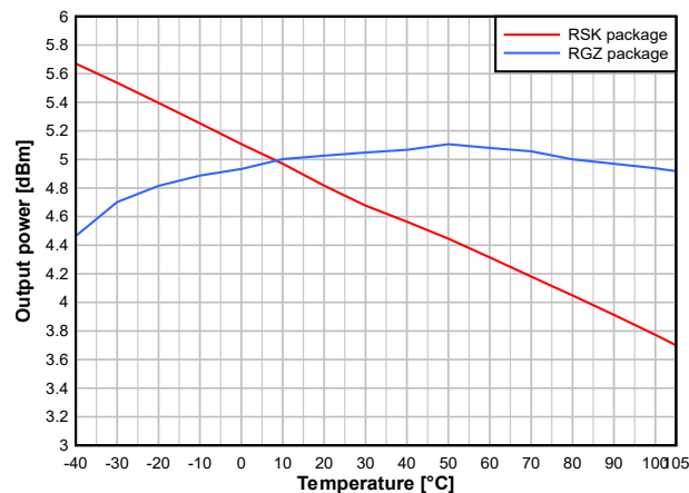
図 7-27. Output Power vs. Temperature (BLE 1Mbps, 2.44GHz, +5dBm)
