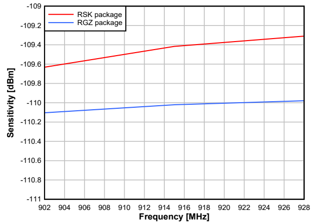
7-15. Sensitivity vs. Frequency (50kbps, 915MHz)
