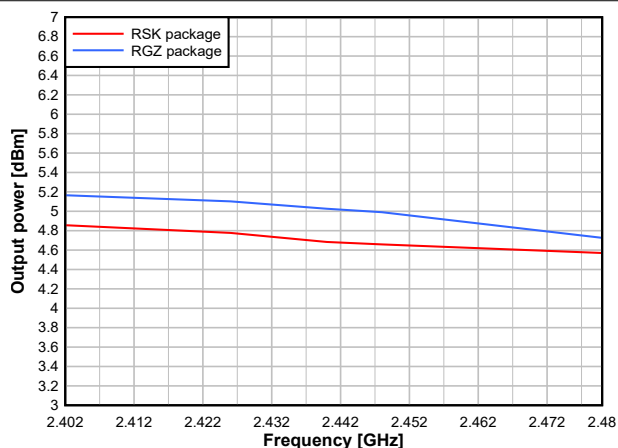
図 7-34. Output Power vs. Frequency (BLE 1Mbps, 2.44GHz, +5dBm)
