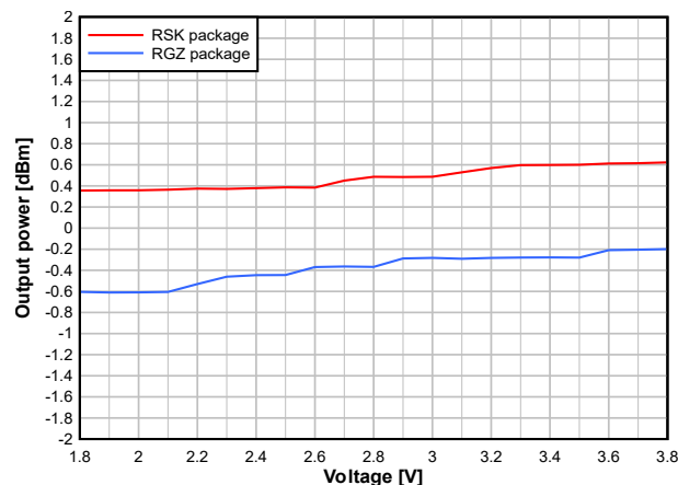
図 7-29. Output Power vs. Supply Voltage (VDD5) (BLE 1Mbps, 2.44GHz, 0dBm)
