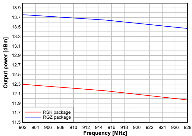
図 7-32. Output Power vs. Frequency (50kbps, 915MHz, +14dBm)
