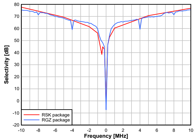
図 7-24. Selectivity vs. Frequency Offset (50kbps, 868.3MHz)
