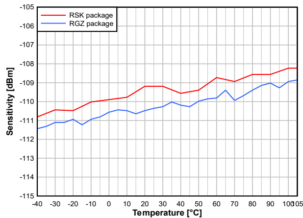
7-18. Sensitivity vs. Temperature (50kbps, 868.3MHz)
