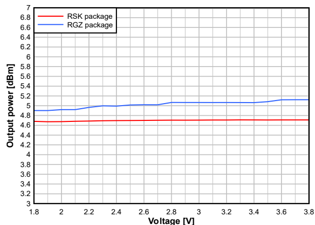
図 7-30. Output Power vs. Supply Voltage (VDD5) (BLE 1Mbps, 2.44GHz, +5dBm)
