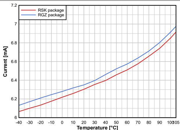
図 7-7. RX Current vs. Temperature (BLE 1Mbps, 2.44GHz)
