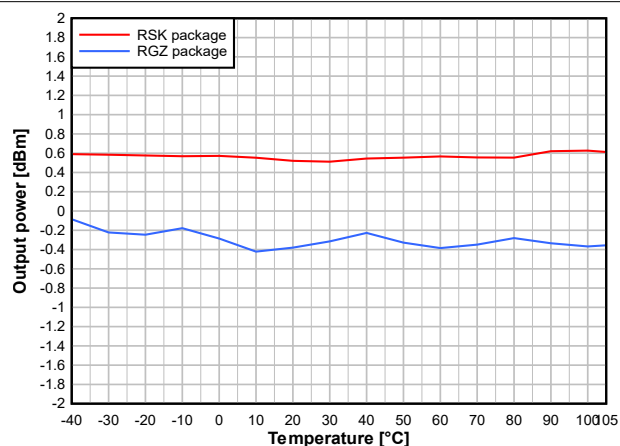
図 7-26. Output Power vs. Temperature (BLE 1Mbps, 2.44GHz, 0dBm)
