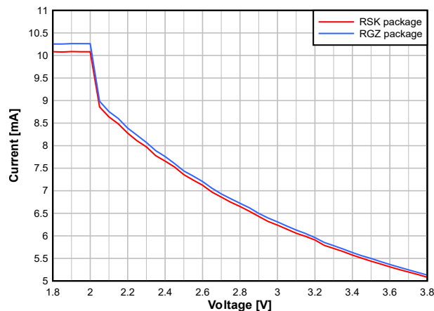
図 7-8. RX Current vs. Supply Voltage (VDD5) (50kbps, 868.3MHz)
