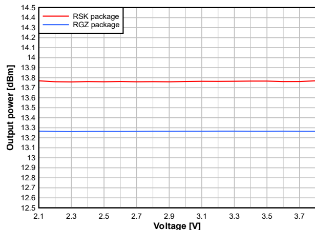
図 7-28. Output Power vs. Supply Voltage (VDD5) (50kbps, 868.3MHz, +14dBm)
