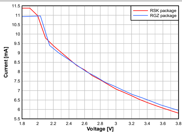
Figure 7-13. TX Current vs. Supply Voltage (VDD) (BLE 1 Mbps, 2.44GHz, 0dBm)
