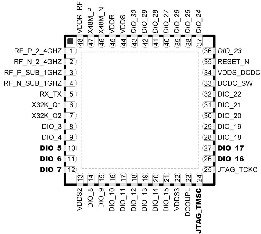
図 6-1. RGZ (7mm × 7mm) Pinout, 0.5mm Pitch (Top View)
