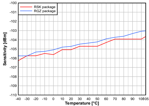
図 7-20. Sensitivity vs. Temperature (250kbps, 2.44GHz)
