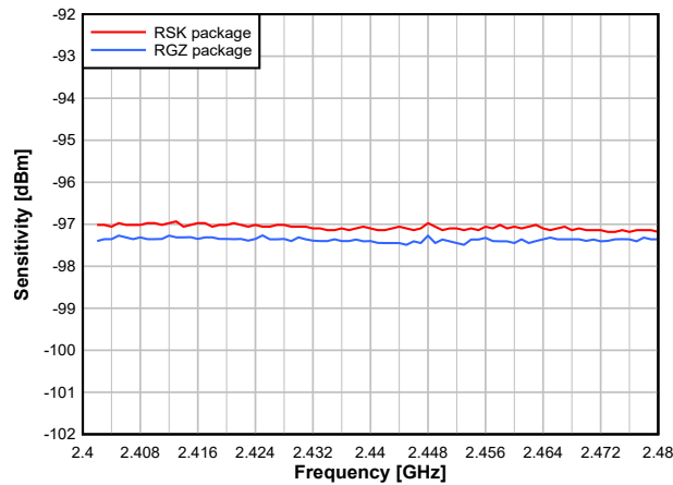
7-16. Sensitivity vs. Frequency (BLE 1Mbps, 2.44GHz)
