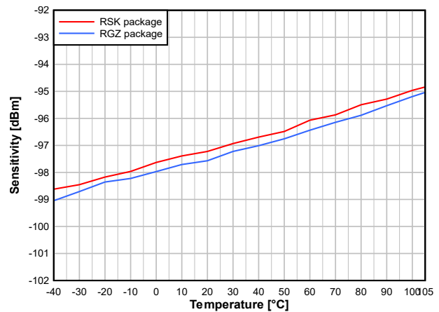
7-19. Sensitivity vs. Temperature (BLE 1 Mbps, 2.44GHz)
