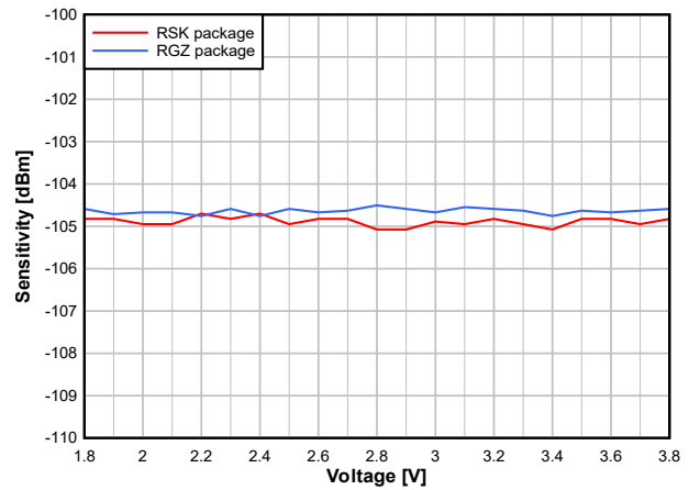
図 7-23. Sensitivity vs. Supply Voltage (VDDS) (250kbps, 2.44GHz)
