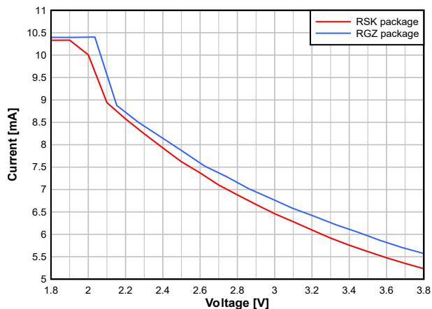
図 7-9. RX Current vs. Supply Voltage (VDD5) (BLE 1Mbps, 2.44GHz)
