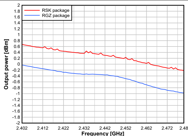
図 7-33. Output Power vs. Frequency (BLE 1Mbps, 2.44GHz, 0dBm)
