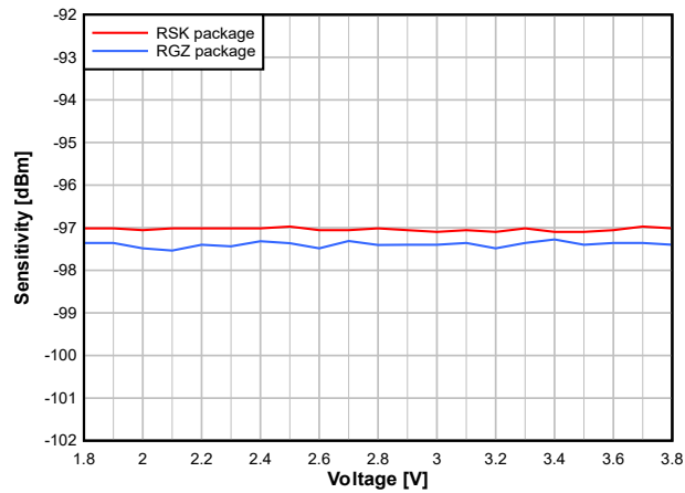
図 7-22. Sensitivity vs. Supply Voltage (VDDS) (BLE 1Mbps, 2.44GHz)
