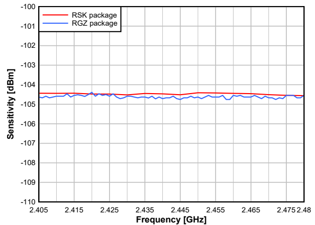
7-17. Sensitivity vs. Frequency (IEEE 802.15.4 OQPSK DSSS1:8, 250kbps, 2.44GHz)
