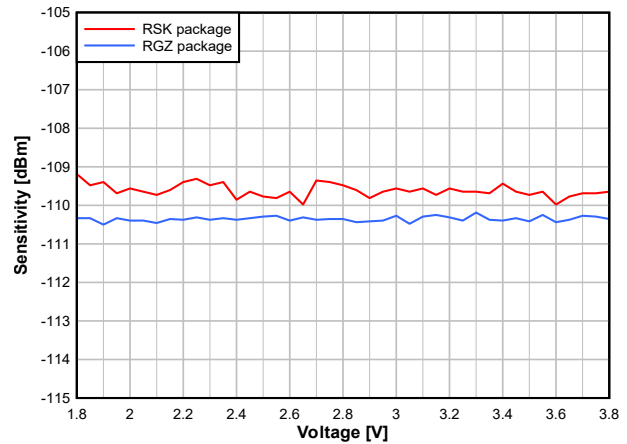
図 7-21. Sensitivity vs. Supply Voltage (VDDS) (50kbps, 868.3MHz)
