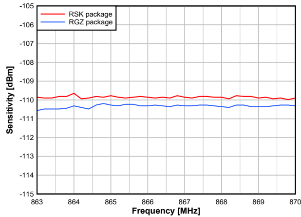
7-14. Sensitivity vs. Frequency (50kbps, 868MHz)
