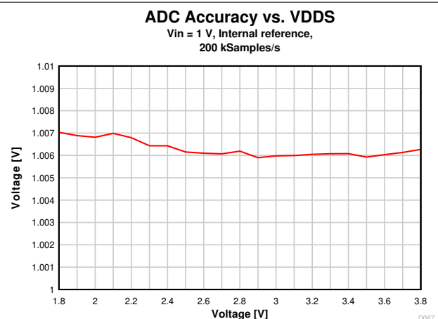
8-38. ADC Accuracy vs. Supply Voltage (VDD5)
