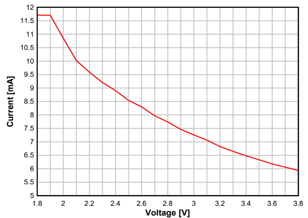
7-11. TX Current vs. Supply Voltage (VDD5) (BLE 1Mbps, 2.44GHz, 0dBm)
