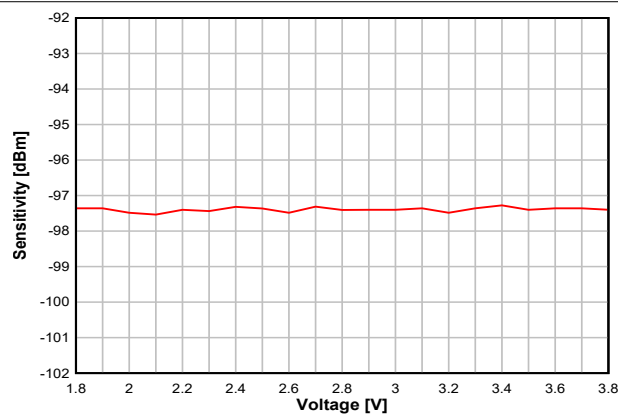
7-18. Sensitivity vs. Supply Voltage (VDD) (BLE 1Mbps, 2.44GHz)
