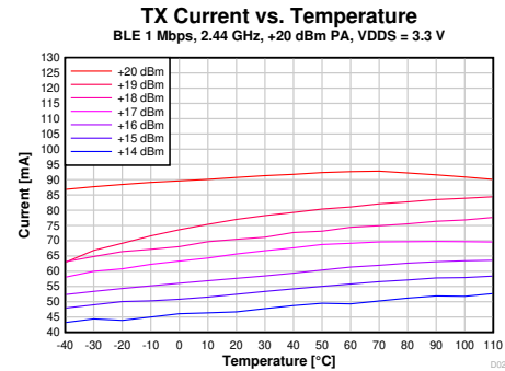
7-9. TX Current vs. Temperature (BLE 1Mbps, 2.44GHz, VDD5 = 3.3V)
