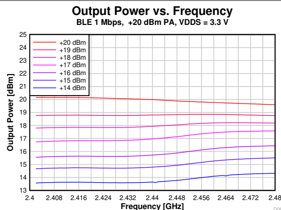
7-31. Output Power vs. Frequency (BLE 1Mbps, 2.44GHz, +20dBm PA)
