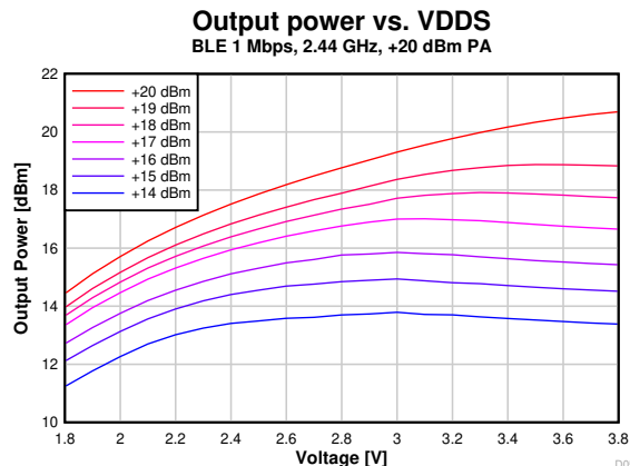
7-27. Output Power vs. Supply Voltage (VDD5) (BLE 1Mbps, 2.44GHz, +20dBm PA)
