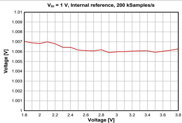
図 7-38. ADC Accuracy vs. Supply Voltage (VDD5)
