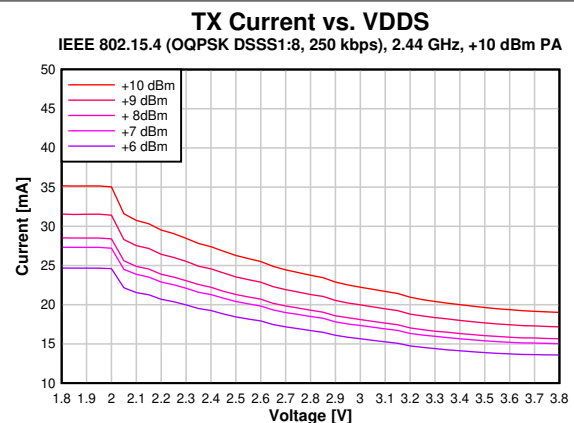
7-13. TX Current vs. Supply Voltage (VDD5) (250kbps, 2.44GHz, +10dBm PA)
