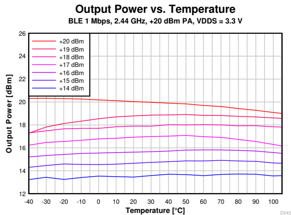
7-23. Output Power vs. Temperature (BLE 1Mbps, 2.44GHz, +20dBm PA)
