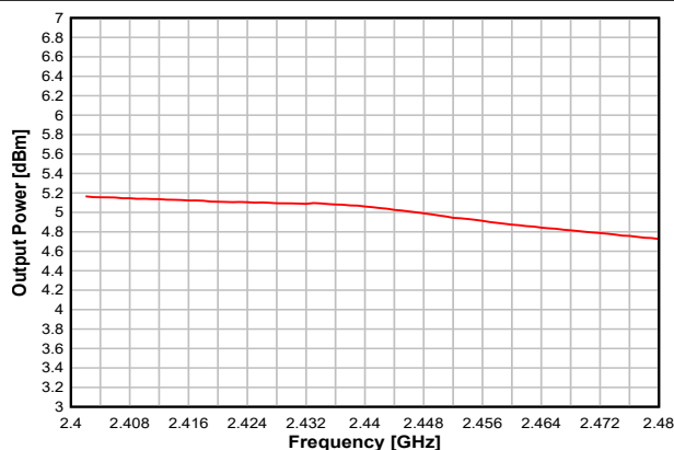
7-30. Output Power vs. Frequency (BLE 1Mbps, 2.44 GHz, +5dBm)
