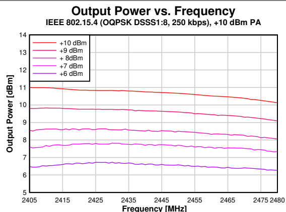
7-32. Output Power vs. Frequency (IEEE 802.15.4-2006, 250 kbps, OQPSK DSSS 1:8, 2.44GHz, +10dBm PA)
