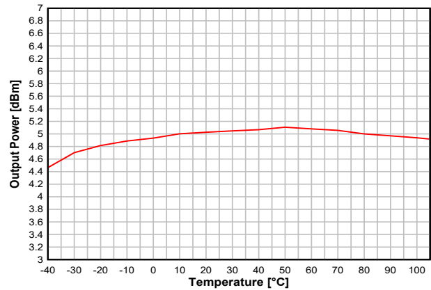
7-22. Output Power vs. Temperature (BLE 1Mbps, 2.44GHz, +5dBm)
