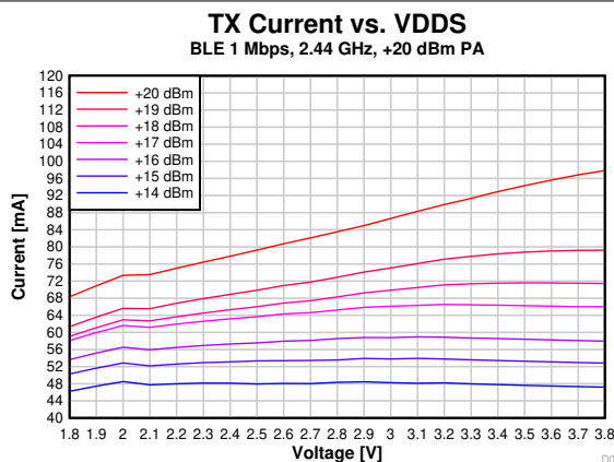
7-12. TX Current vs. Supply Voltage (VDD5) (BLE 1Mbps, 2.44GHz, +20dBm PA)
