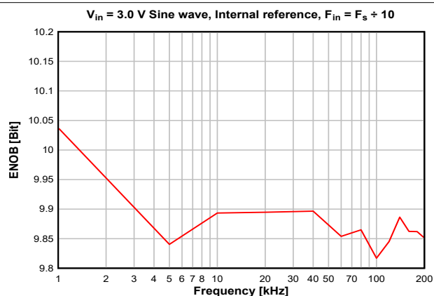
図 7-34. ENOB vs. Sampling Frequency
