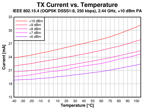
7-10. TX Current vs. Temperature (250kbps, 2.44GHz, +10dBm PA)
