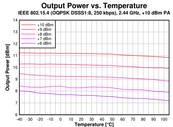
7-24. Output Power vs. Temperature (IEEE 802.15.4-2006, 250 kbps, OQPSK DSSS 1:8, 2.44GHz, +10dBm PA)
