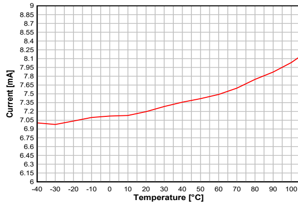
7-8. TX Current vs. Temperature (BLE 1Mbps, 2.44GHz, 0dBm)
