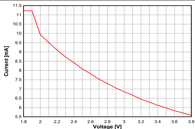
図 7-7. RX Current vs. Supply Voltage (VDDSD) (BLE 1Mbps, 2.44GHz)
