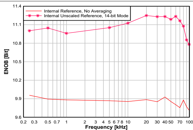
図 7-33. ENOB vs. Input Frequency
