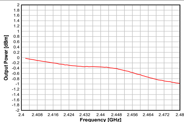
7-29. Output Power vs. Frequency (BLE 1Mbps, 2.44 GHz, 0dBm)
