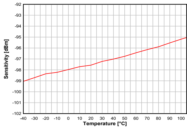
7-16. Sensitivity vs. Temperature (BLE 1Mbps, 2.44GHz)
