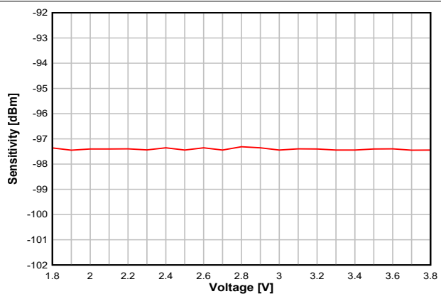
7-19. Sensitivity vs. Supply Voltage (VDD) (BLE 1Mbps, 2.44GHz, DCDC Off)
