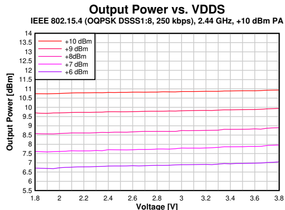
7-28. Output Power vs. Supply Voltage (VDD5) (IEEE 802.15.4-2006, 250 kbps, OQPSK DSSS 1:8, 2.44GHz, +10dBm PA)
