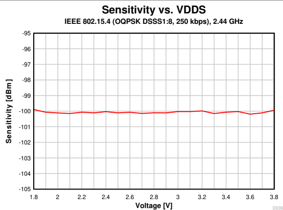
7-20. Sensitivity vs. Supply Voltage (VDDS) (IEEE 802.15.4-2006, 250 kbps, OQPSK DSSS 1:8, 2.44GHz)
