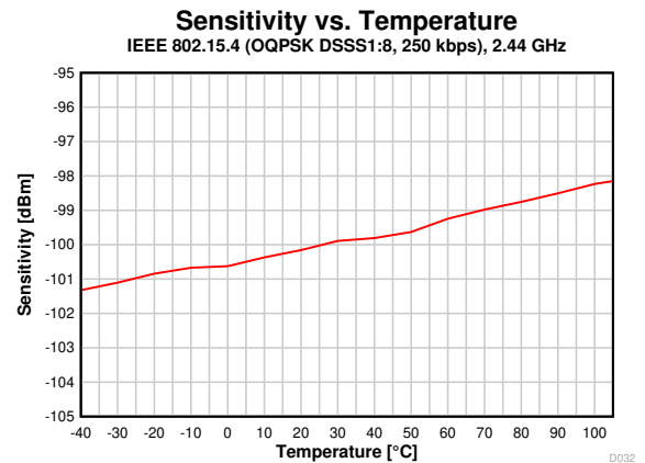
7-17. Sensitivity vs. Temperature (IEEE 802.15.4-2006, 250 kbps, OQPSK DSSS 1:8, 2.44GHz)
