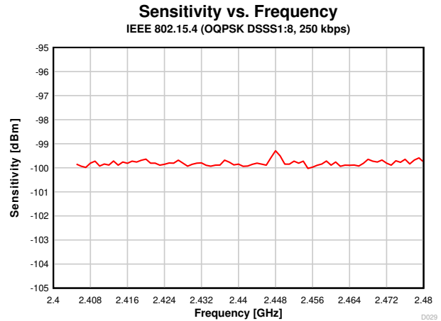
7-15. Sensitivity vs. Frequency (IEEE 802.15.4-2006, 250 kbps, OQPSK DSSS 1:8, 2.44GHz)
