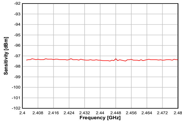
7-14. Sensitivity vs. Frequency (BLE 1Mbps, 2.44GHz)
