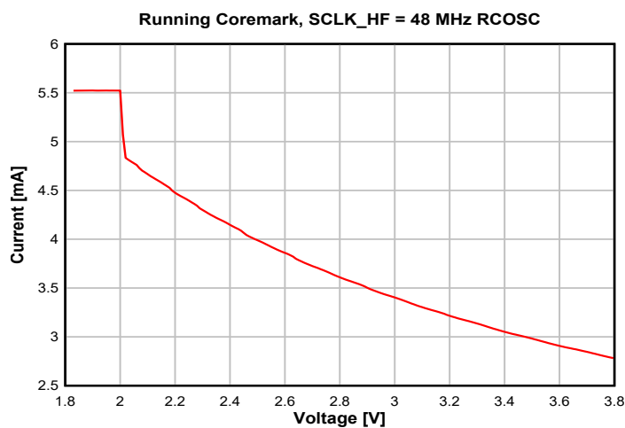
図 7-4. Active Mode (MCU) Current vs. Supply Voltage (VDD5)
