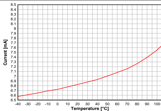
図 7-6. RX Current vs. Temperature (BLE 1Mbps, 2.44GHz)
