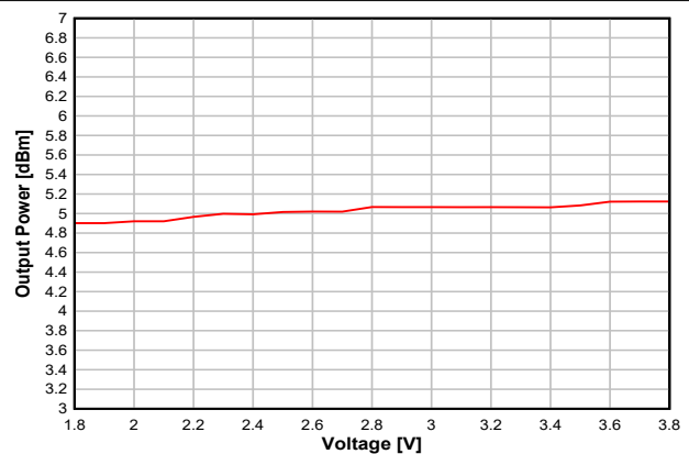
7-26. Output Power vs. Supply Voltage (VDD5) (BLE 1 Mbps, 2.44GHz, +5dBm)
