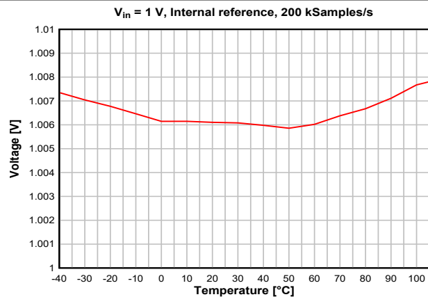
図 7-37. ADC Accuracy vs. Temperature
