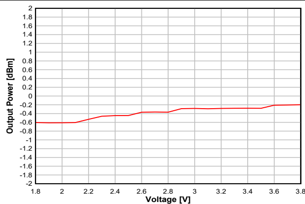
7-25. Output Power vs. Supply Voltage (VDD5) (BLE 1 Mbps, 2.44GHz, 0dBm)
