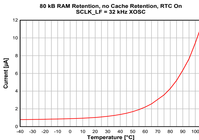
図 7-5. Standby Mode (MCU) Current vs. Temperature
