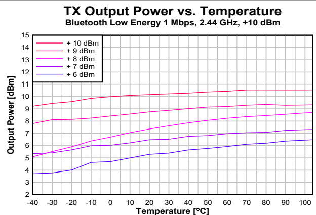
FIG 7-24. Output Power vs. Temperature (2.44 GHz, +10 dBm PA)
