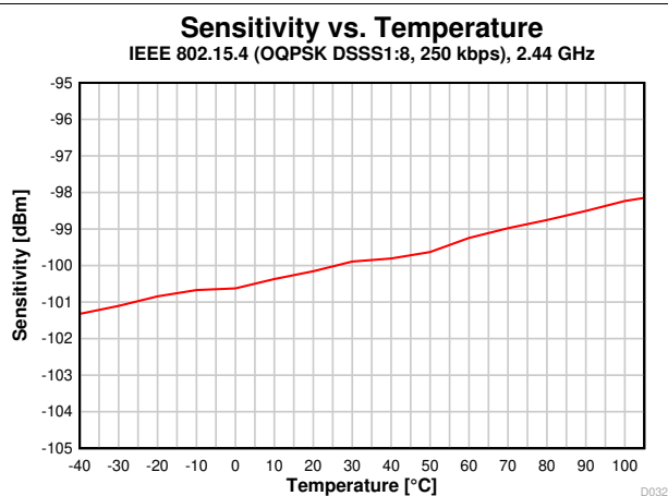
7-17. Sensitivity vs. Temperature (250 kbps, 2.44 GHz)
