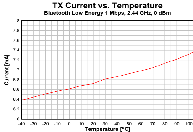
图 7-8. TX Current vs. Temperature (Bluetooth Low Energy 1 Mbps, 2.44 GHz)
