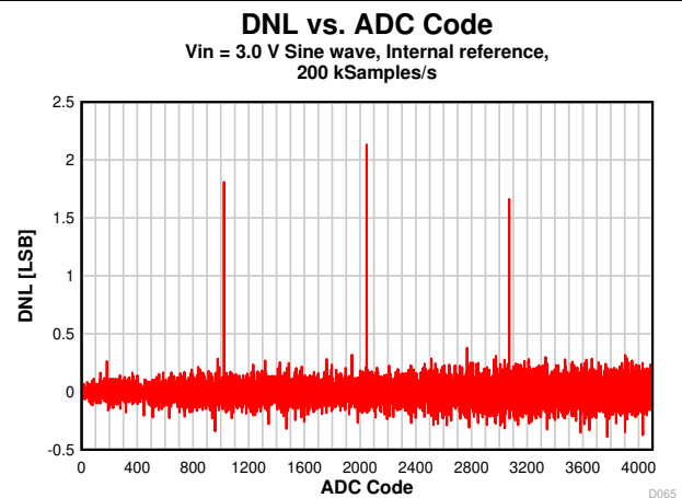
7-36. DNL vs. ADC Code
