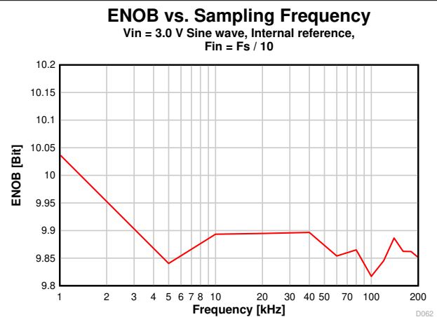
7-34. ENOB vs. Sampling Frequency
