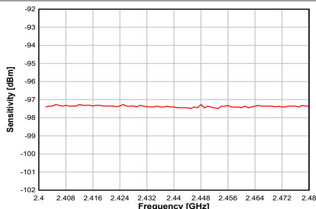
図 8-10. Sensitivity vs. Frequency (BLE 1 Mbps, 2.44 GHz)
