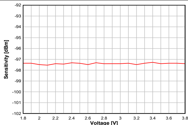
図 8-14. Sensitivity vs. Supply Voltage (VDD) (BLE 1 Mbps, 2.44 GHz)
