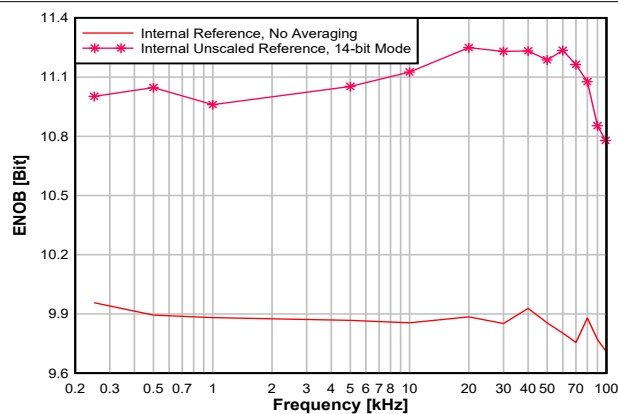
8-23. ENOB vs. Input Frequency
