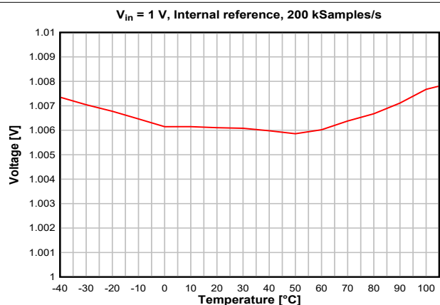
8-27. ADC Accuracy vs. Temperature
