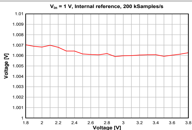
8-28. ADC Accuracy vs. Supply Voltage (VDD5)
