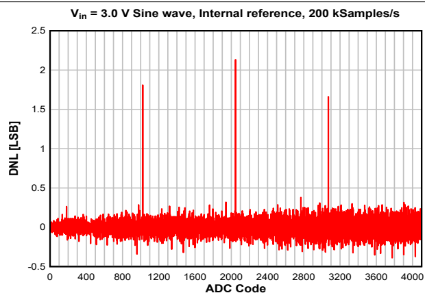
8-26. DNL vs. ADC Code
