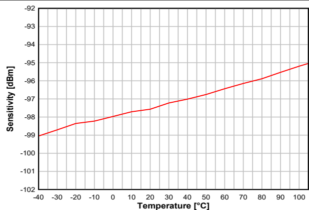
図 8-12. Sensitivity vs. Temperature (BLE 1 Mbps, 2.44 GHz)
