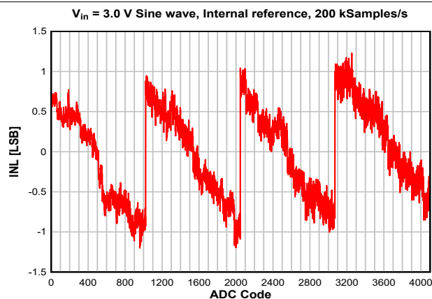
8-25. INL vs. ADC Code
