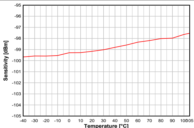
図 8-13. Sensitivity vs. Temperature (IEEE 802.15.4-2006, 250 kbps, OQPSK DSSS 1:8, 2.44 GHz)
