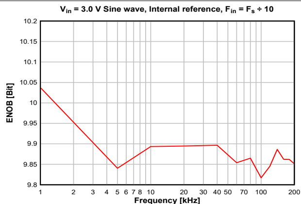
8-24. ENOB vs. Sampling Frequency
