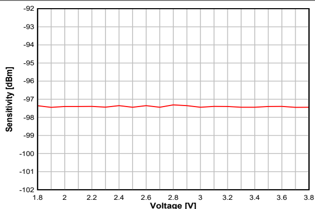
図 8-15. Sensitivity vs. Supply Voltage (VDD) (BLE 1 Mbps, 2.44 GHz, DCDC Off)
