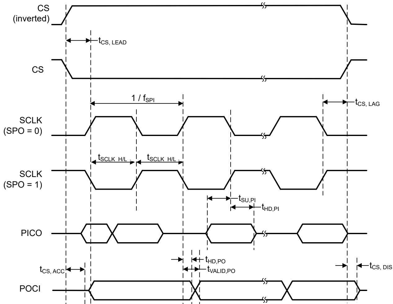
Peripheral Mode, SPH = 1
