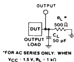
図 5-3. Propagation Delays Times and Test Circuit.
