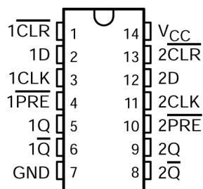
図 3-1. D, N, or J Package 14-Pin SOIC, PDIP, or CDIP (Top View)
