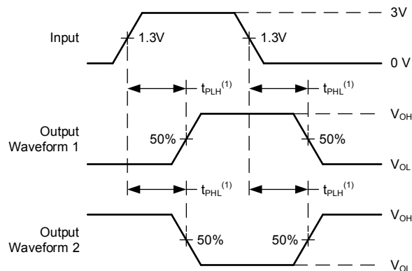
6-5. Voltage Waveforms, Propagation Delays for TTL-Compatible Inputs
