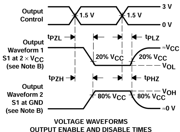
6-1. Load Circuit and Voltage Waveforms
