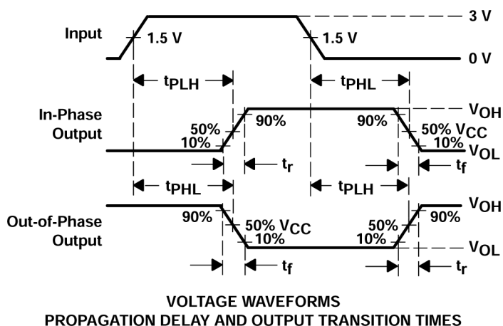
6-1. Load Circuit and Voltage Waveforms
