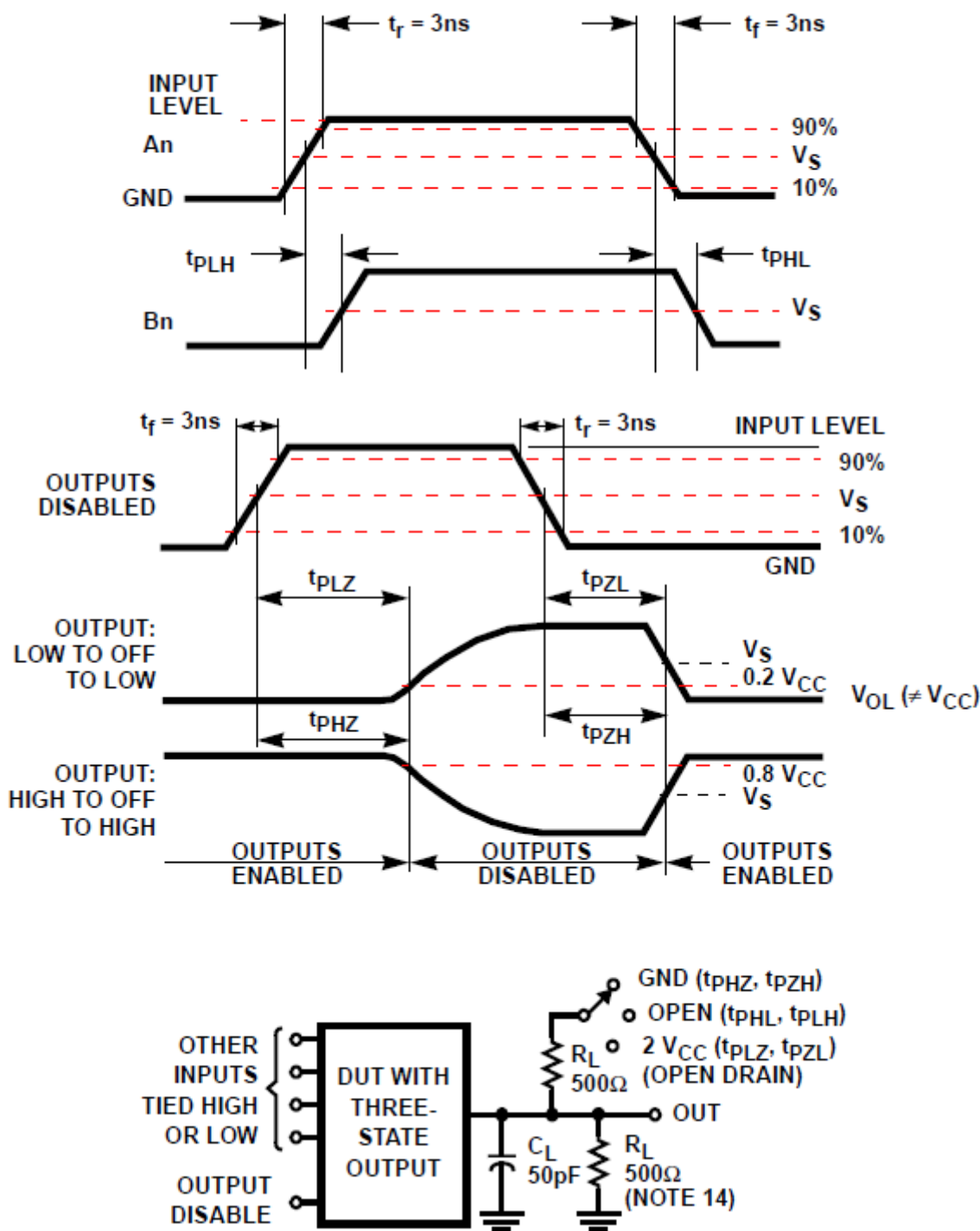
図 4-1. THREE-STATE PROPAGATION DELAY TIMES AND TEST CIRCUIT
