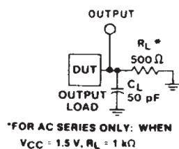
図 5-3. Propagation Delays Times and Test Circuit.
