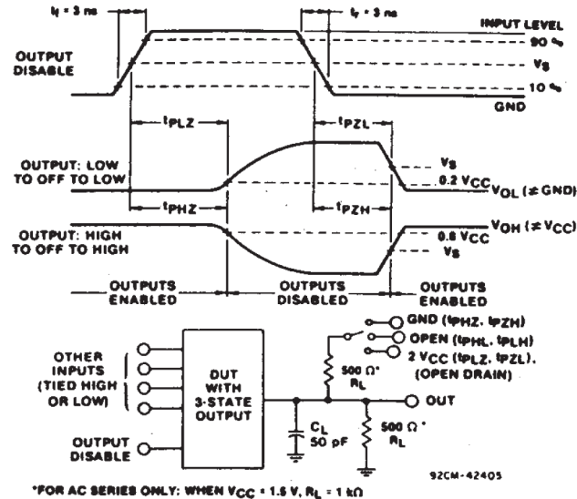
図 5-2. Three-state Propagation Delay Waveforms and Test Circuit.
