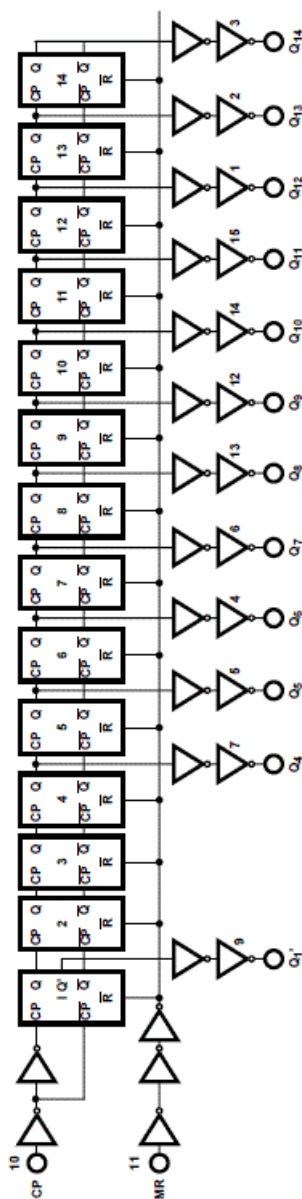
7-1. Functional Diagram
