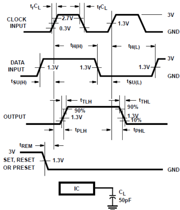
FIG 6-6. HCT setup times, hold times, removal time, and propagation delay times for edge triggered sequential logic circuits
