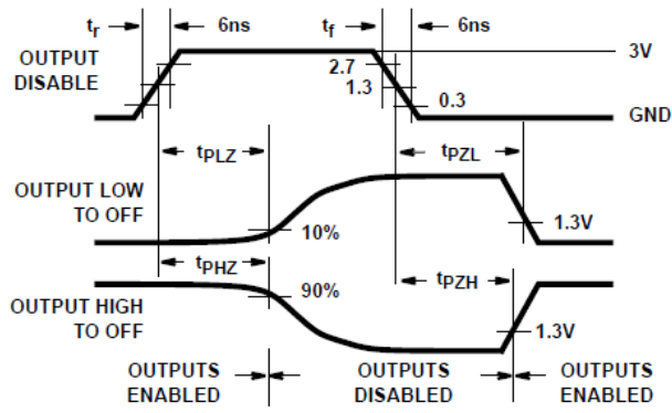
FIG 6-8. HCT three-state propagation delay waveform
