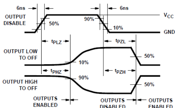
FIG 6-7. HC three-state propagation delay waveform
