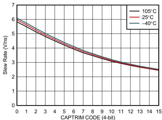
Figure 9-2. Output Slew Rate vs. CAPTRIM Code
