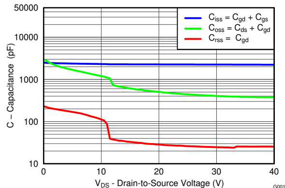
4-5. Capacitance
