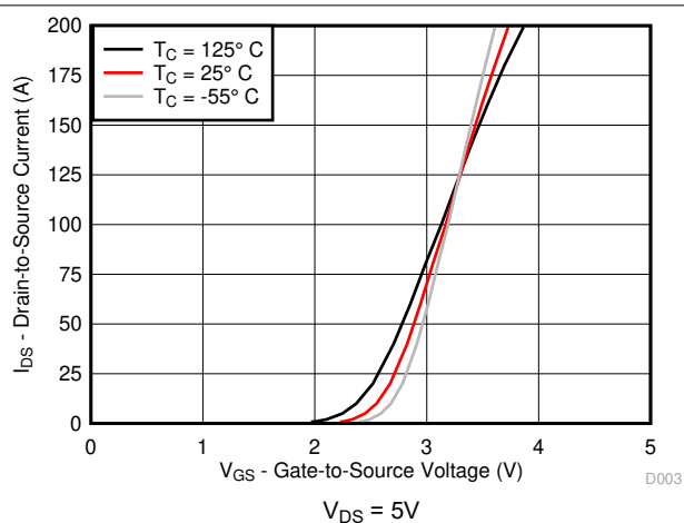
図 4-3. Transfer Characteristics
