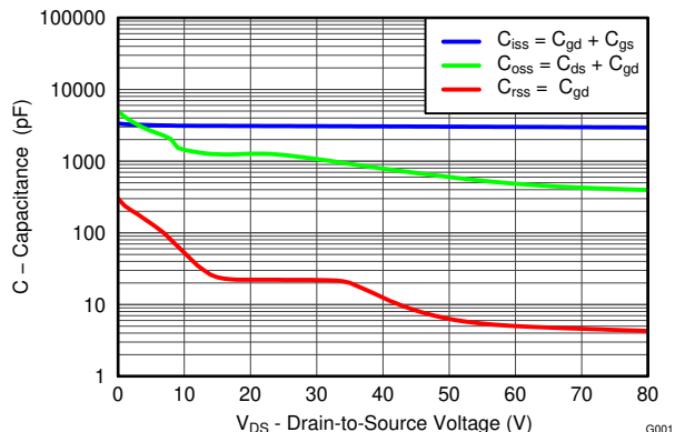
4-5. Capacitance
