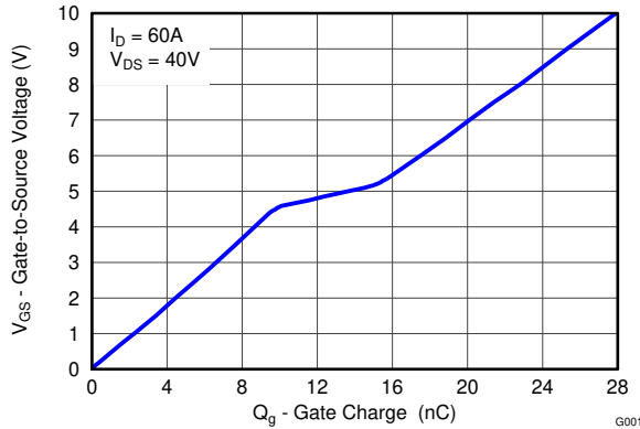
4-4. Gate Charge
