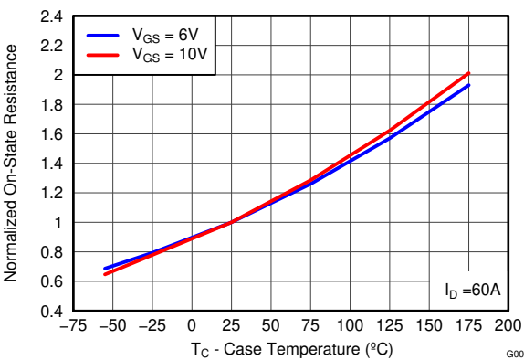
図 4-8. Normalized On-State Resistance vs Temperature
