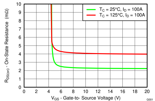
FIG 4-7. On-State Resistance vs Gate-to-Source Voltage
