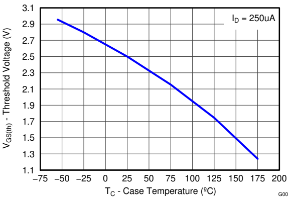
FIG 4-6. Threshold Voltage vs Temperature
