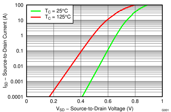
FIG 4-9. Typical Diode Forward Voltage
