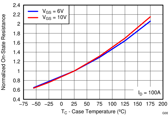
FIG 4-8. Normalized On-State Resistance vs Temperature
