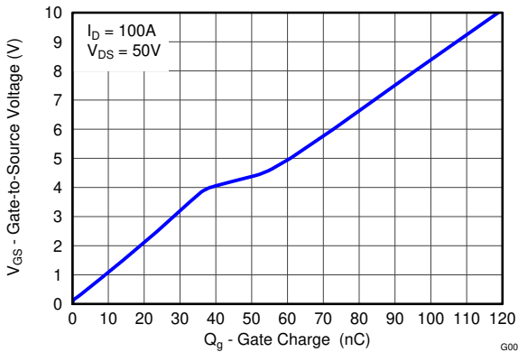
FIG 4-4. Gate Charge
