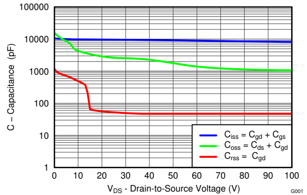
FIG 4-5. Capacitance
