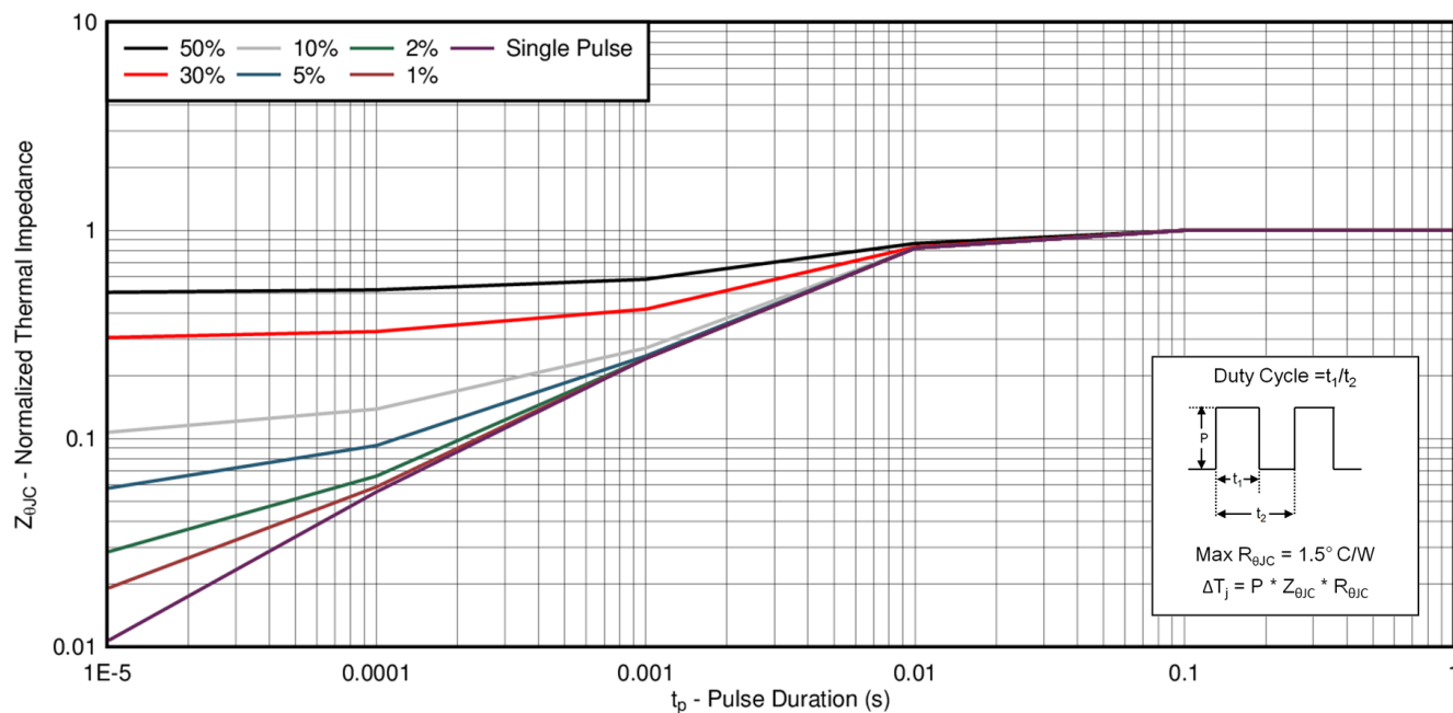
FIG 5-1. Transient Thermal Impedance
