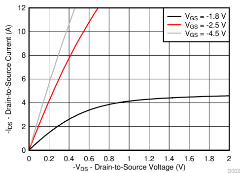
4-2. Saturation Characteristics
