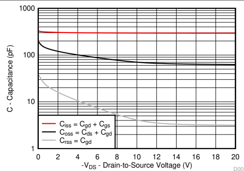
4-5. Capacitance
