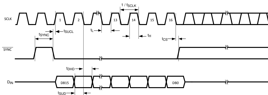
5-1. Timing Diagram
