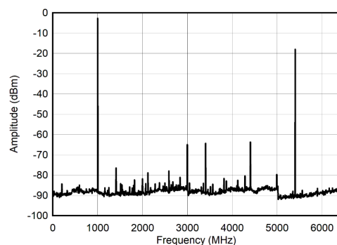
✎ 6-42. Single Channel NRZ Mode: Single Tone Spectrum at 1 GHz
