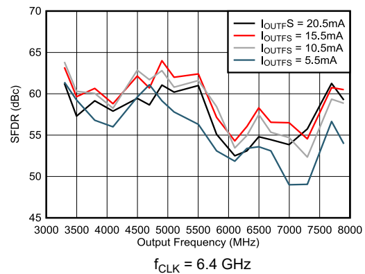
FIG 6-90. Dual Channel 2xRF Mode: SFDR vs Output Frequency and Output Current
