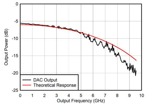
FIG 6-8. Single Channel RTZ Mode: Output Power vs Output Frequency
