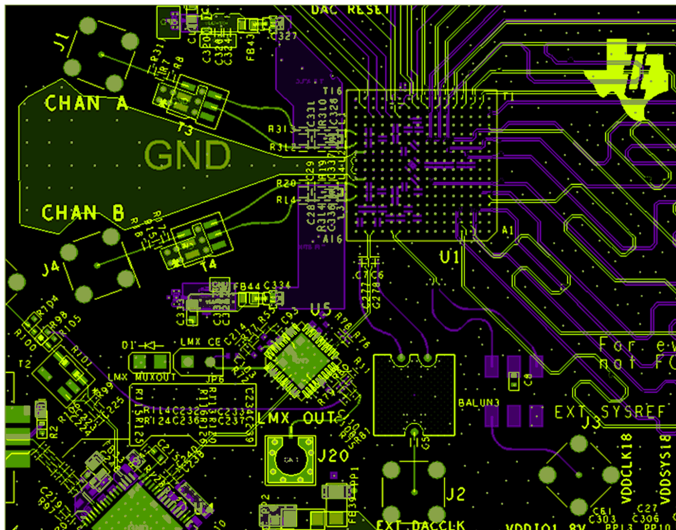
8-5. Top (green traces) and Bottom (purple traces) Routing of DAC CLK and SYSREF
