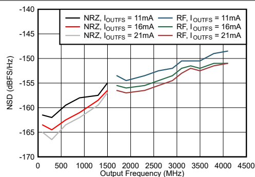
Figure 6-68. Dual Channel NRZ and RF Mode: NSD vs Output Frequency and Output Current
