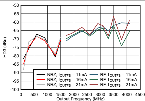
Figure 6-67. Dual Channel NRZ and RF Mode: HD3 vs Output Frequency and Output Current
