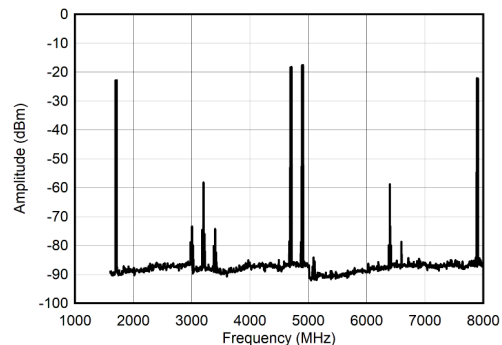
✎ 6-38. Dual Channel 2xRF Mode: Dual Tone Spectrum at 3.8 to 5.8 GHz \pm 10 MHz
