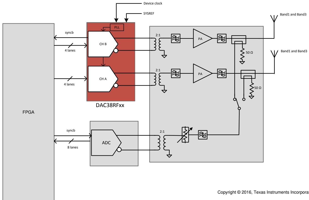
図 8-2. Two Antennae Multi-band Radio Frequency Transmitter
