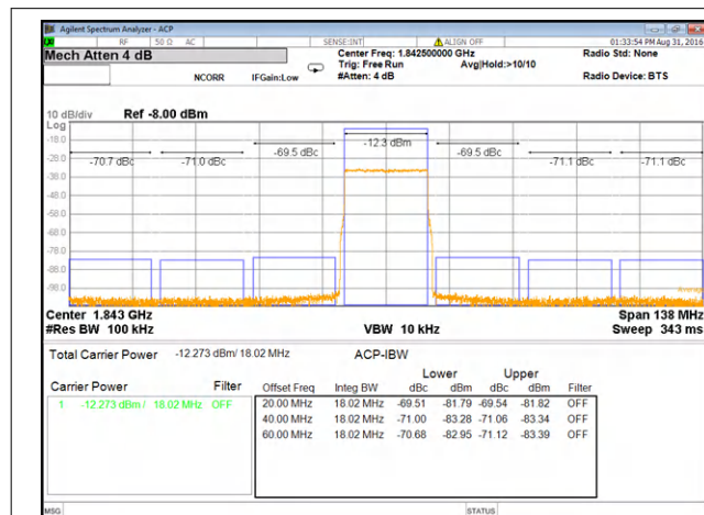
図 8-4. Dual band ACPR Performance in Downlink Band 3 with On-chip PLL
