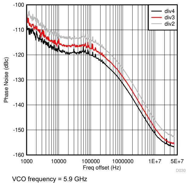
6-44. VCO0 Output clock Phase Noise vs Offset Frequency Over Divider Ratio
