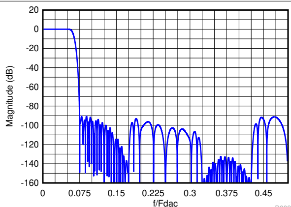
図 7-15. Composite Magnitude Response for 8x Interpolation
