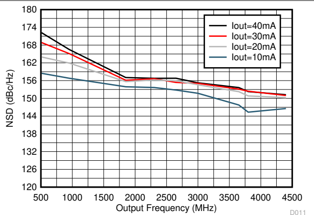
Measured 50 MHz from carrier DAC38RF83/93/85
