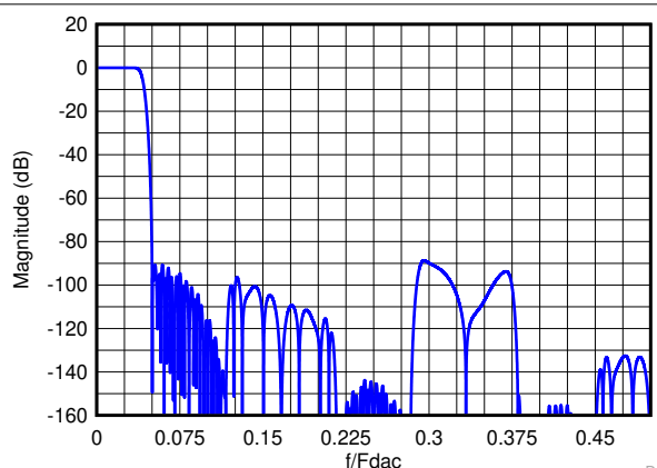
図 7-17. Composite Magnitude Response for 12x Interpolation
