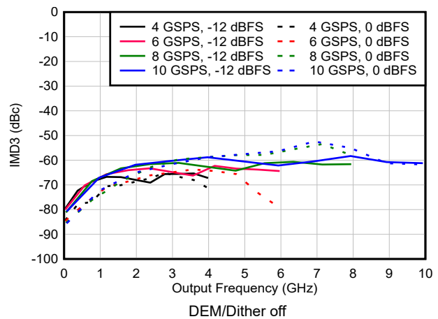
图 6-130. IMD3 vs Frequency and Sample Rate in NRZ/RF Modes
