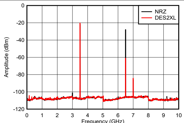
6-28. f_{\text{OUT}} = 3497\text{ MHz} , 0 dBFS
