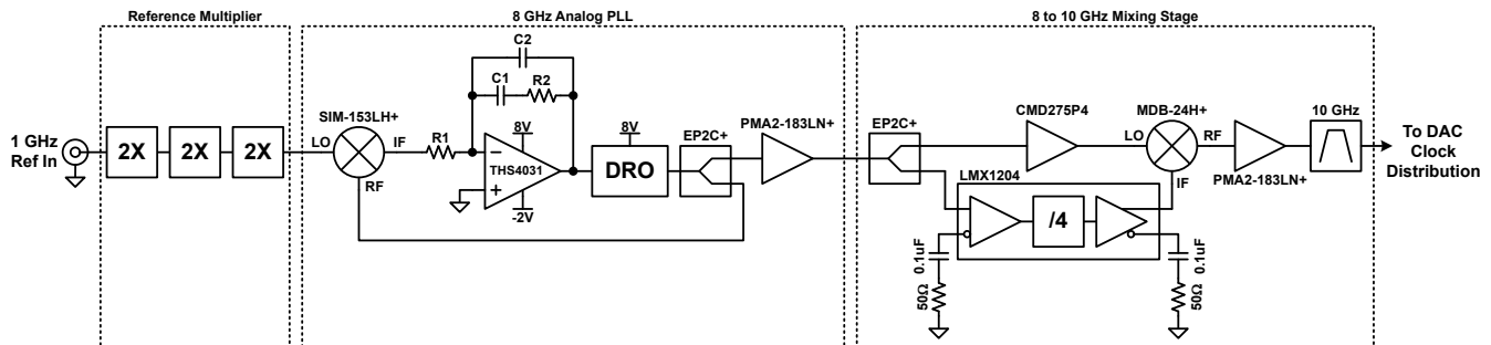
8-12. 10 GHz Clock Synthesizer
