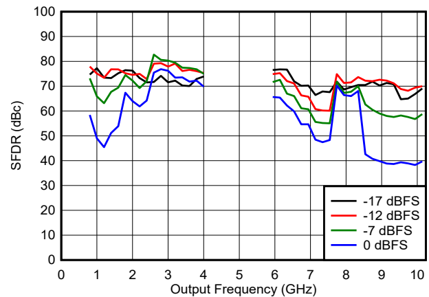
FIG 6-106. SFDR vs Frequency and Digital Amplitude in DES2X Modes
