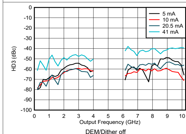
図 6-157. HD3 vs Frequency and Output Current in NRZ/RF Modes
