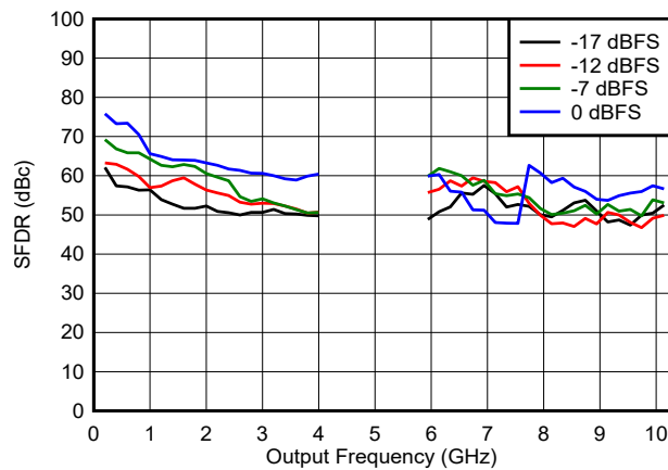
FIG 6-105. SFDR vs Frequency and Digital Amplitude in DES2X Modes
