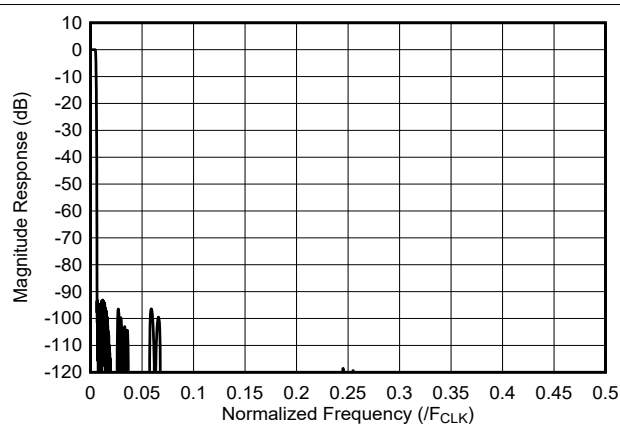
7-36. 96x Interpolation Filter Response
