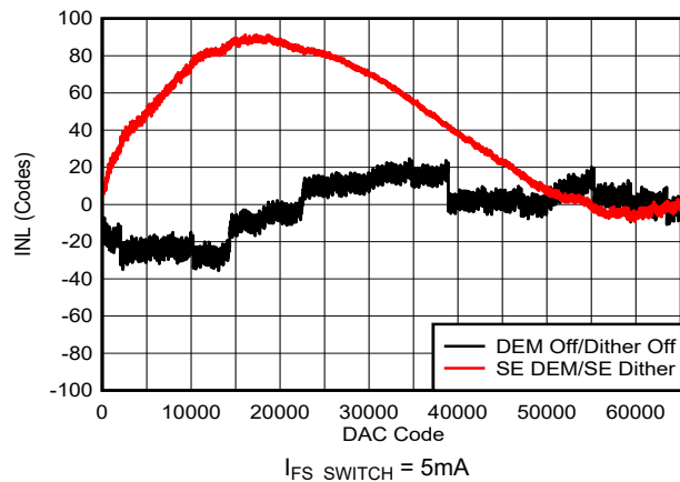
图 6-14. INL vs DAC Code: 5mA
