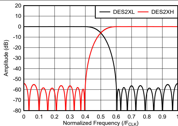
図 7-48. DES Interpolator Frequency Response
