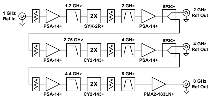
8-10. Reference Multiplier Chain
