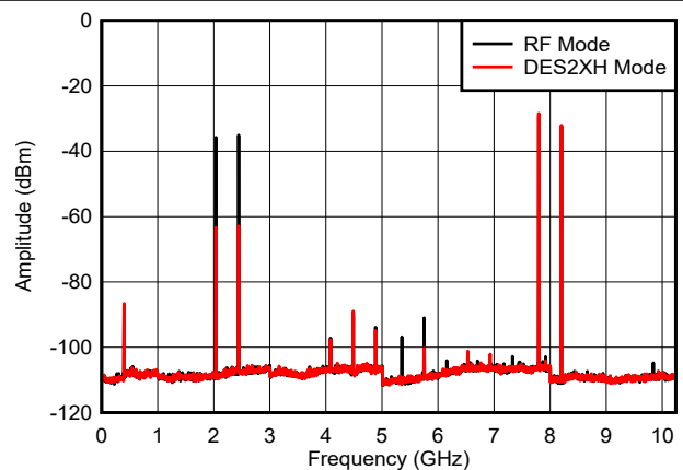
図 6-41. Dual Tone, f_{\text{OUT}} = 7997\text{ MHz} , 0 dBFS
