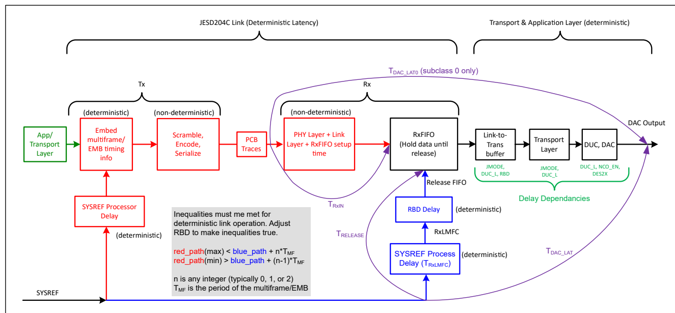
7-57. Definition of Device Latencies
