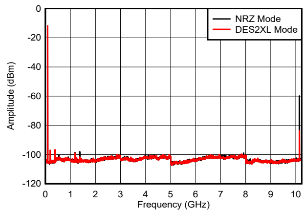
図 6-9. f_{\text{OUT}} = 97\text{ MHz} , -6 dBFS
