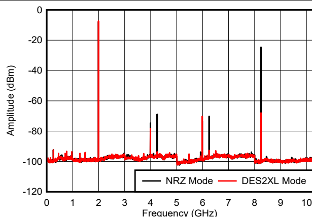
図 6-14. f_{\text{OUT}} = 1997\text{ MHz} , 0 dBFS
