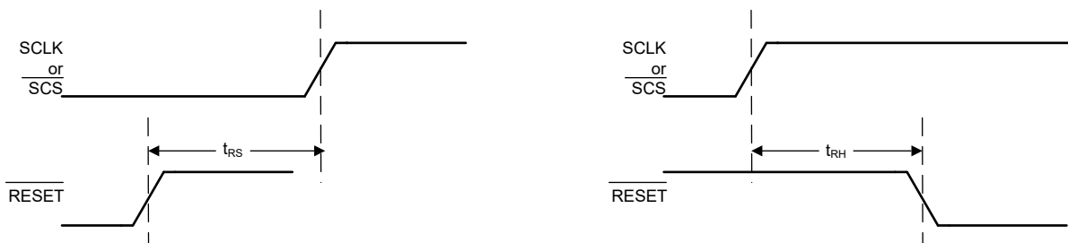
図 6-5. RESET Timing Diagram
