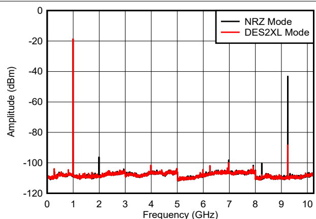
図 6-11. f_{\text{OUT}} = 997\text{ MHz} , 0 dBFS
