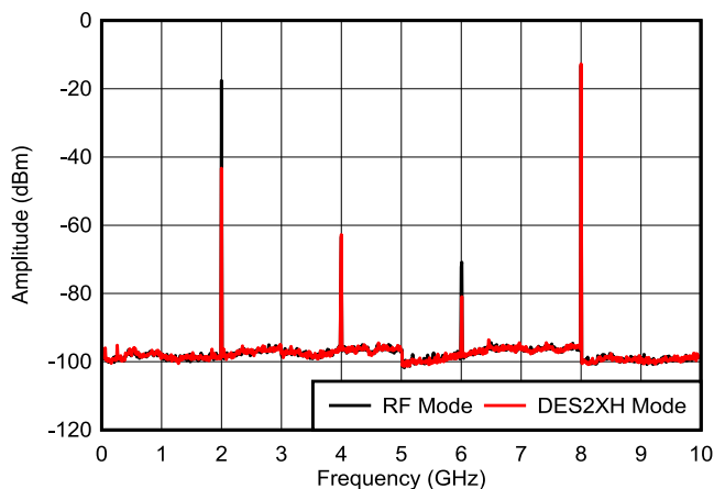
図 8-4. Output Spectra Comparing DES2XH and RF Modes
