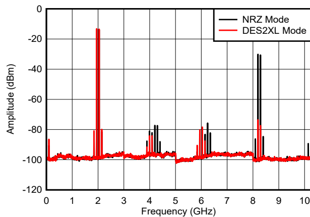
图 6-32. Dual Tone, f_{\text{OUT}} = 1997\text{ MHz} , 0 dBFS
