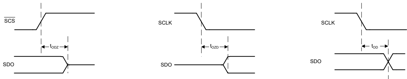
図 6-3. SPI Data Output Timing Diagram
