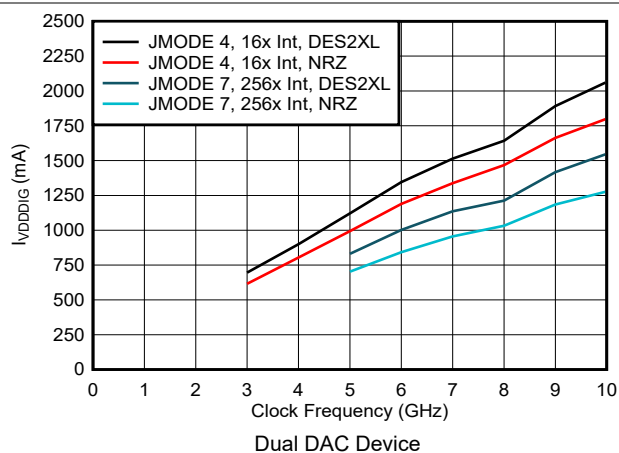
Figure 6-54. VDDDIG Current vs Clock Frequency and Digital Mode
