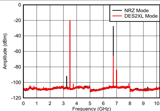
図 6-17. f_{\text{OUT}} = 3497\text{ MHz} , 0 dBFS
