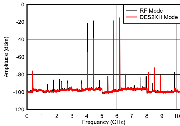
図 6-38. Dual Tone, f_{\text{OUT}} = 5997\text{ MHz} , 0 dBFS
