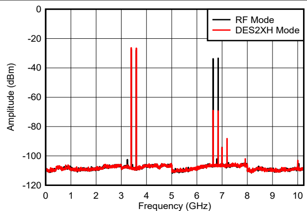
图 6-35. Dual Tone, f_{\text{OUT}} = 3497\text{ MHz} , 0 dBFS
