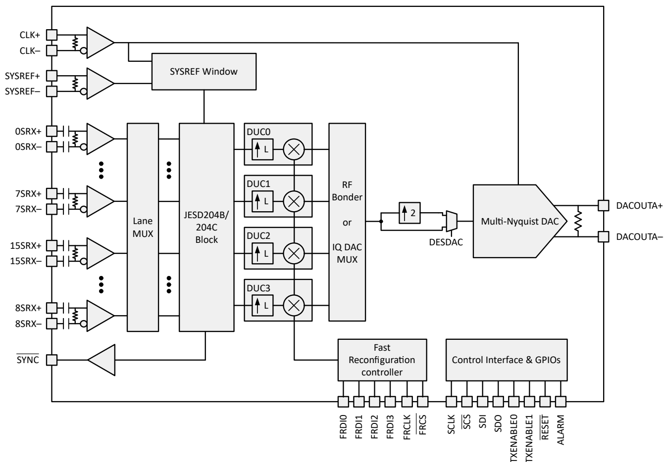
図 7-2. Single Channel Device
