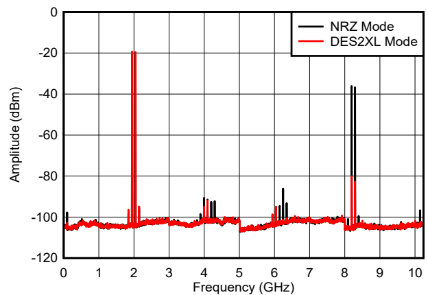
图 6-33. Dual Tone, f_{\text{OUT}} = 1997\text{ MHz} , -6 dBFS
