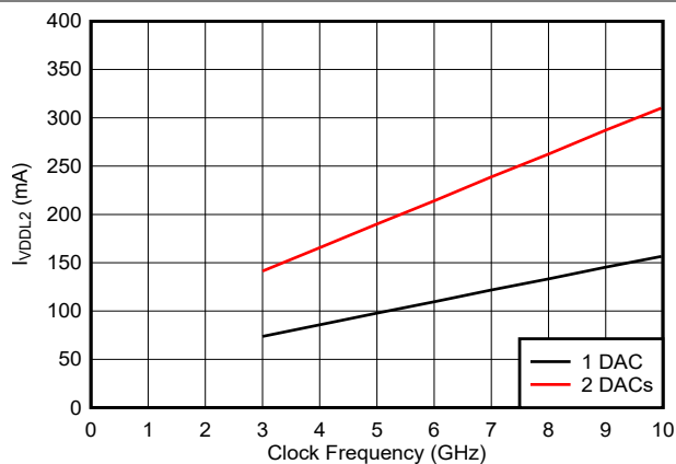
Figure 6-49. VDDLx Current vs Clock Frequency
