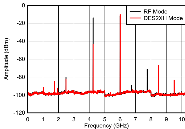
図 6-20. f_{\text{OUT}} = 5997\text{ MHz} , 0 dBFS
