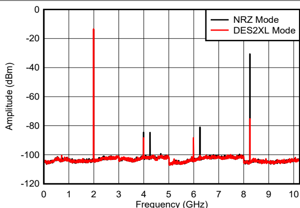
図 6-15. f_{\text{OUT}} = 1997\text{ MHz} , -6 dBFS
