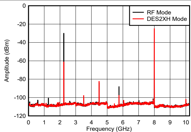
図 6-23. f_{\text{OUT}} = 7997\text{ MHz} , 0 dBFS
