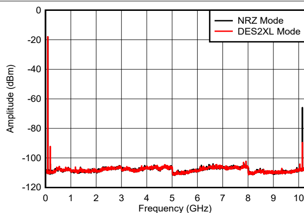
図 6-8. f_{\text{OUT}} = 97\text{ MHz} , 0 dBFS
