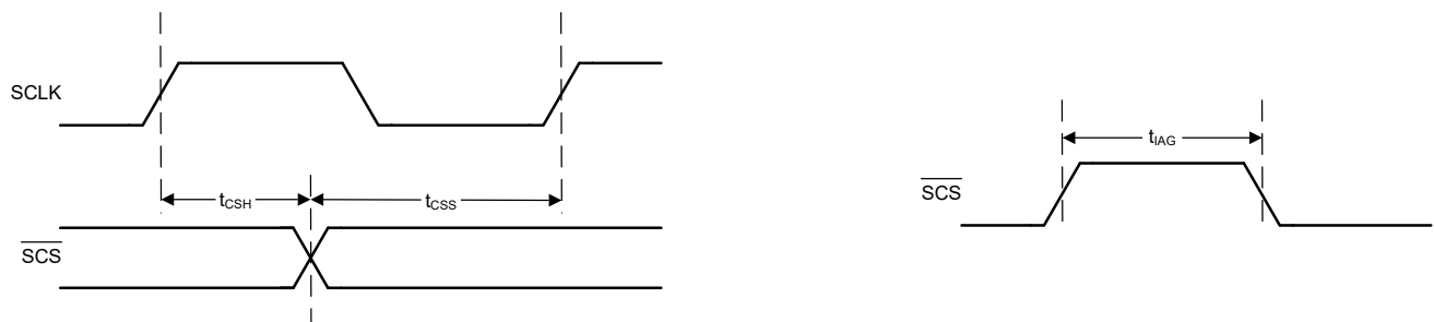
図 6-4. SPI Chip Select Timing Diagram
