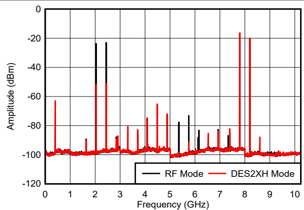
図 6-39. Dual Tone, f_{\text{OUT}} = 5997\text{ MHz} , -6 dBFS
