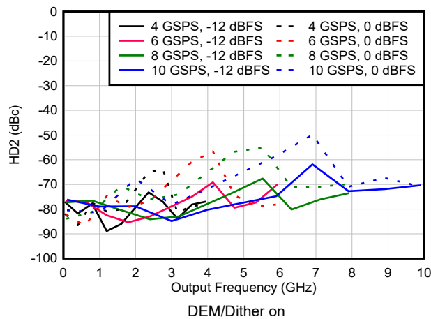
図 6-155. HD2 vs Frequency and Sample Rate in DES2X Modes
