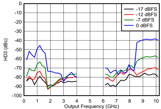
Figure 6-166. HD3 vs Frequency and Digital Amplitude in DES2X Modes
