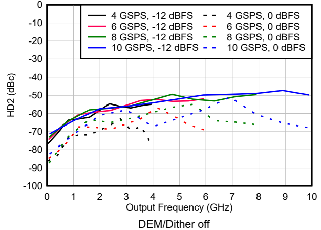
図 6-154. HD2 vs Frequency and Sample Rate in NRZ/RF Modes
