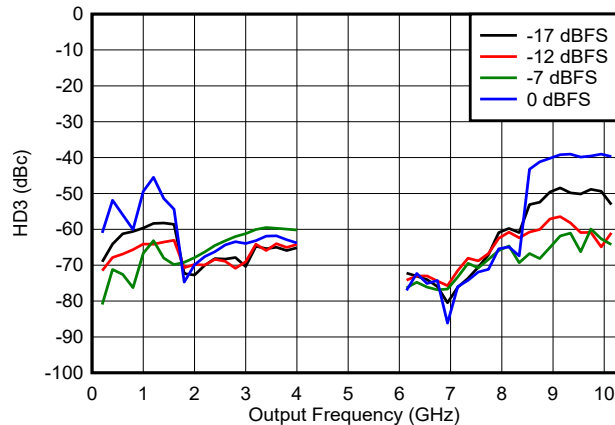
Figure 6-165. HD3 vs Frequency and Digital Amplitude in DES2X Modes
