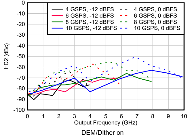
図 6-153. HD2 vs Frequency and Sample Rate in NRZ/RF Modes
