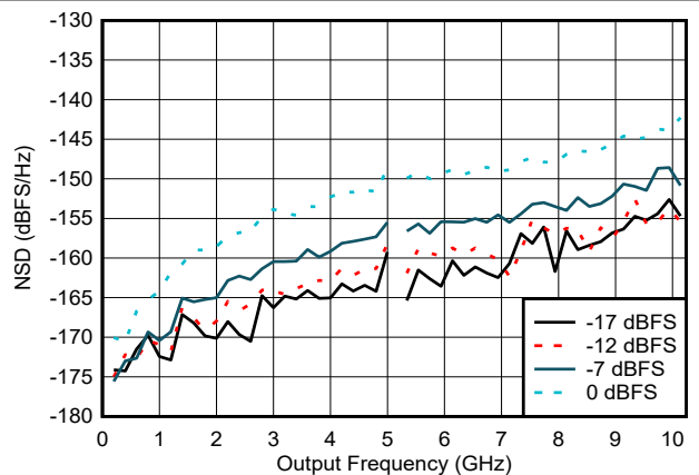
Figure 6-66. NSD vs Output Frequency and Digital Amplitude
