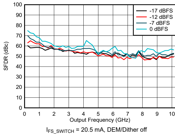
Figure 6-101. SFDR vs Frequency and Digital Amplitude in NRZ/RF Modes
