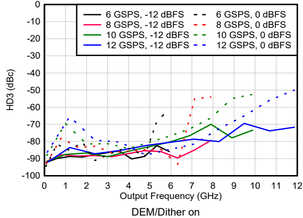
図 6-164. HD3 vs Frequency and Sample Rate in DES2X Modes
