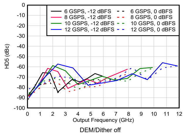
図 6-185. HD5 vs Frequency and Sample Rate in DES2X Modes
