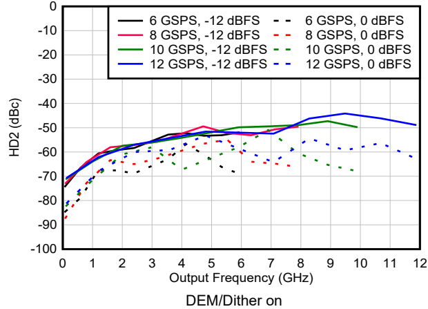
図 6-146. HD2 vs Frequency and Sample Rate in NRZ/RF Modes
