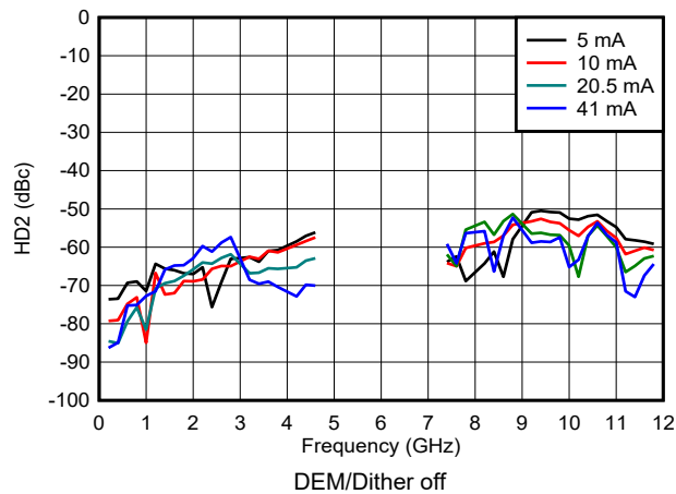
Figure 6-136. HD2 vs Frequency and Output Current in DES2X Modes
