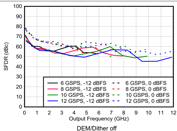
図 6-105. SFDR vs Frequency and Sample Rate in DES2X Modes
