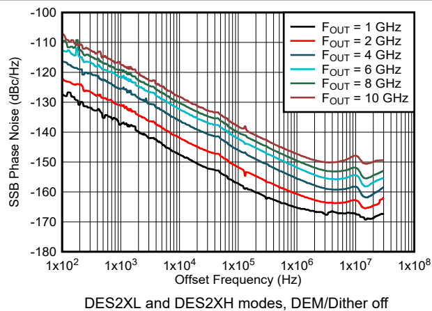
图 6-195. Phase Noise vs Offset Frequency and Output Frequency
