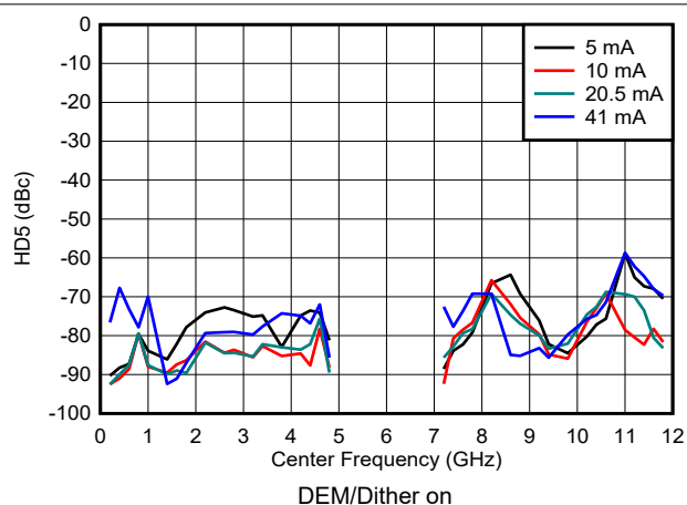
Figure 6-177. HD5 vs Frequency and Output Current in DES2X Modes
