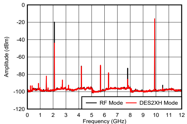
图 6-32. f_{\text{OUT}} = 8097\text{ MHz} , -6 dBFS
