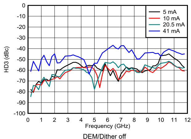
図 6-150. HD3 vs Frequency and Output Current in NRZ/RF Modes
