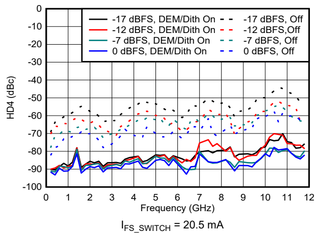
图 6-170. HD4 vs Frequency and Digital Amplitude in NRZ/RF Modes
