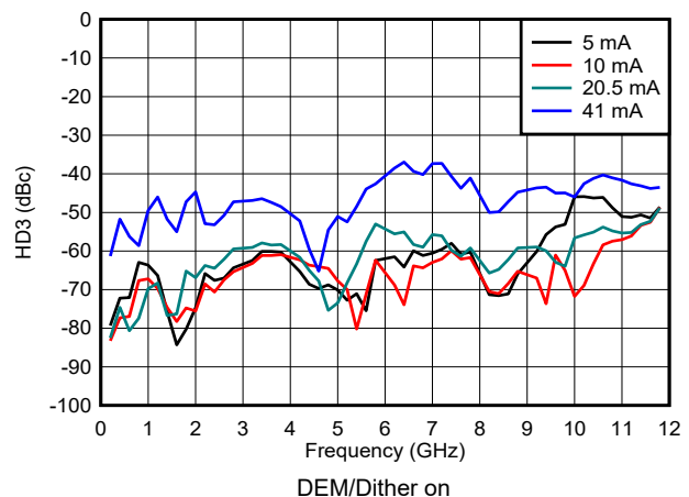
図 6-151. HD3 vs Frequency and Output Current in NRZ/RF Modes
