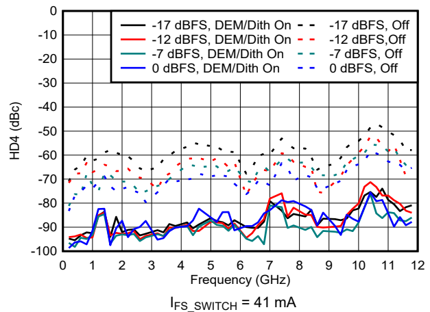
图 6-173. HD4 vs Frequency and Digital Amplitude in NRZ/RF Modes
