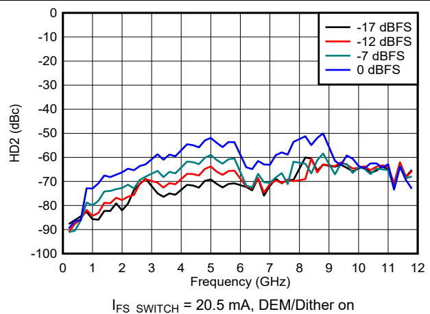
Figure 6-139. HD2 vs Frequency and Digital Amplitude in NRZ/RF Modes
