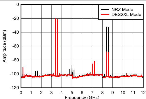
Figure 6-50. Dual Tone, f_{\text{OUT}} = 3497\text{ MHz} , -6 dBFS
