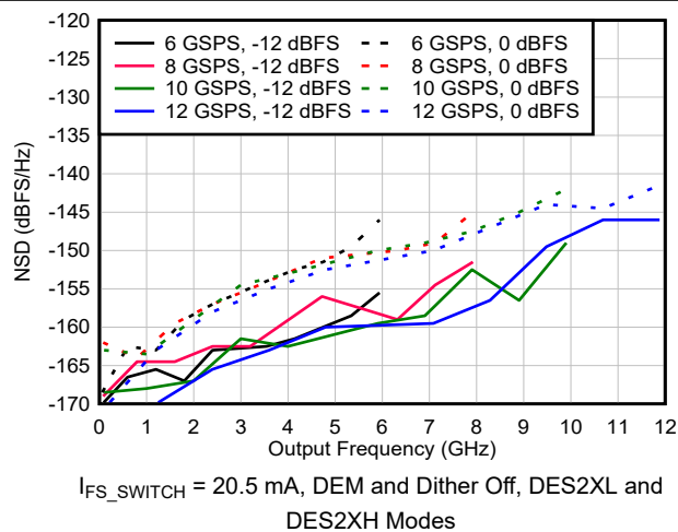
図 6-74. NSD vs Output Frequency and Sample Rate
