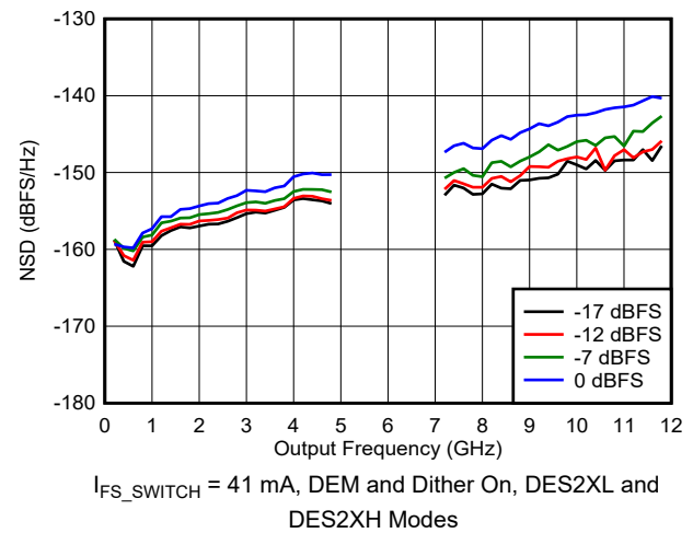
図 6-71. NSD vs Output Frequency and Digital Amplitude
