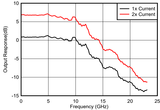
図 6-8. Output Response vs Frequency
