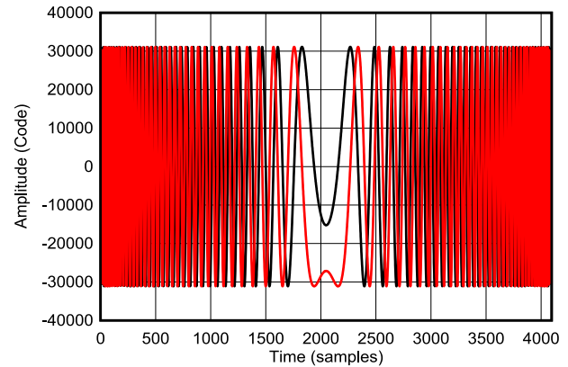
図 8-14. Complex Time Domain of NLFM Chirp (Red = real, Black = imag)
