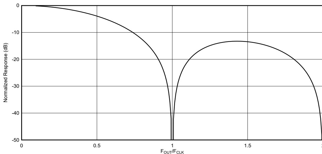
Figure 7-4. NRZ Mode Output Frequency Response
