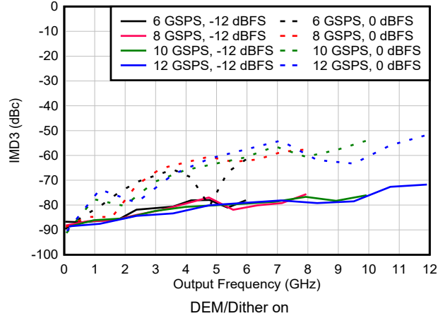
図 6-122. IMD3 vs Frequency and Sample Rate in NRZ/RF Modes
