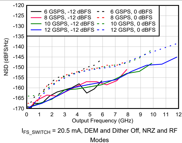
図 6-72. NSD vs Output Frequency and Sample Rate
