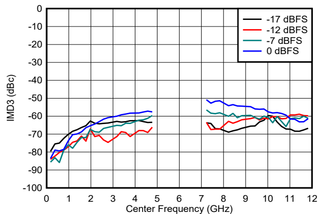
■ 6-112. IMD3 vs Frequency and Digital Amplitude in NRZ/RF Modes
