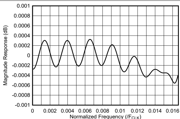
7-29. 24x Interpolation Filter Passband Response
