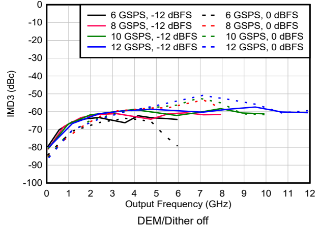
図 6-123. IMD3 vs Frequency and Sample Rate in NRZ/RF Modes
