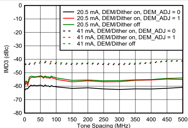
図 6-118. IMD3 vs Tone Spacing in NRZ Mode
