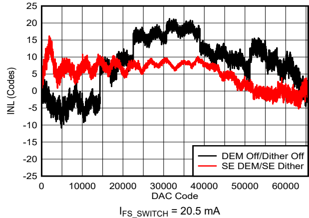
図 6-13. INL vs DAC Code: 20.5 mA
