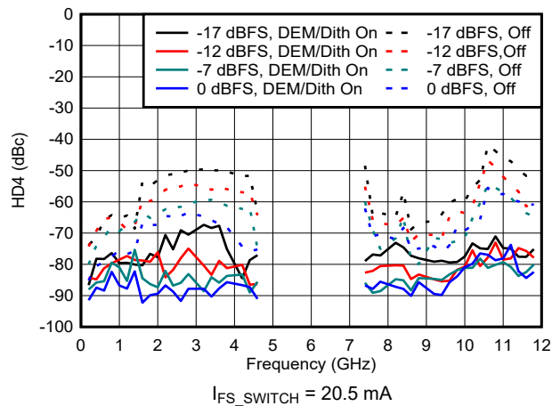
图 6-172. HD4 vs Frequency and Digital Amplitude in NRZ/RF Modes
