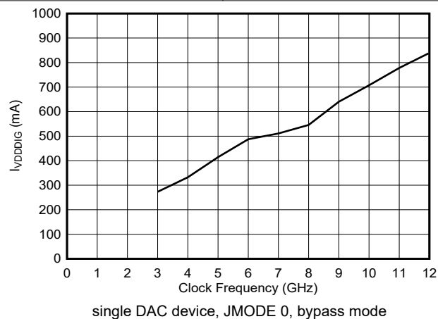
Figure 6-217. VDDDIG Current vs Clock Frequency
