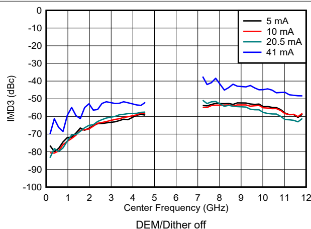
図 6-108. IMD3 vs Frequency and Output Current in DES2X Modes
