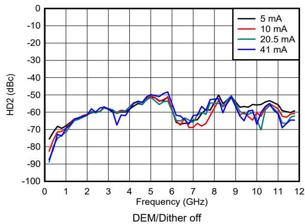
Figure 6-134. HD2 vs Frequency and Output Current in NRZ/RF Modes
