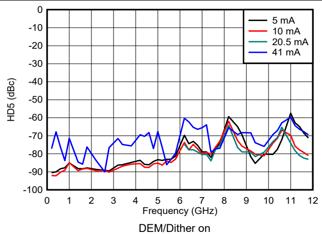
图 6-175. HD5 vs Frequency and Output Current in NRZ/RF Modes
