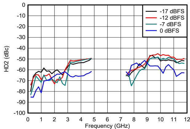
■ 6-140. HD2 vs Frequency and Digital Amplitude in NRZ/RF Modes
