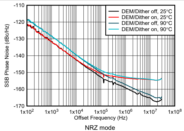
图 6-196. Phase Noise vs Offset Frequency at 1 GHz
