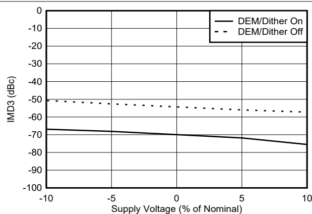
図 6-132. IMD3 vs Voltage in RF Mode at 9002 MHz
