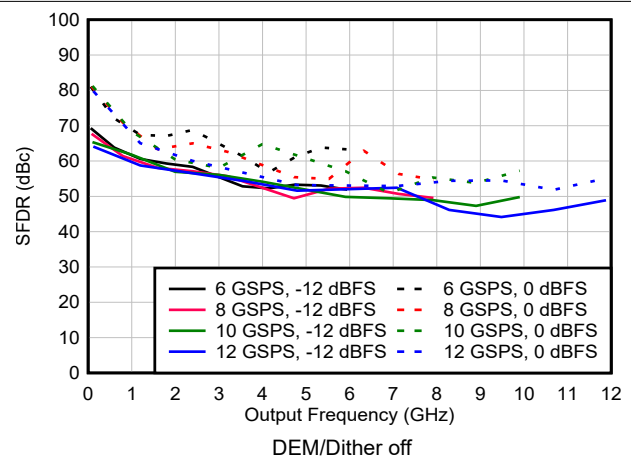
Figure 6-103. SFDR vs Frequency and Sample Rate in NRZ/RF Modes
