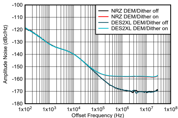
Figure 6-200. Amplitude Noise vs Offset Frequency at 1 GHz
