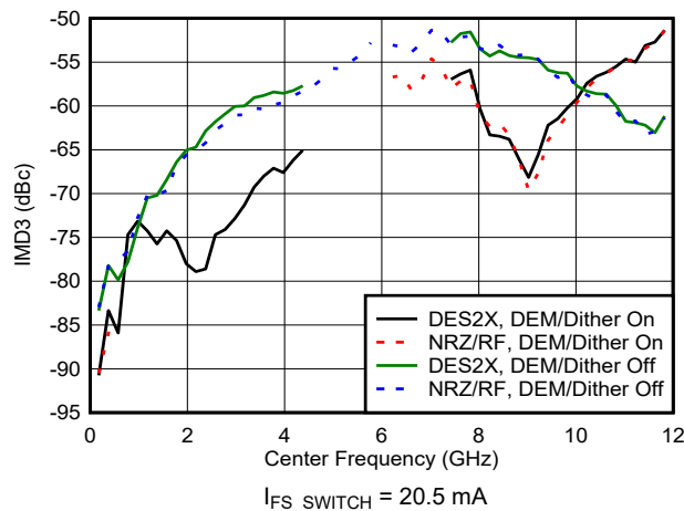
図 6-84. IMD3 vs Frequency and Mode
