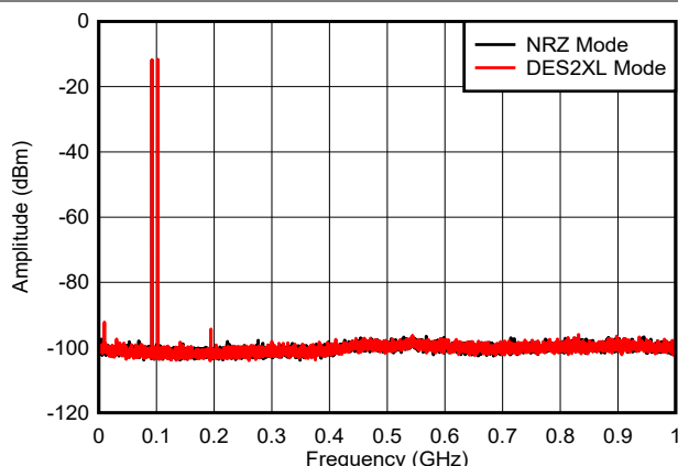
6-38. Dual Tone, f_{\text{OUT}} = 97\text{ MHz} , 0 dBFS (0 - 1 GHz)
