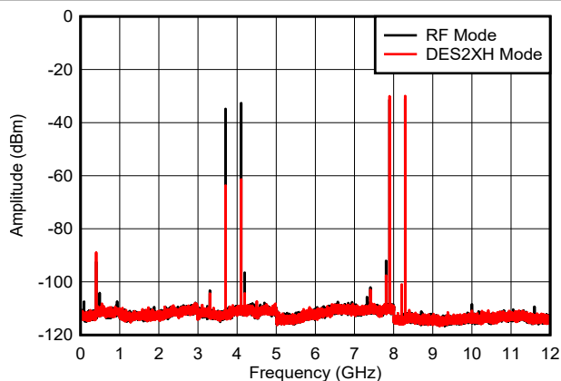
Figure 6-52. Dual Tone, f_{\text{OUT}} = 8097\text{ MHz} , 0 dBFS
