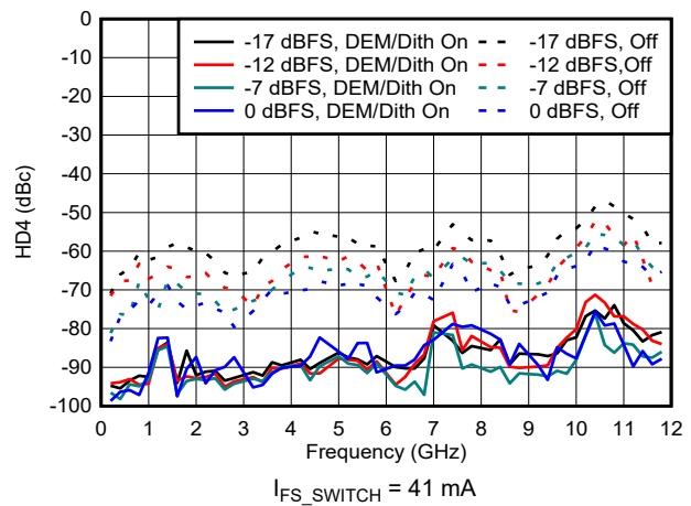
图 6-171. HD4 vs Frequency and Digital Amplitude in NRZ/RF Modes
