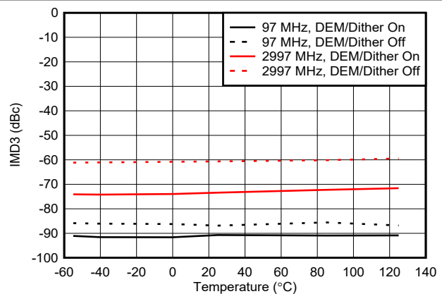
図 6-127. IMD3 vs Temperature in DES2XL Mode
