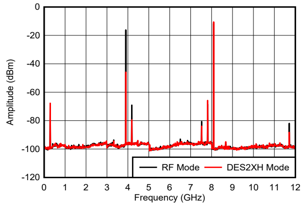
图 6-31. f_{\text{OUT}} = 8097\text{ MHz} , 0 dBFS
