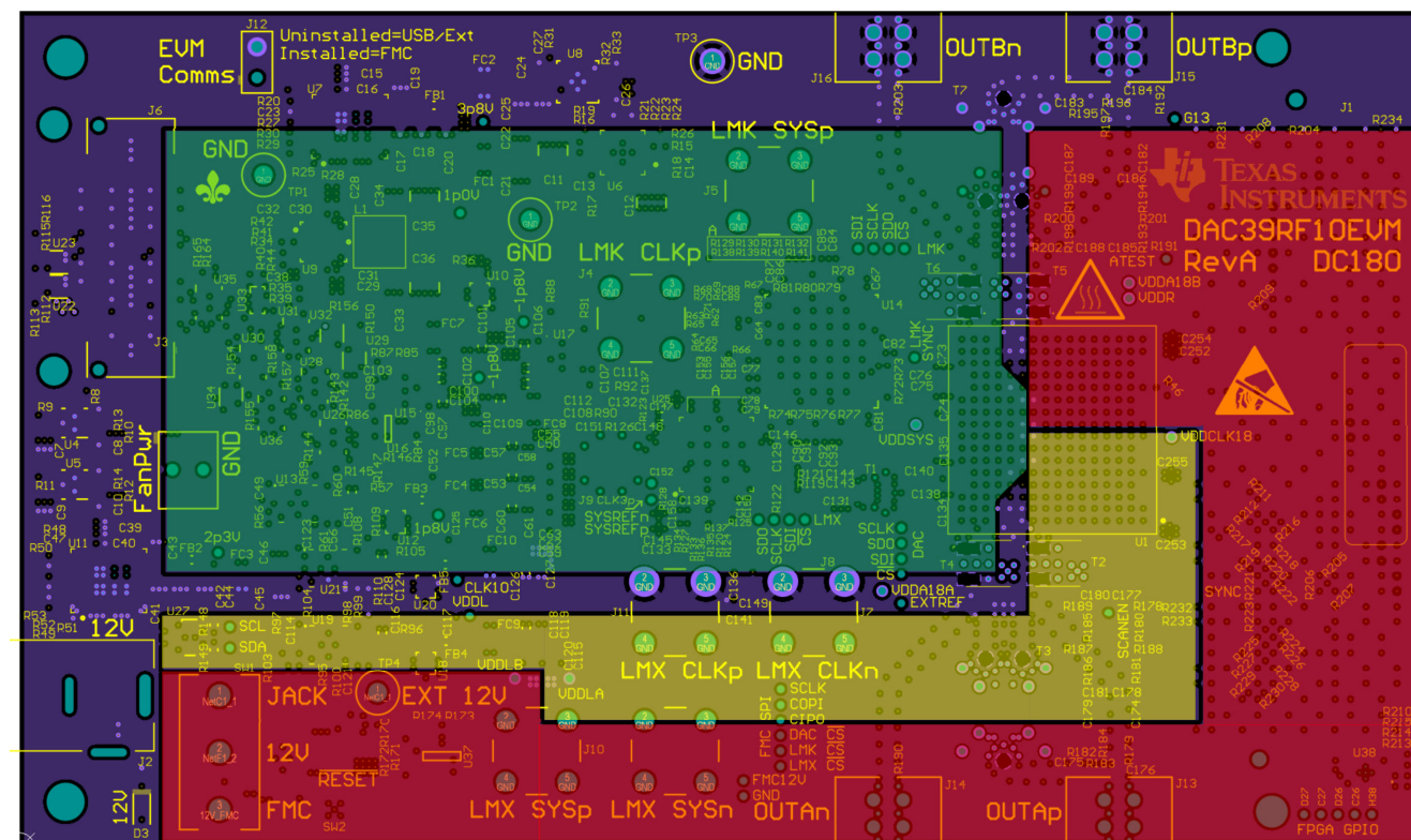
Layer5 / PWR2 DAC VDDL A = RED DAC VDDL B = YELLOW DAC VDDCLK1P0V = GREEN ❑ 8-31. Power Plane Layout for Layer 5
