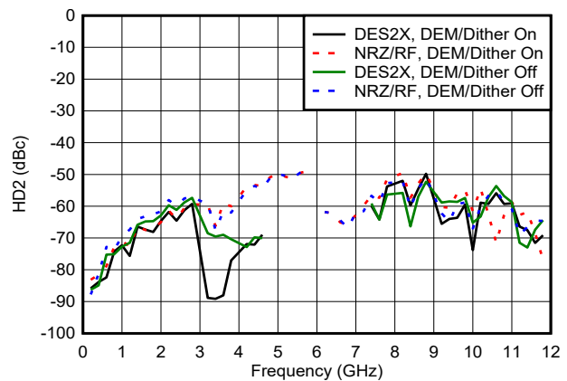
図 6-87. HD2 vs Frequency and Mode
