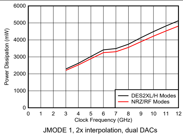
Figure 6-206. Power Dissipation vs Clock Frequency and DAC Mode
