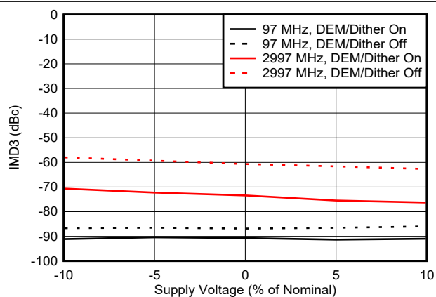
図 6-131. IMD3 vs Voltage in DES2XL Mode
