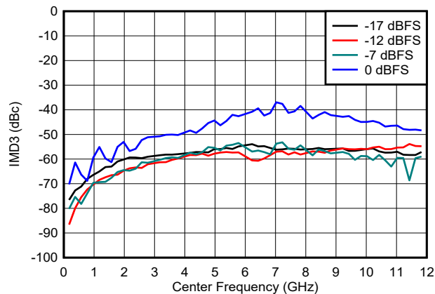
■ 6-110. IMD3 vs Frequency and Digital Amplitude in NRZ/RF Modes
