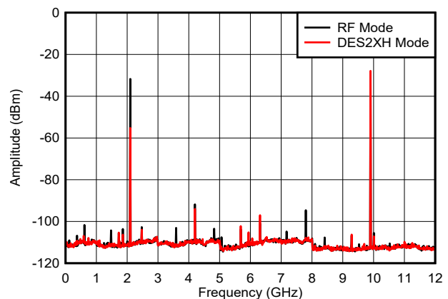
图 6-34. f_{\text{OUT}} = 9897\text{ MHz} , 0 dBFS
