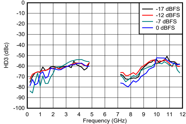
FIG 6-158. HD3 vs Frequency and Digital Amplitude in DES2X Modes
