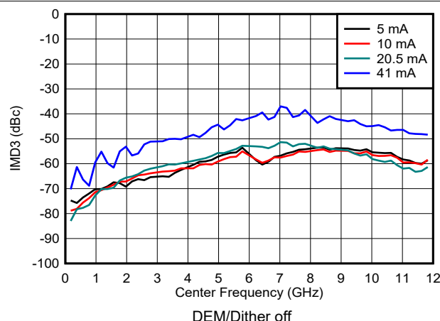
図 6-106. IMD3 vs Frequency and Output Current in NRZ/RF Modes
