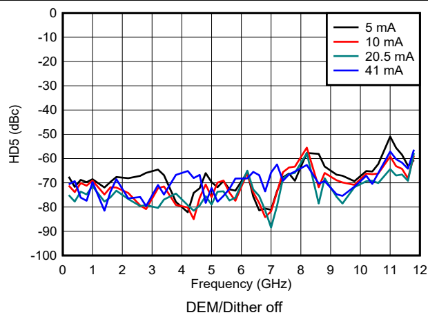
图 6-174. HD5 vs Frequency and Output Current in NRZ/RF Modes
