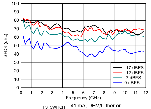
Figure 6-97. SFDR vs Frequency and Digital Amplitude in NRZ/RF Modes
