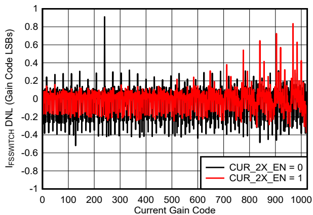
FIG 6-18. I_{\text{FS\_SWITCH}} Error Differential Non-Linearity vs Gain Code
