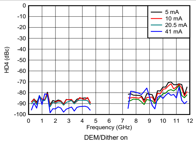
図 6-169. HD4 vs Frequency and Output Current in DES2X Modes
