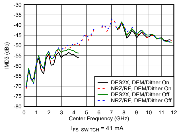
図 6-85. IMD3 vs Frequency and Mode
