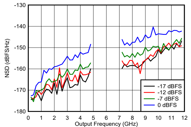
Figure 6-67. NSD vs Output Frequency and Digital Amplitude
