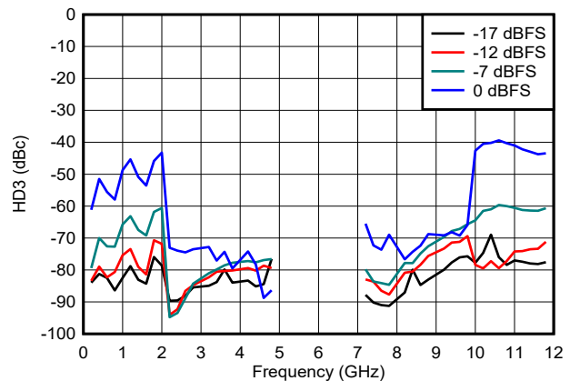
FIG 6-159. HD3 vs Frequency and Digital Amplitude in DES2X Modes
