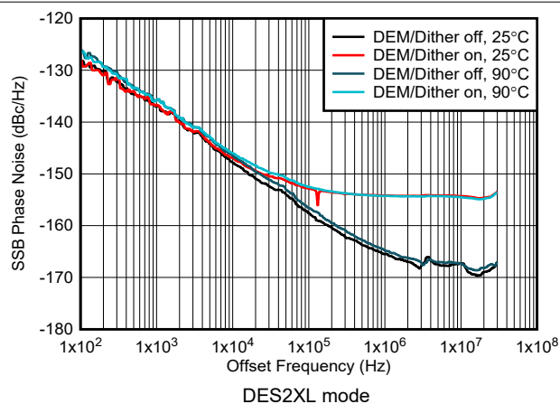
图 6-197. Phase Noise vs Offset Frequency at 1 GHz
