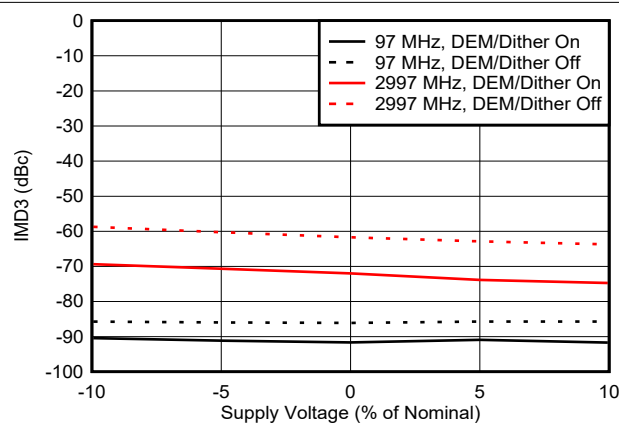
図 6-130. IMD3 vs Voltage in NRZ Mode
