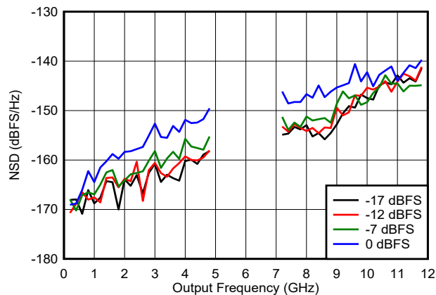
Figure 6-66. NSD vs Output Frequency and Digital Amplitude
