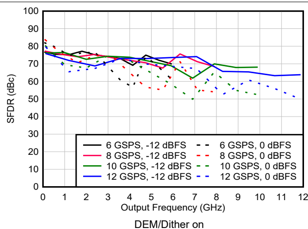
図 6-104. SFDR vs Frequency and Sample Rate in DES2X Modes
