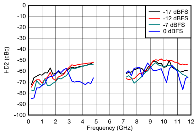
■ 6-142. HD2 vs Frequency and Digital Amplitude in DES2X Modes
