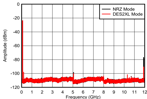
6-39. Dual Tone, f_{\text{OUT}} = 97\text{ MHz} , -6 dBFS (0 - f_{\text{CLK}} )
