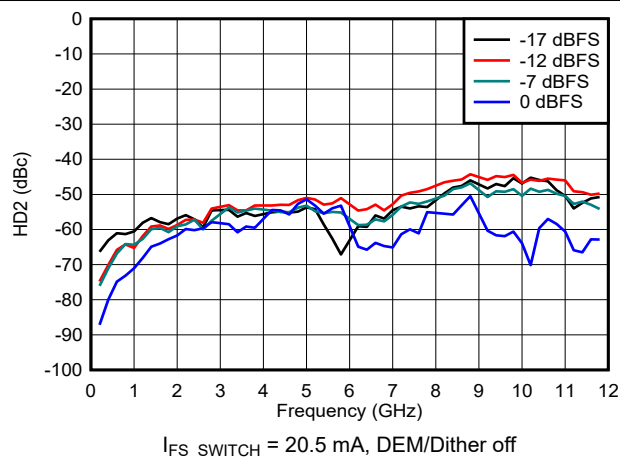
Figure 6-138. HD2 vs Frequency and Digital Amplitude in NRZ/RF Modes
