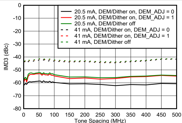
図 6-119. IMD3 vs Tone Spacing in DES2XL Mode
