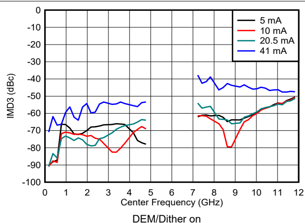
図 6-109. IMD3 vs Frequency and Output Current in DES2X Modes
