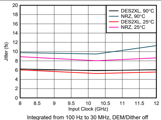
图 6-198. Jitter vs Input Clock
