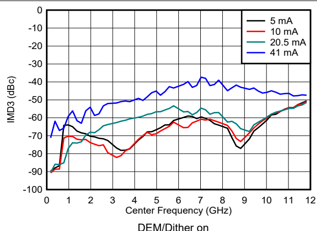
図 6-107. IMD3 vs Frequency and Output Current in NRZ/RF Modes
