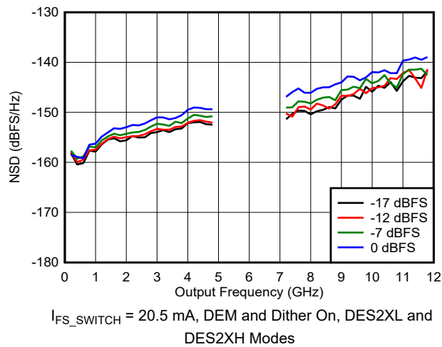
図 6-70. NSD vs Output Frequency and Digital Amplitude
