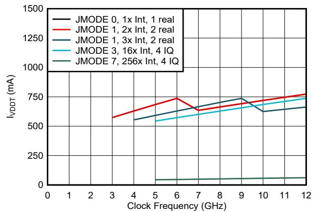
Figure 6-215. VDDT Current vs Clock Frequency and Mode
