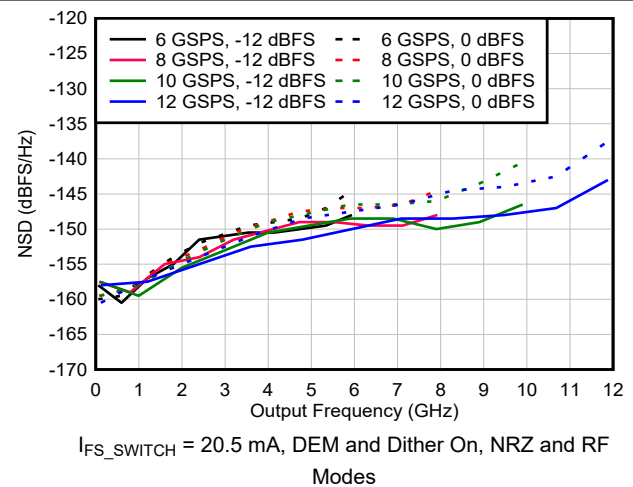
図 6-73. NSD vs Output Frequency and Sample Rate
