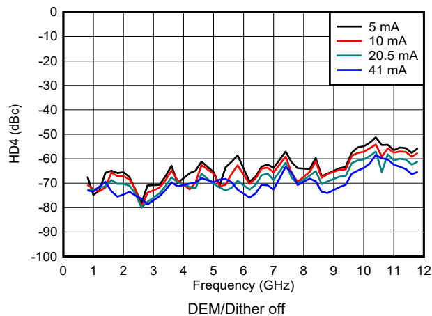
図 6-166. HD4 vs Frequency and Output Current in NRZ/Rf Modes
