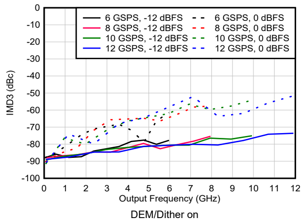
図 6-124. IMD3 vs Frequency and Sample Rate in DES2X Modes
