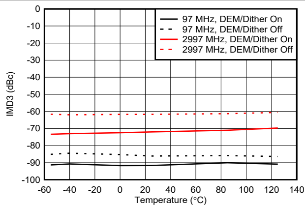
図 6-126. IMD3 vs Temperature in NRZ Mode
