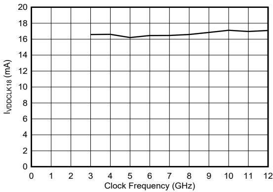
FIG 6-209. VDDCLK18 Current vs Clock Frequency
