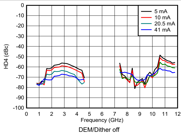
図 6-168. HD4 vs Frequency and Output Current in DES2X Modes
