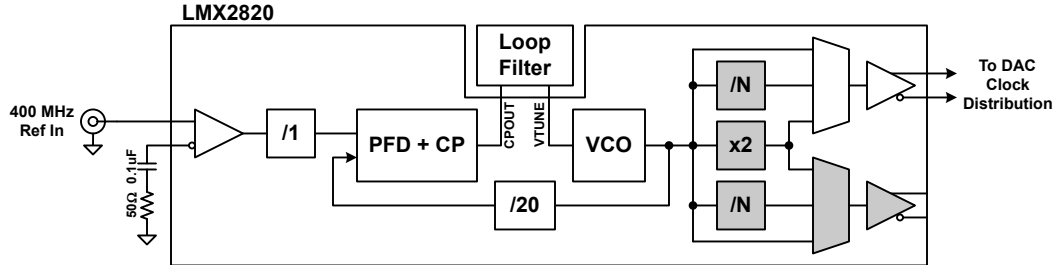
8-7. LMX2820 with Internal VCO
