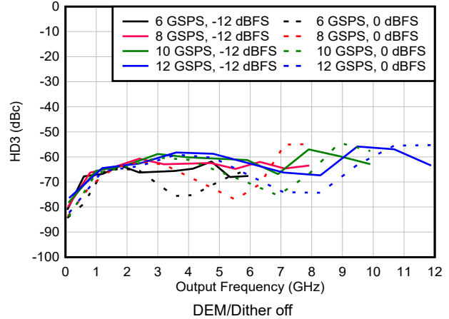
図 6-165. HD3 vs Frequency and Sample Rate in DES2X Modes
