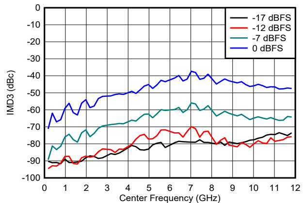
■ 6-111. IMD3 vs Frequency and Digital Amplitude in NRZ/RF Modes
