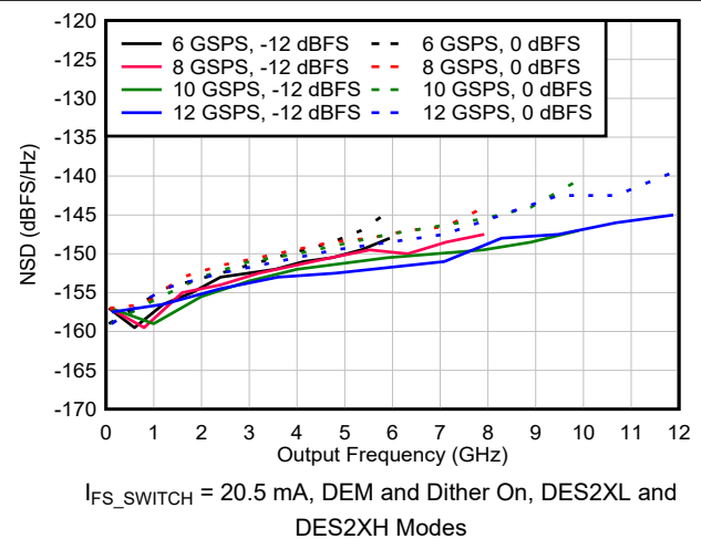
図 6-75. NSD vs Output Frequency and Sample Rate
