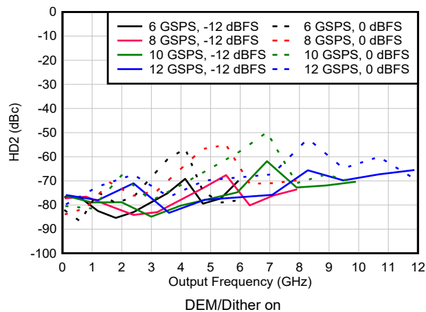
図 6-148. HD2 vs Frequency and Sample Rate in DES2X Modes
