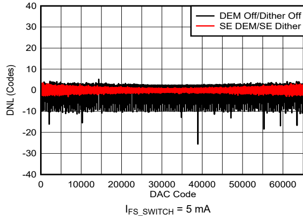
図 6-12. DNL vs DAC Code: 5 mA
