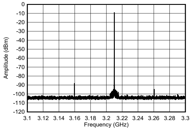
図 8-19. In Band Single Tone Frequency Spectra with f_{OUT} = 3.211 GHz
