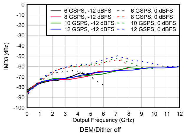
図 6-125. IMD3 vs Frequency and Sample Rate in DES2X Modes
