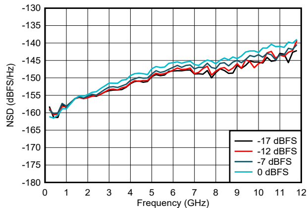
Figure 6-64. NSD vs Output Frequency and Digital Amplitude
