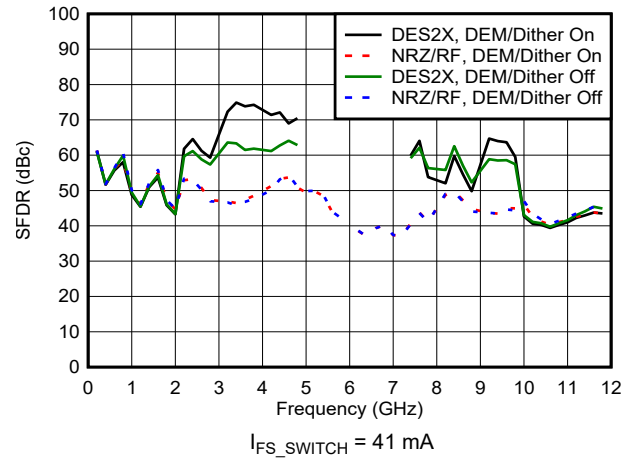
図 6-83. SFDR vs Frequency and Mode
