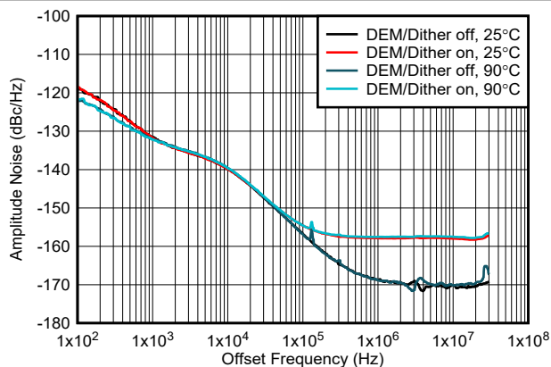
Figure 6-202. Amplitude Noise vs Offset Frequency and Temperature at 1 GHz
