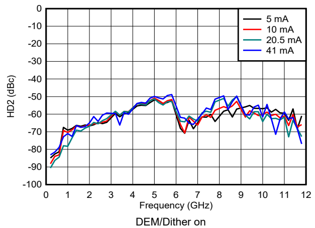
Figure 6-135. HD2 vs Frequency and Output Current in NRZ/RF Modes
