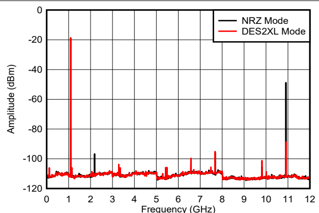
图 6-22. f_{\text{OUT}} = 1097\text{ MHz} , 0 dBFS
