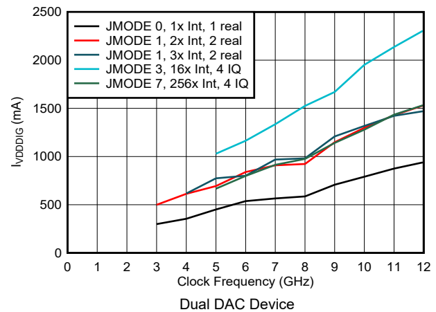
Figure 6-216. VDDDIG Current vs Clock Frequency and Digital Mode
