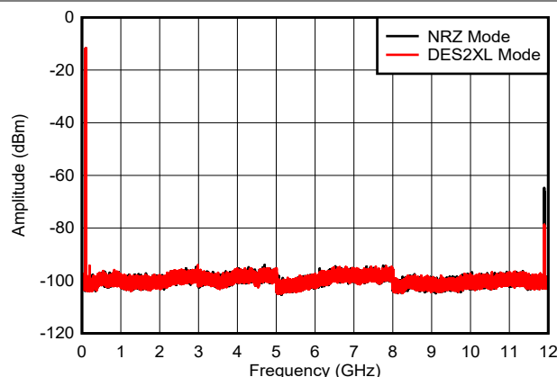
6-37. Dual Tone, f_{\text{OUT}} = 97\text{ MHz} , 0 dBFS (0 - f_{\text{CLK}} )
