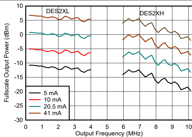
図 6-8. Output Response vs Frequency
