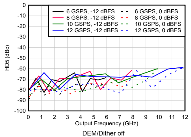
図 6-183. HD5 vs Frequency and Sample Rate in NRZ/RF Modes
