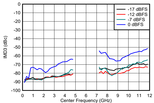
■ 6-113. IMD3 vs Frequency and Digital Amplitude in NRZ/RF Modes
