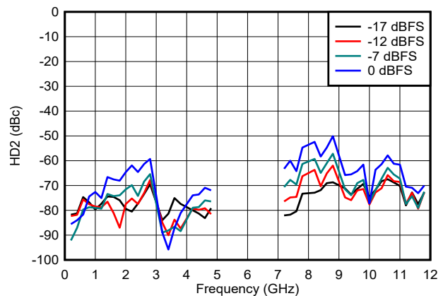
■ 6-143. HD2 vs Frequency and Digital Amplitude in DES2X Modes
