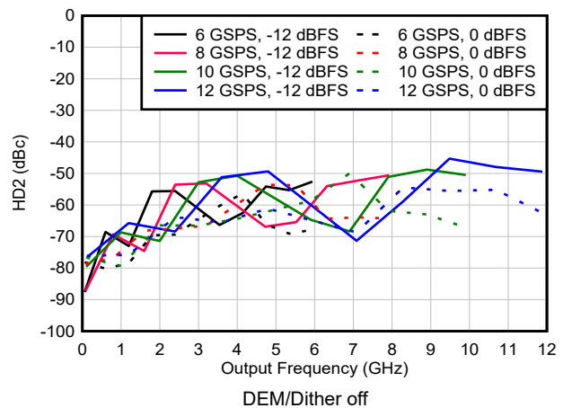
図 6-149. HD2 vs Frequency and Sample Rate in DES2X Modes
