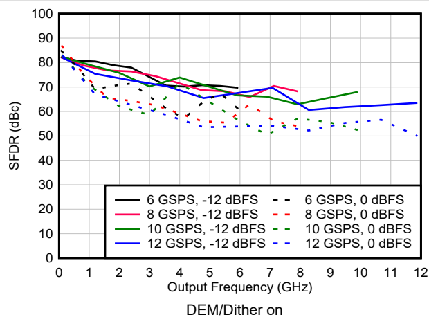
Figure 6-102. SFDR vs Frequency and Sample Rate in NRZ/RF Modes
