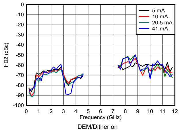
Figure 6-137. HD2 vs Frequency and Output Current in DES2X Modes
