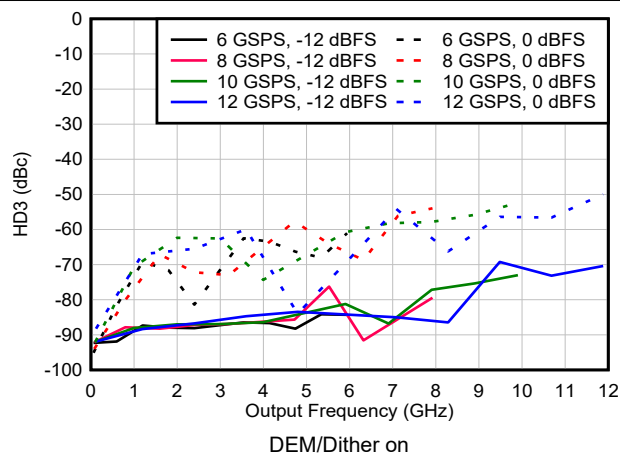
FIG 6-162. HD3 vs Frequency and Sample Rate in NRZ/RF Modes
