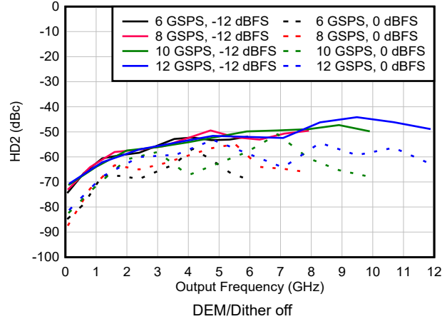
図 6-147. HD2 vs Frequency and Sample Rate in NRZ/RF Modes
