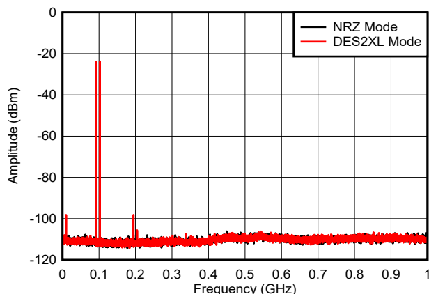
6-40. Dual Tone, f_{\text{OUT}} = 97\text{ MHz} , -6 dBFS (0 - 1 GHz)
