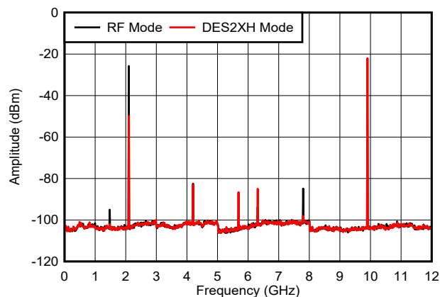
图 6-33. f_{\text{OUT}} = 8097\text{ MHz} , -12 dBFS
