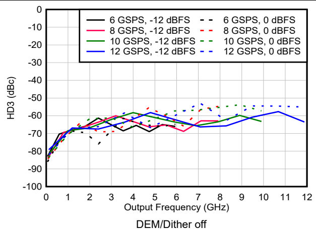
FIG 6-163. HD3 vs Frequency and Sample Rate in NRZ/RF Modes
