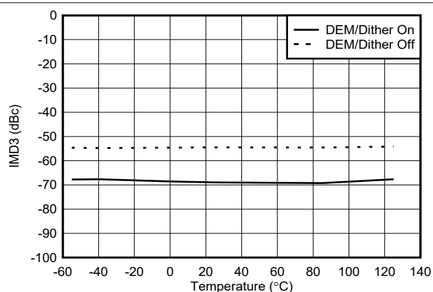
図 6-129. IMD3 vs Temperature in DES2XH Mode at 9002 MHz
