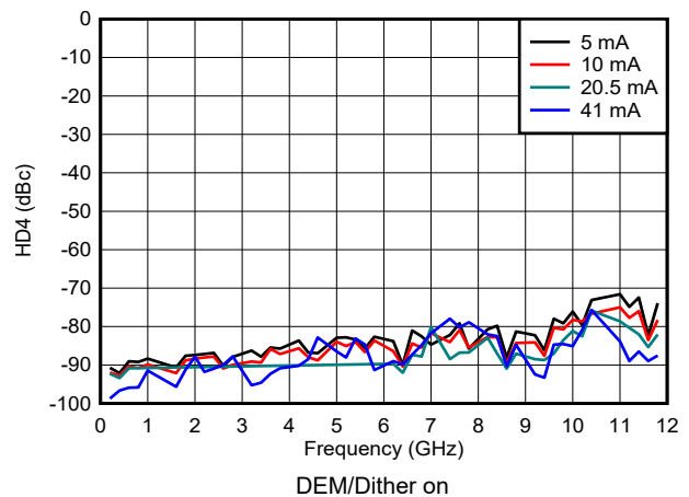
図 6-167. HD4 vs Frequency and Output Current in NRZ/Rf Modes
