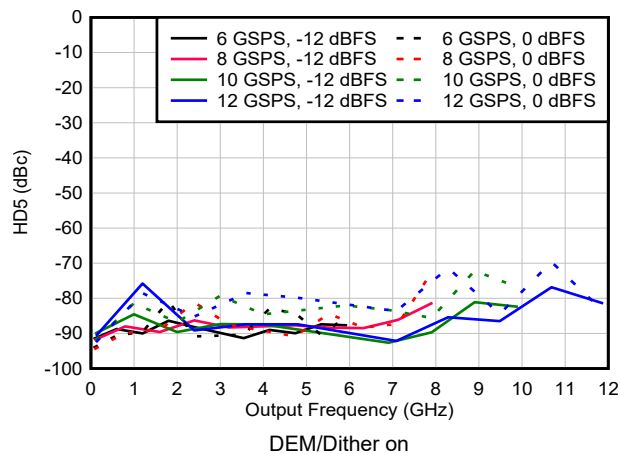
図 6-184. HD5 vs Frequency and Sample Rate in DES2X Modes
