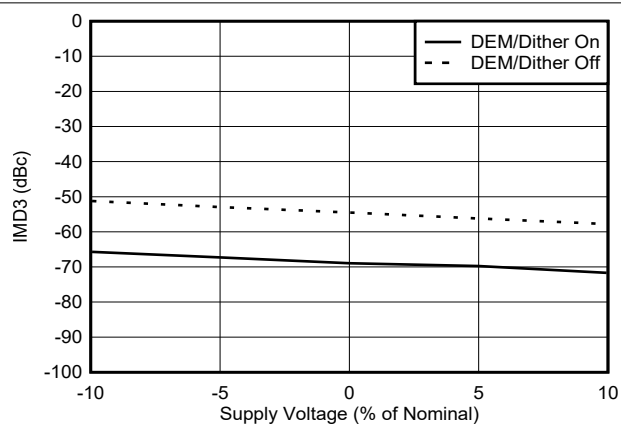
図 6-133. IMD3 vs Voltage in DES2XH Mode at 9002 MHz
