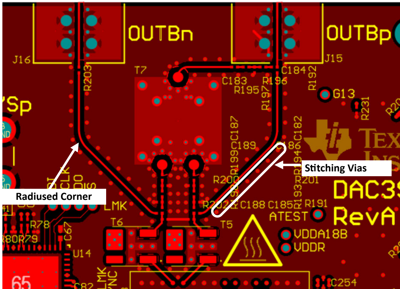
✎ 8-23. Radius Corner and Stitch Vias next to High_Speed Signal Trace
