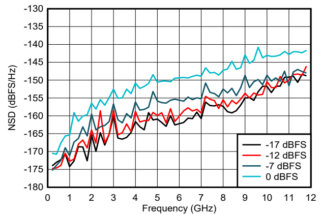
Figure 6-65. NSD vs Output Frequency and Digital Amplitude
