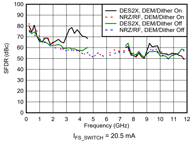
図 6-82. SFDR vs Frequency and Mode
