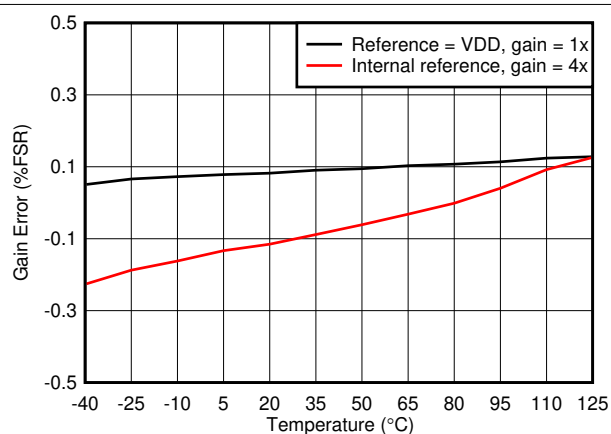
7-19. Gain Error vs Temperature
