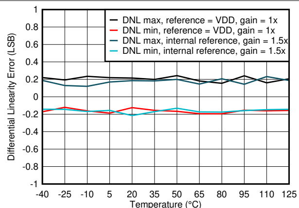
FIG 7-5. Differential Linearity Error vs Temperature
