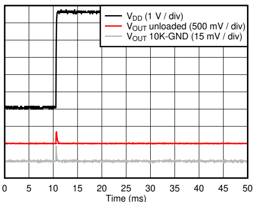
7-39. Power-on Glitch
