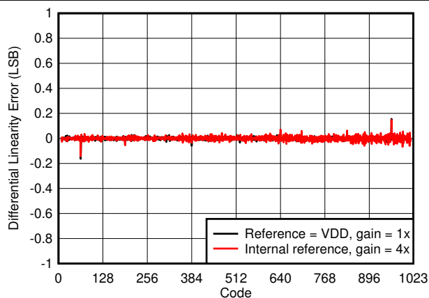
FIG 7-12. Differential Linearity Error vs Digital Input Code
