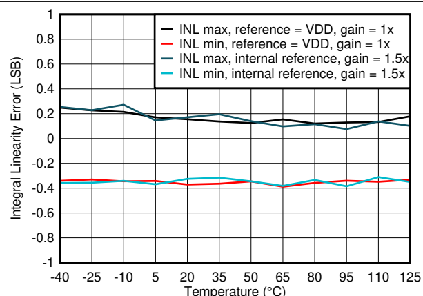
FIG 7-4. Integral Linearity Error vs Temperature
