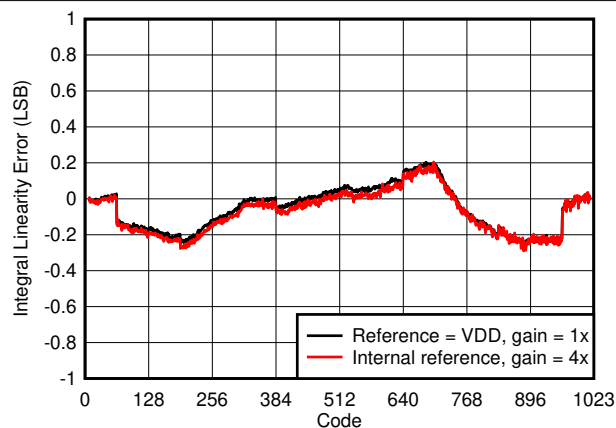
FIG 7-11. Integral Linearity Error vs Digital Input Code
