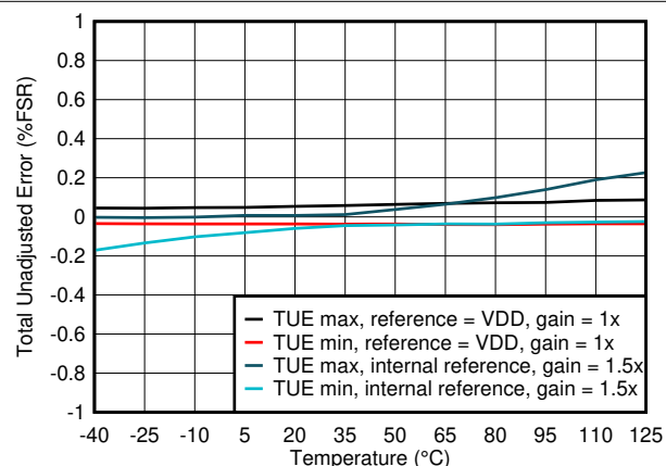
FIG 7-6. Total Unadjusted Error vs Temperature
