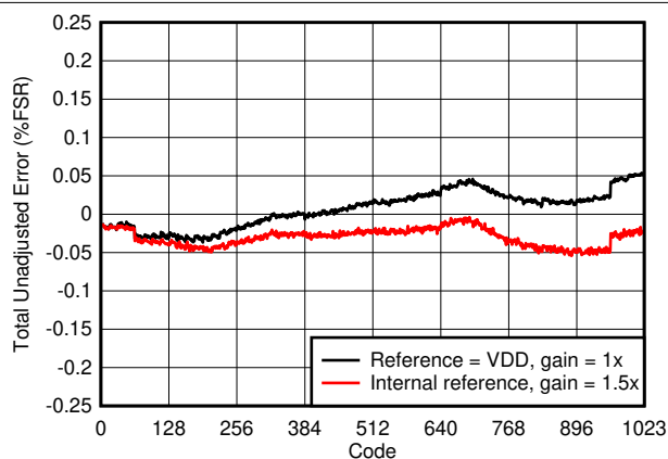
FIG 7-3. Total Unadjusted Error vs Digital Input Code
