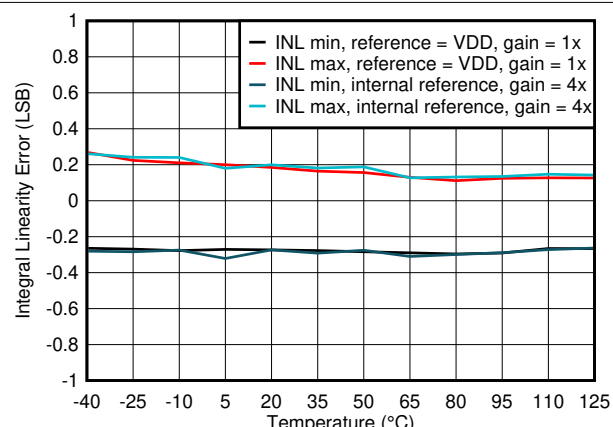
FIG 7-14. Integral Linearity Error vs Temperature
