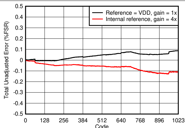
FIG 7-13. Total Unadjusted Error vs Digital Input Code
