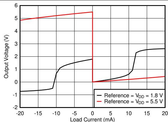
FIG 7-34. Source and Sink Capability
