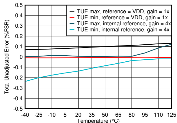
FIG 7-16. Total Unadjusted Error vs Temperature
