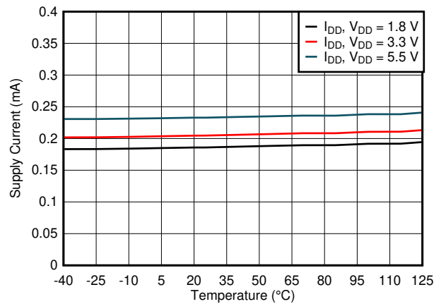
7-30. Supply Current vs Temperature
