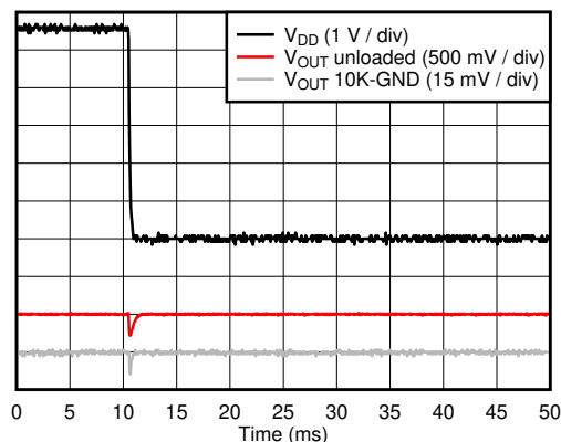
7-40. Power-off Glitch
