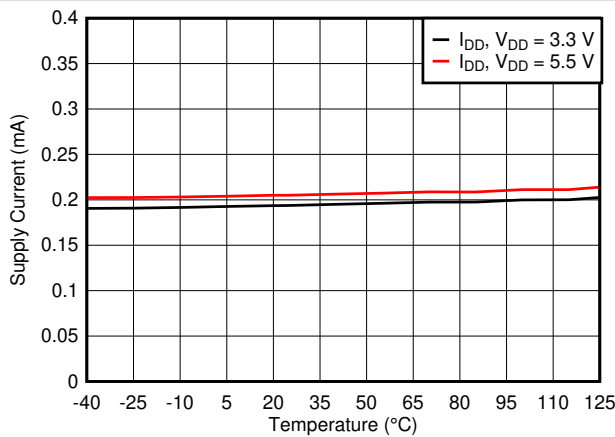
7-31. Supply Current vs Temperature
