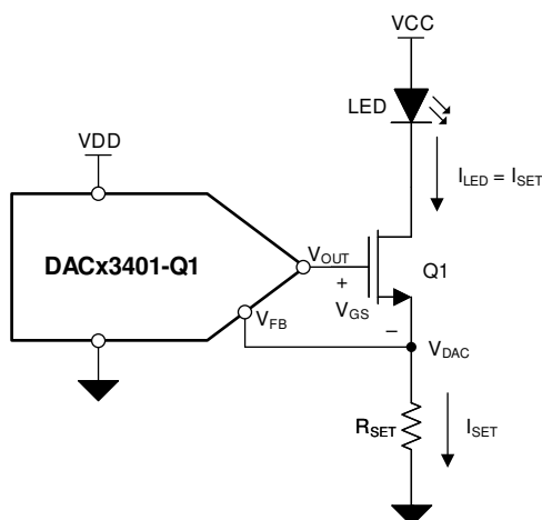
図 9-1. LED Biasing
