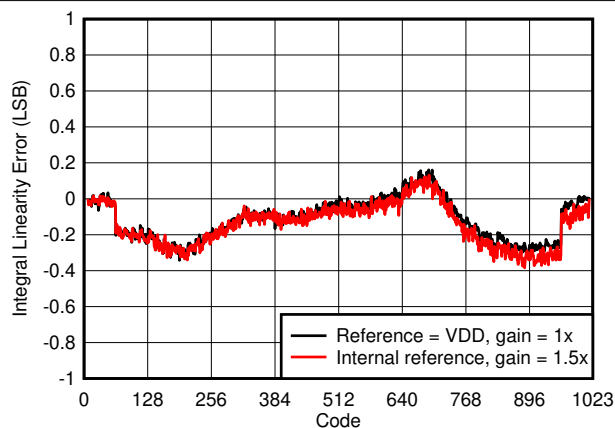
FIG 7-1. Integral Linearity Error vs Digital Input Code
