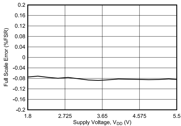
7-27. Full-Scale Error vs Supply Voltage
