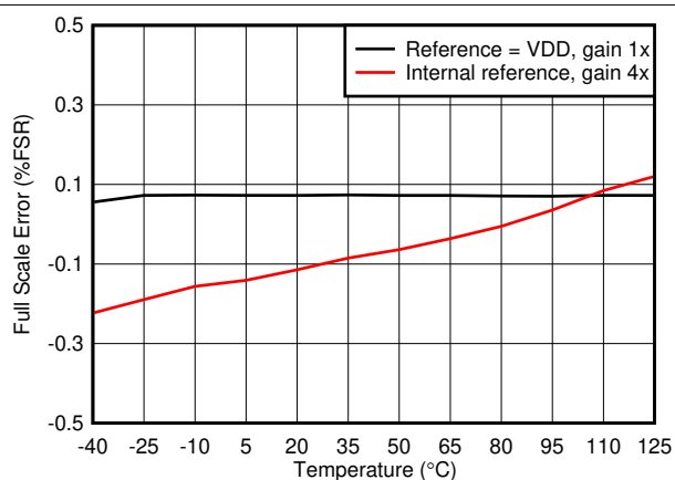
7-20. Full-Scale Error vs Temperature
