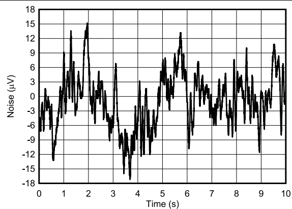
FIG 7-45. DAC Output Noise: 0.1 Hz to 10 Hz
