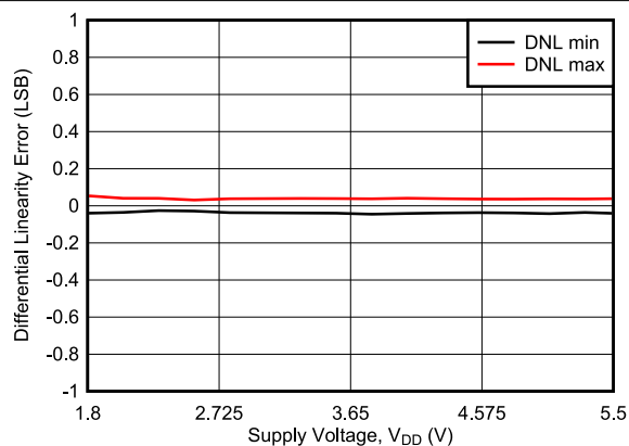
FIG 7-22. Differential Linearity Error vs Supply Voltage
