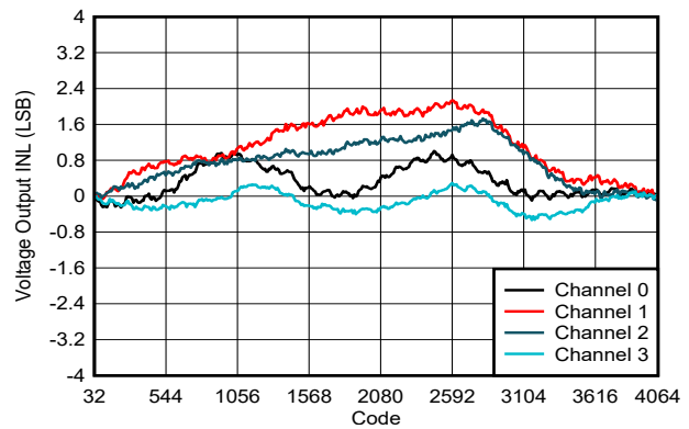
FIG 6-5. Voltage Output INL vs Digital Input Code
