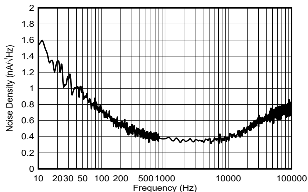
6-56. Current Output Noise Density
