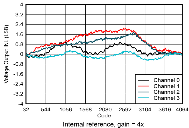
FIG 6-4. Voltage Output INL vs Digital Input Code
