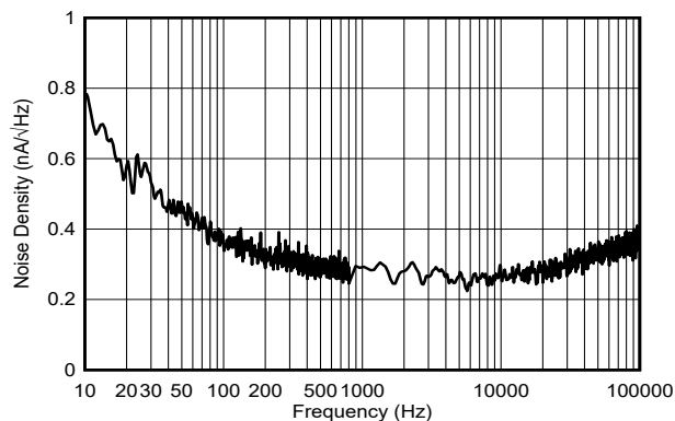
6-55. Current Output Noise Density
