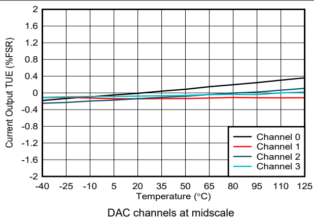
6-44. Current Output TUE vs Temperature
