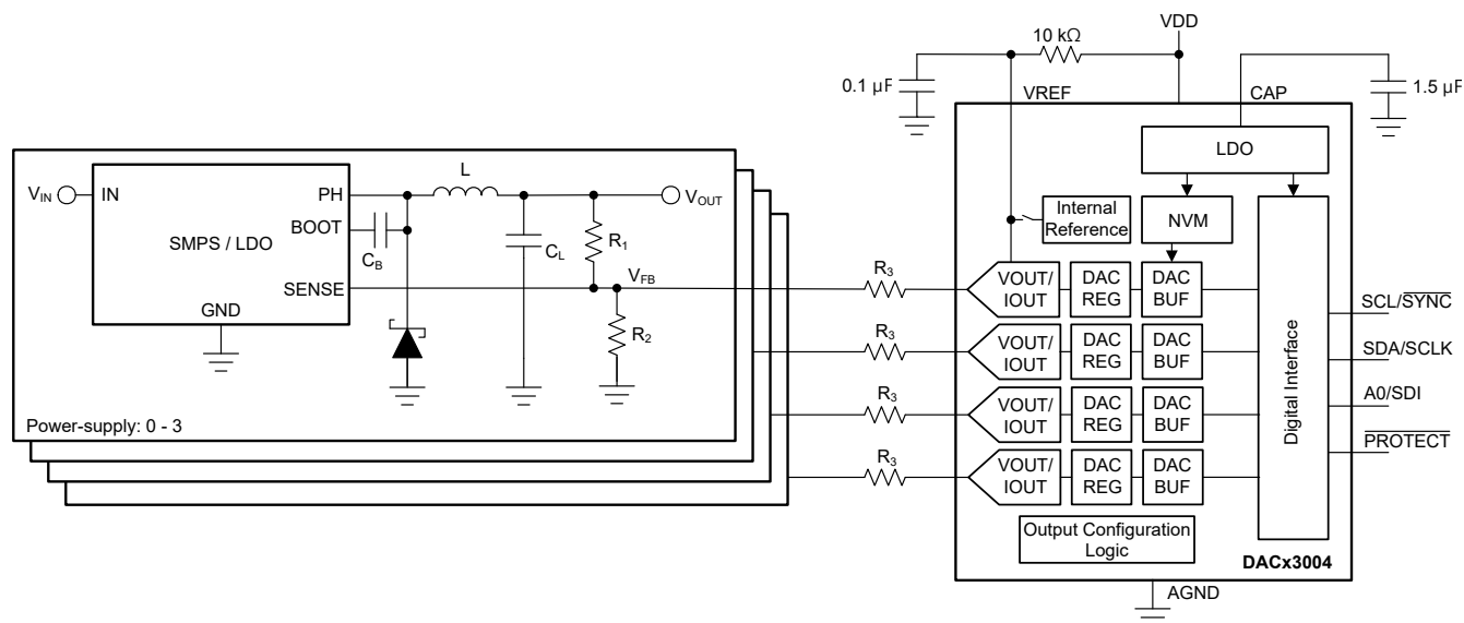
8-1. Voltage Margining and Scaling
