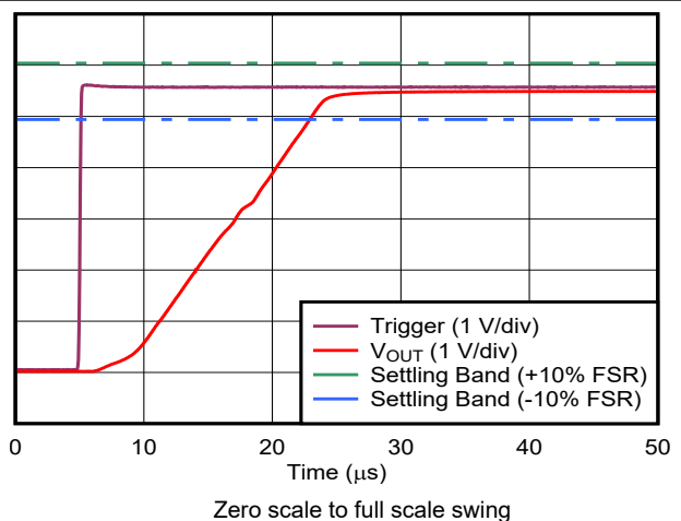
FIG 6-21. Voltage Output Settling Time - Rising Edge
