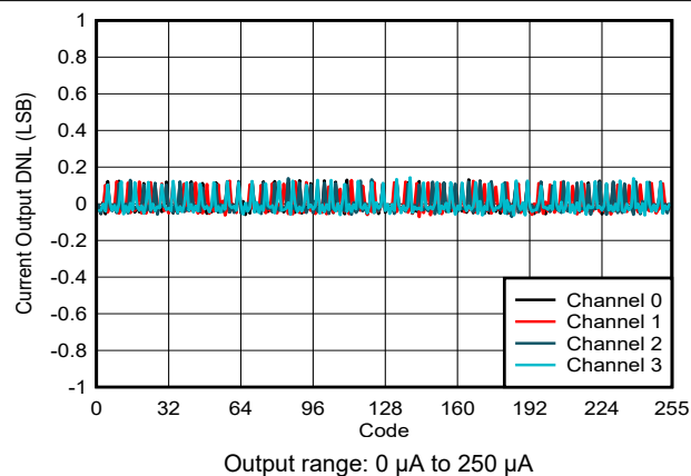
FIG 6-37. Current Output DNL vs Digital Input Code
