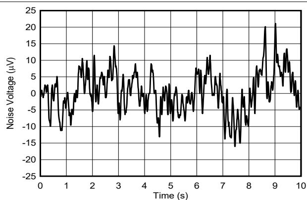
FIG 6-29. Voltage Output Flicker Noise
