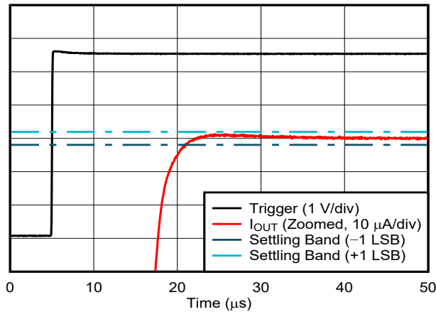
FIG 6-49. Current Output Setting Time, Rising Edge
