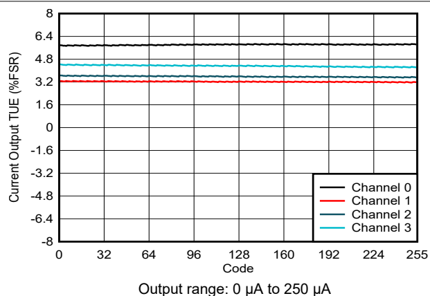
FIG 6-42. Current Output TUE vs Digital Input Code
