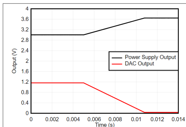
FIG 8-2. Power-Supply Margin High
