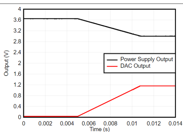
FIG 8-3. Power-Supply Margin Low
