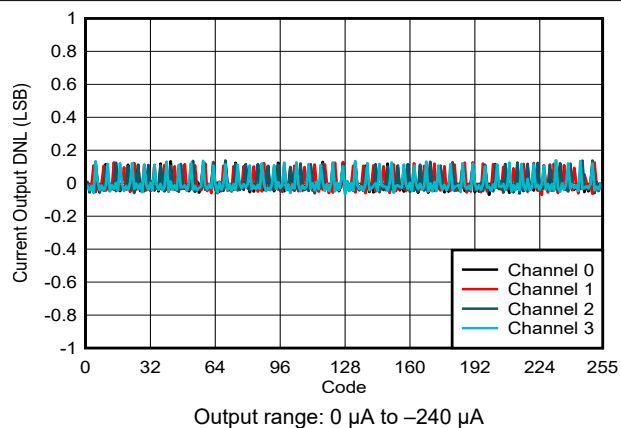
FIG 6-38. Current Output DNL vs Digital Input Code
