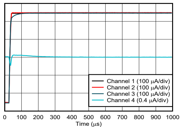
FIG 6-51. Current Output Power-On Glitch
