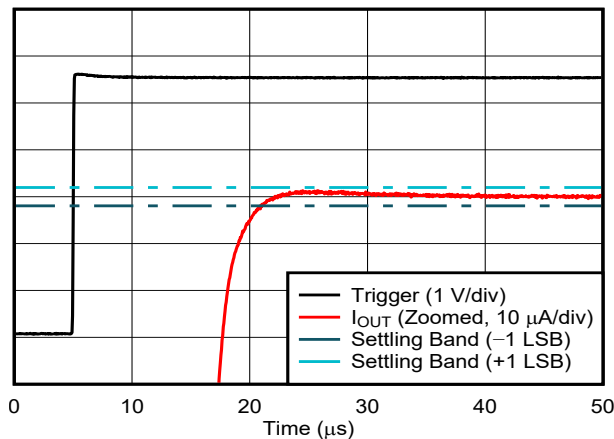
FIG 6-43. Current Output Setting Time, Rising Edge
