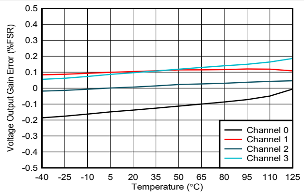
FIG 6-17. Voltage Output Gain Error vs Temperature
