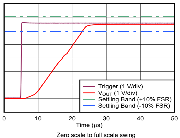
FIG 6-21. Voltage Output Setting Time - Rising Edge
