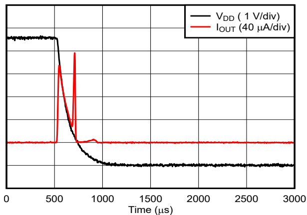
FIG 6-44. Current Output Setting Time, Falling Edge
