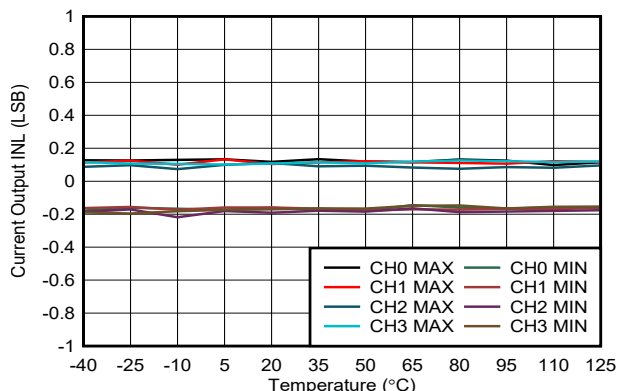
FIG 6-32. Current Output INL vs Temperature
