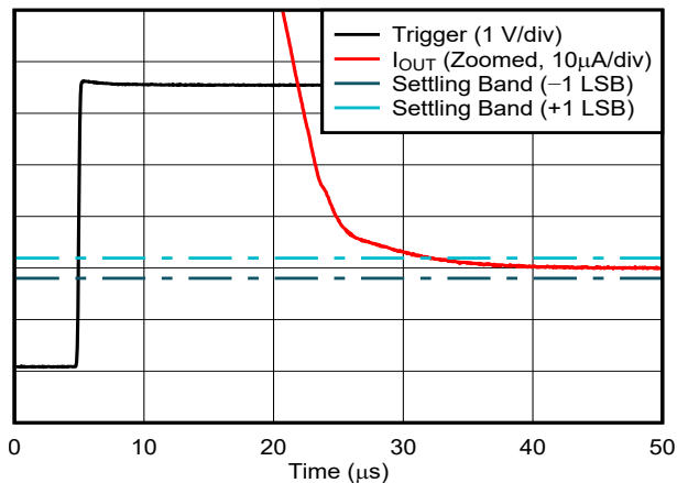
FIG 6-44. Current Output Setting Time, Falling Edge
