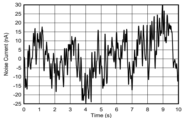
6-50. Current Output Flicker Noise
