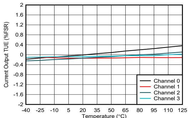
6-38. Current Output TUE vs Temperature
