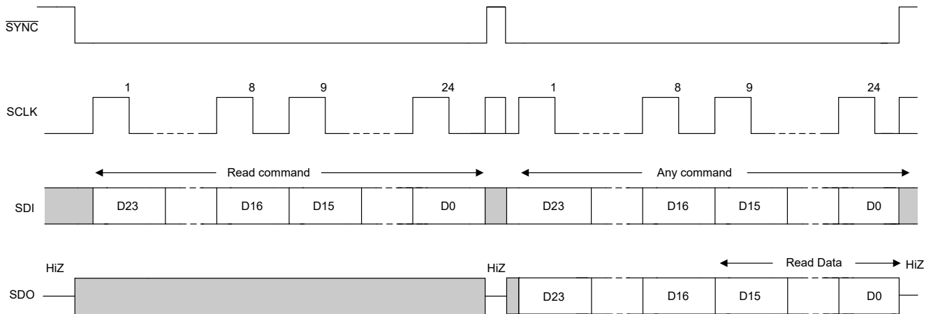
図 7-15. SPI Read Cycle
