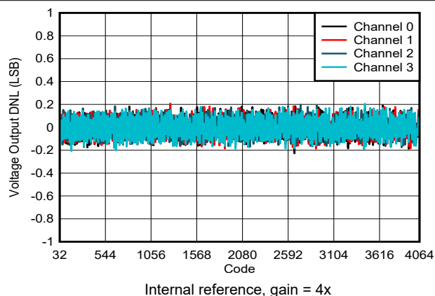
Figure 6-8. Voltage Output DNL vs Digital Input Code
