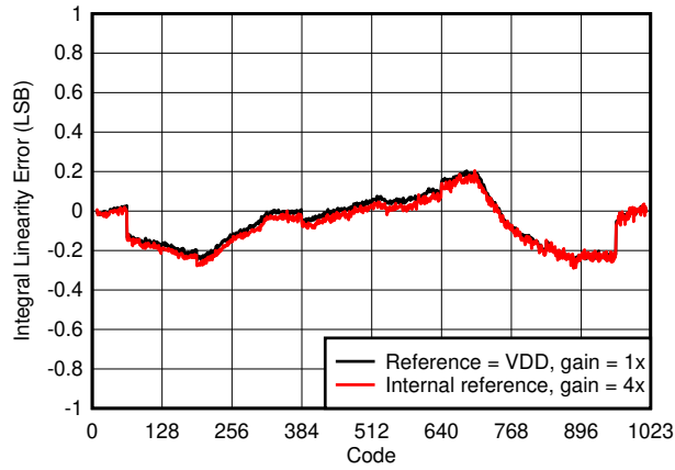
図 6-2. Integral Linearity Error vs Digital Input Code
