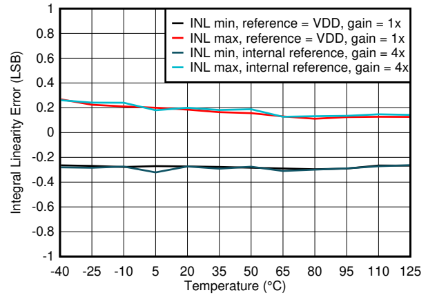
図 6-3. Integral Linearity Error vs Temperature
