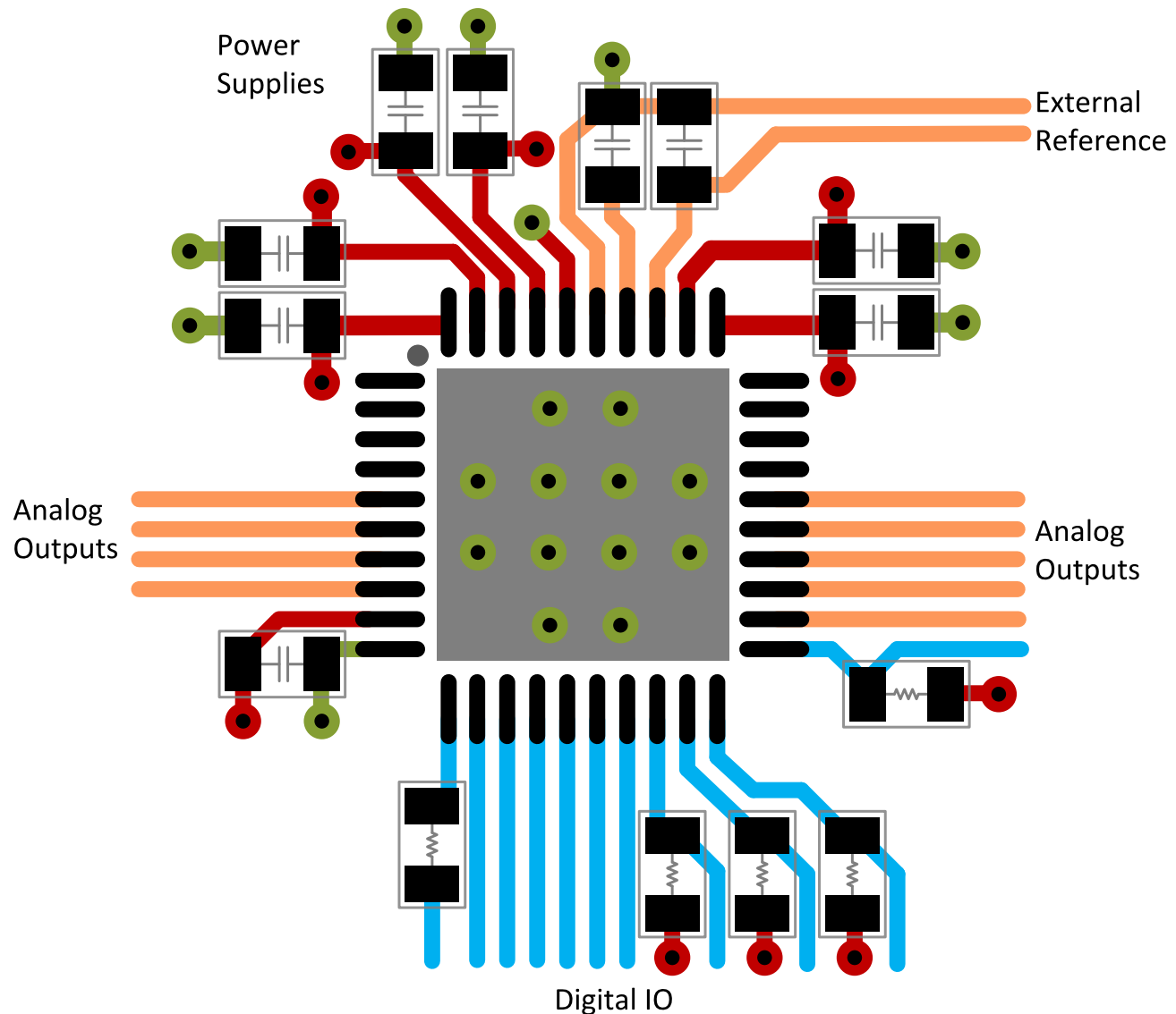
70. Example Layout
