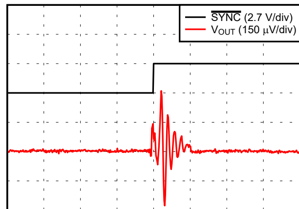
Time (50 ns/div) V_{DD} = 2.7\text{ V} , V_{REF} = 2.5\text{ V}
