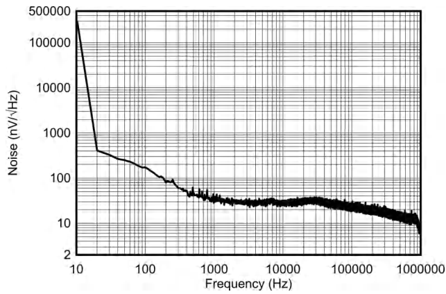
Figure 6-21. Output Noise Density vs Frequency
