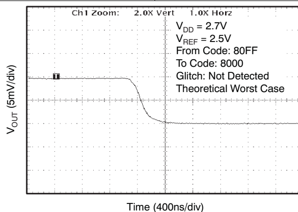
Figure 45. Glitch Energy: 2.7-V, 256-LSB Step, Falling Edge
