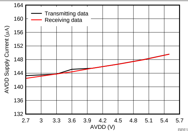
FIG 17. FF / PA Mode AVDD Supply Current versus Voltage with External Reference
