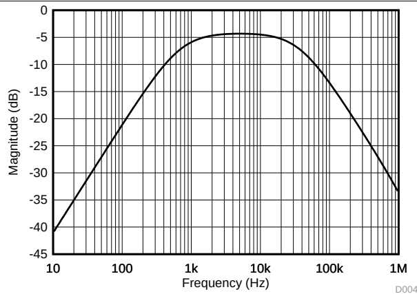
FIG 2. HART Mode External Band-Pass Filter Response
