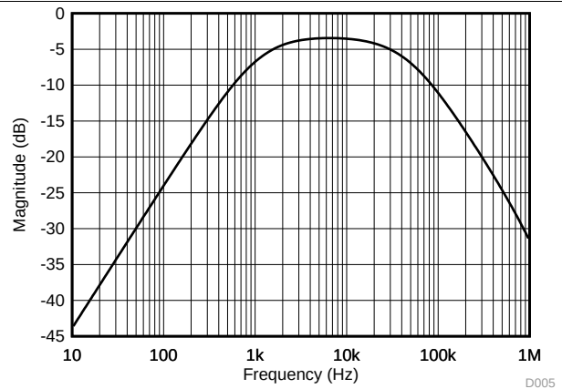
FIG 3. HART Mode Internal Band-Pass Filter Response
