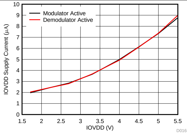
FIG 14. HART Mode IOVDD Supply Current versus Voltage with Internal Reference
