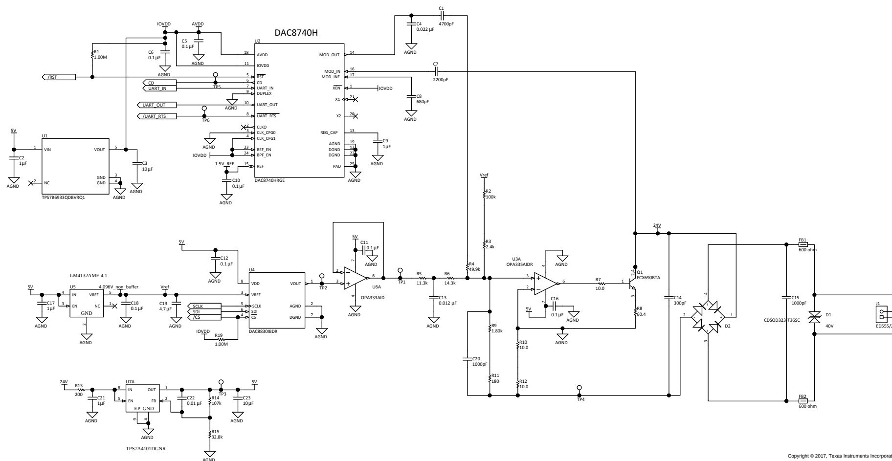
34. 2-Wire Transmitter with DAC8742H HART Modem Design Schematic
