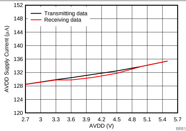
FIG 15. HART Mode AVDD Supply Current versus Voltage with Internal Reference
