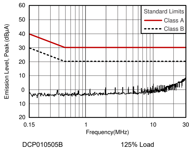
Figure 6-1. Conducted Emissions
