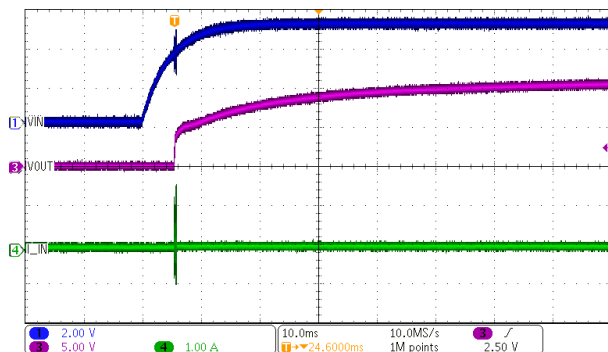
图 7-3. DCP010505BP Start-Up at No Load
