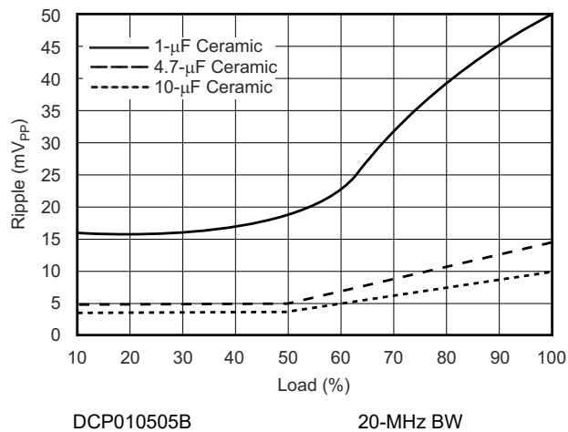
Figure 6-3. Output Ripple versus Load
