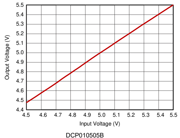
Figure 6-4. Line Regulation
