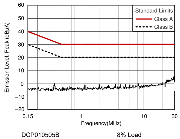
Figure 6-2. Conducted Emissions
