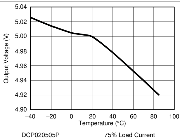
6-4. Output Voltage versus Temperature
