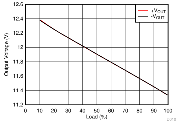
A. DCP021212DP Note: Operations under 10% Load
