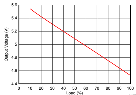
A. 6-6. Load Regulation Note: Operations under 10% Load
