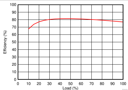
A. 6-5. Efficiency versus Load
