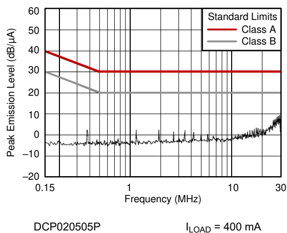
6-1. Conducted Emissions versus Frequency
