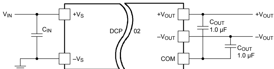
图 7-8. Dual Output Devices Connected in Series
