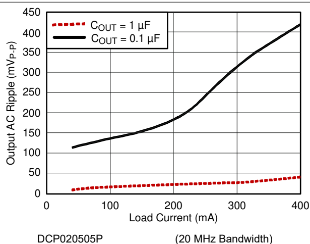
6-3. Output AC Ripple versus Load Current
