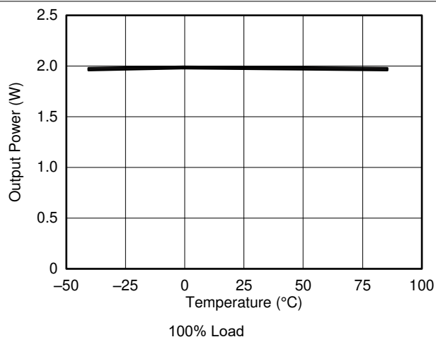
6-2. Output Power versus Temperature
