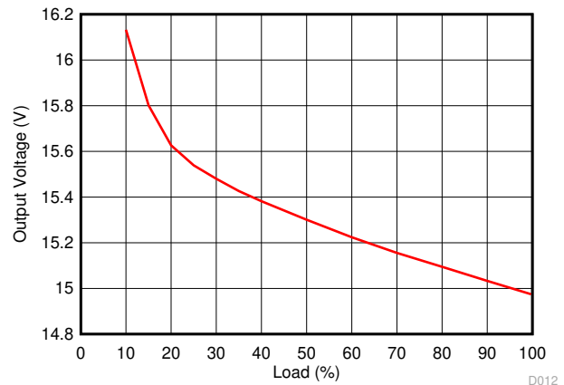
A. DCP021515P Note: Operations under 10% Load
