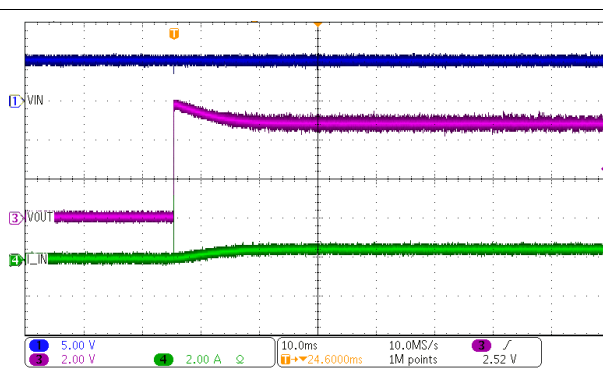
Figure 7-6. DCP020505P Enable Start-Up at 100% Load
