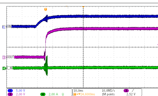
Figure 7-4. DCP020505P Start-Up at 10% Load
