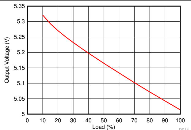
A. DCP022405P Note: Operations under 10% Load
