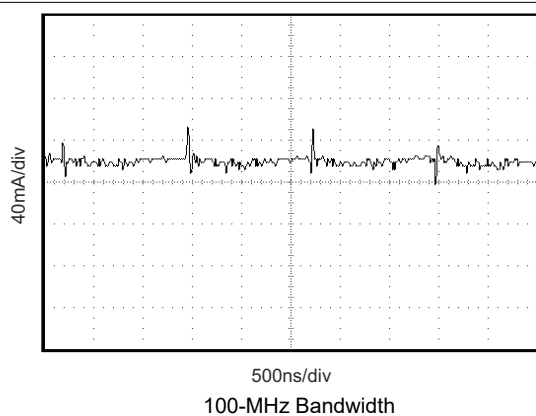
7-17. Input Current Reflected Ripple
