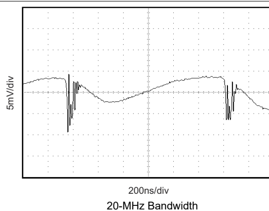
7-18. DCR010505P Output Voltage Ripple at 100% Load
