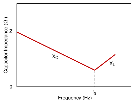
Figure 9-2. Capacitor Impedance versus Frequency
