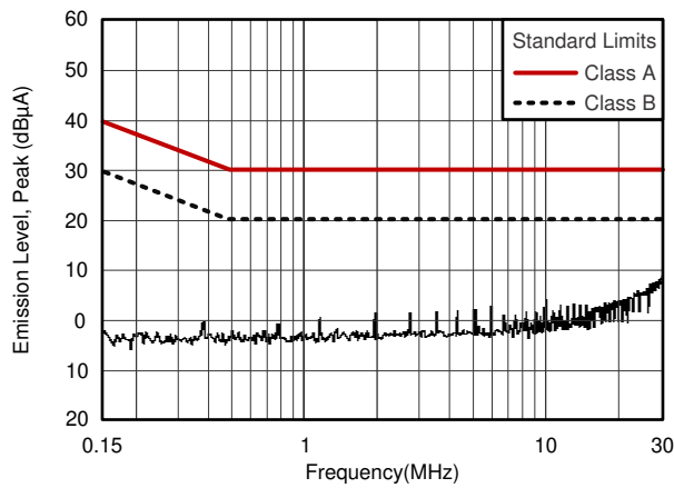
7-1. Conducted Emissions
