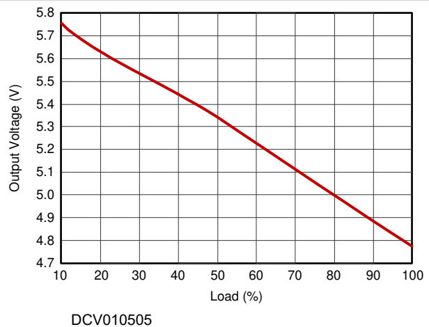
7-6. Load Regulation
