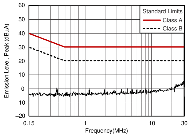
7-2. Conducted Emissions
