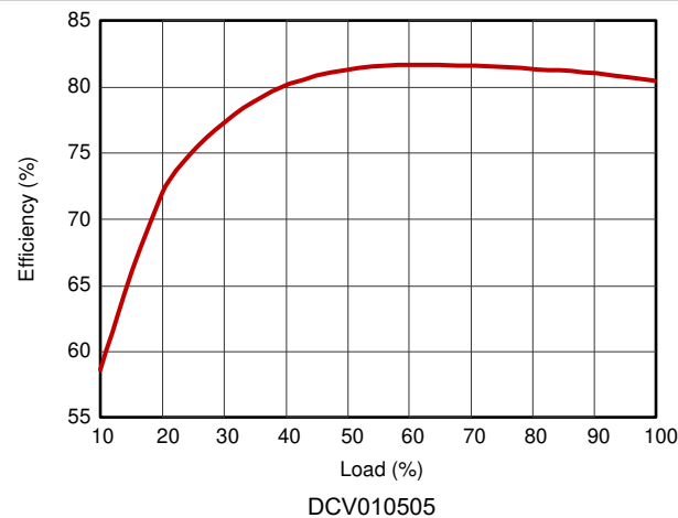
7-5. Efficiency versus Load
