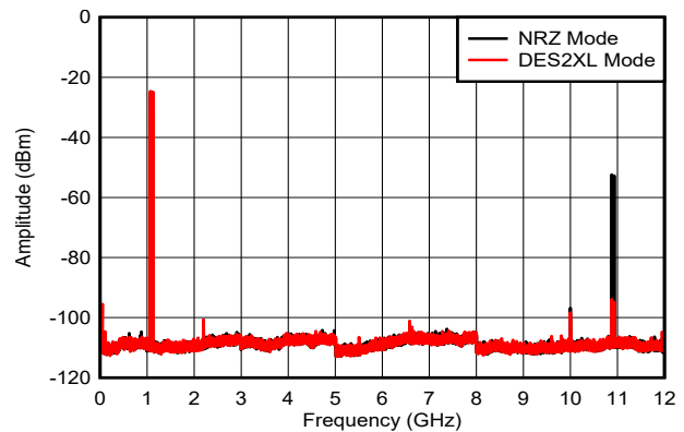
図 6-29. Dual Tone, f_{\text{OUT}} = 1097\text{MHz} , 0dBFS
