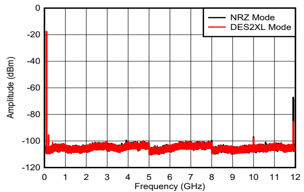
図 6-27. Dual Tone, f_{\text{OUT}} = 97\text{MHz} , -6dBFS
