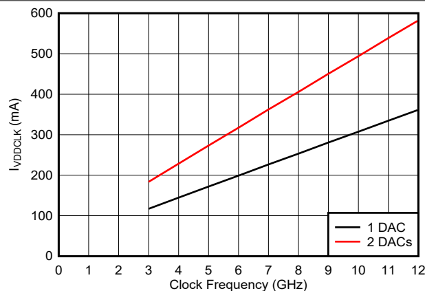
Independent of JMODE and Interpolation Figure 6-52. VDDCLK Current vs Clock Frequency
