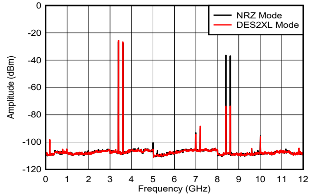
図 6-35. Dual Tone, f_{\text{OUT}} = 3497\text{MHz} , 0dBFS
