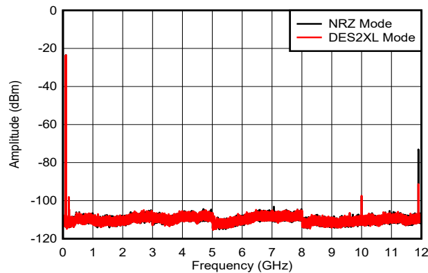
図 6-26. Dual Tone, f_{\text{OUT}} = 97\text{MHz} , 0dBFS
