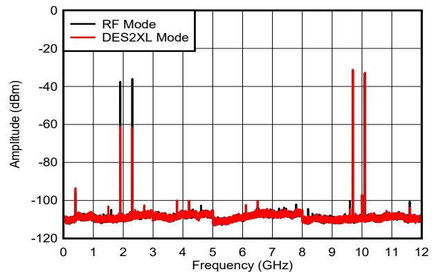
図 6-41. Dual Tone, f_{\text{OUT}} = 9897\text{MHz} , 0dBFS
