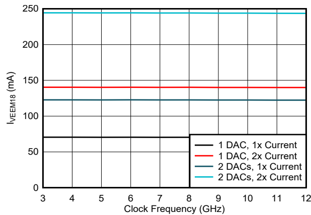
Independent of JMODE and Interpolation Figure 6-50. VEEM18 Current vs Clock Frequency and Output Current
