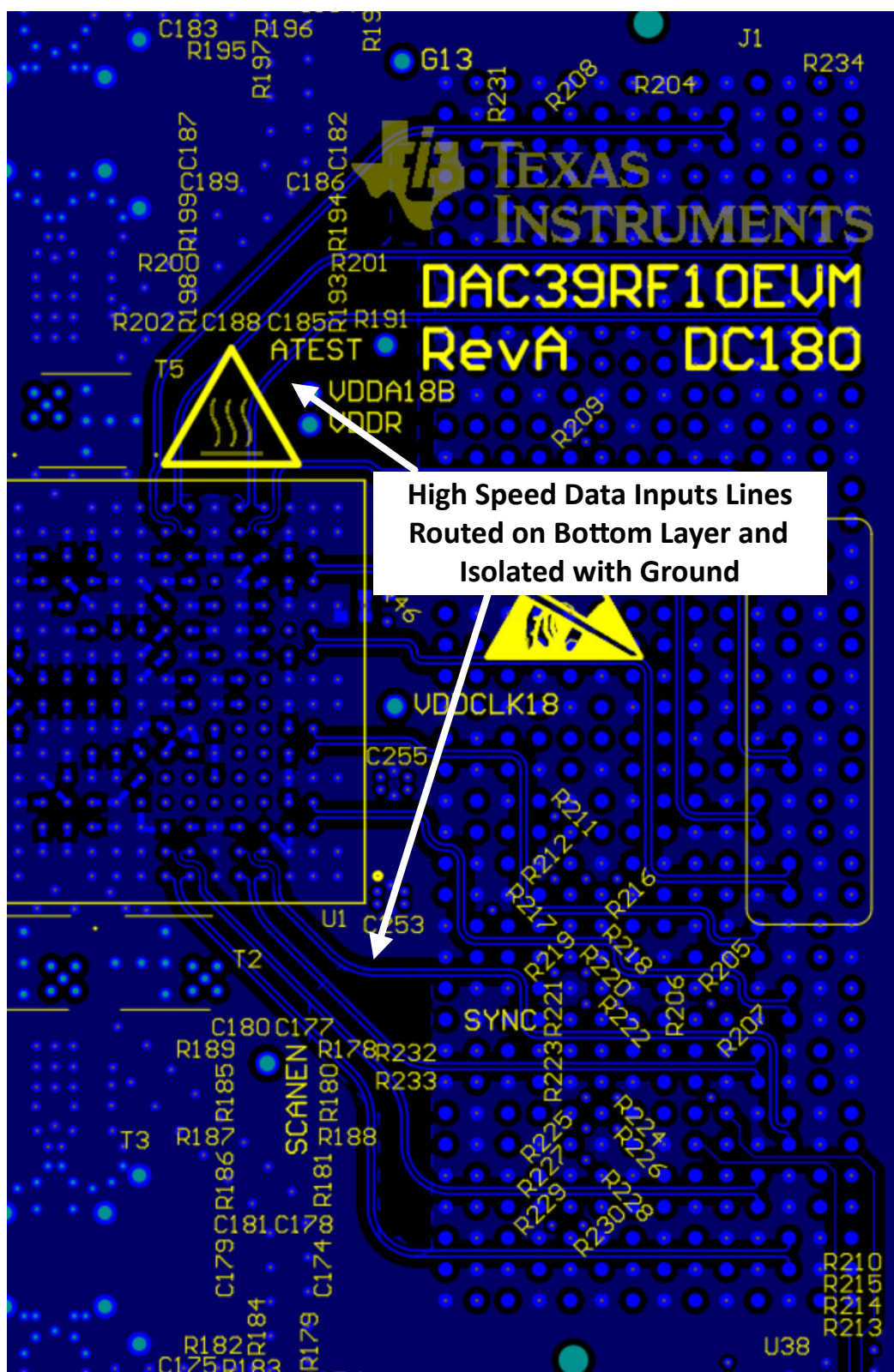
8-29. Serdes Bottom Layer Routing with Ground Isolation
