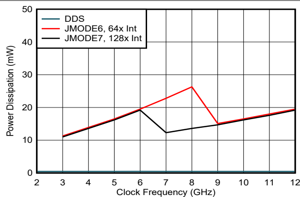
Dependent on # of Serdes and baud rate Figure 6-54. VDDR18 Current vs Clock Frequency and Interface Mode
