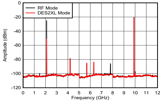
図 6-22. f_{\text{OUT}} = 8097\text{MHz} , -12dBFS
