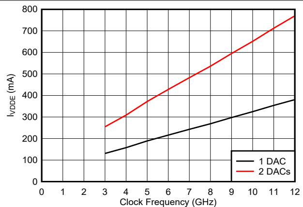
Independent of JMODE and Interpolation Figure 6-53. VDDE Current vs Clock Frequency
