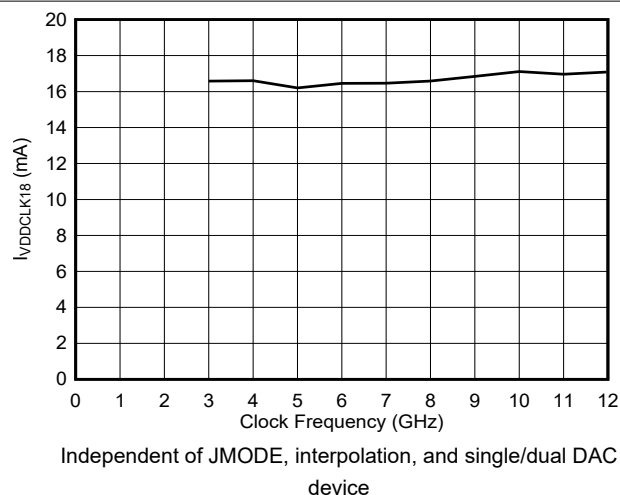
Figure 6-49. VDDCLK18 Current vs Clock Frequency
