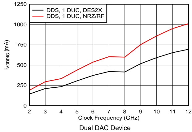
FIG 6-58. VDDDIG Current vs Clock Frequency and DAC Mode
