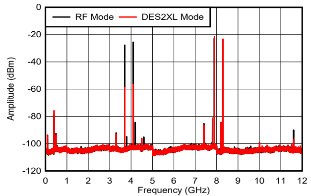
図 6-39. Dual Tone, f_{\text{OUT}} = 8097\text{MHz} , -6dBFS
