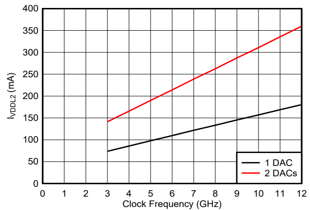
Independent of JMODE and Interpolation Figure 6-51. VDDLx Current vs Clock Frequency
