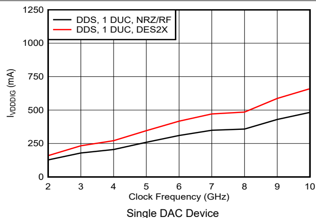
6-59. VDDDIG Current vs Clock Frequency and DAC Mode
