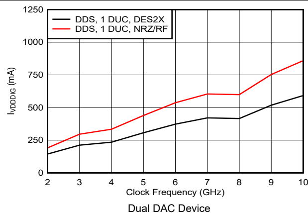
6-58. VDDDIG Current vs Clock Frequency and DAC Mode
