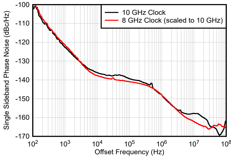
図 8-12. 8GHz and 10GHz Clock Phase Noise
